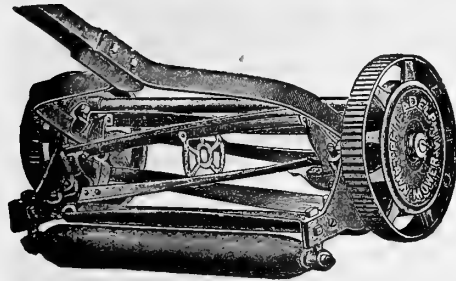
Philadelphia Lawn Mower. Style K.
