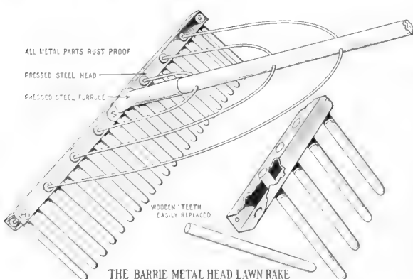
THE BARRIE METAL HEAD LAWN RAKE
