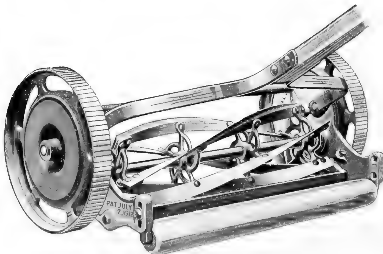
Farquhar's Automatic Lawn Mower.
