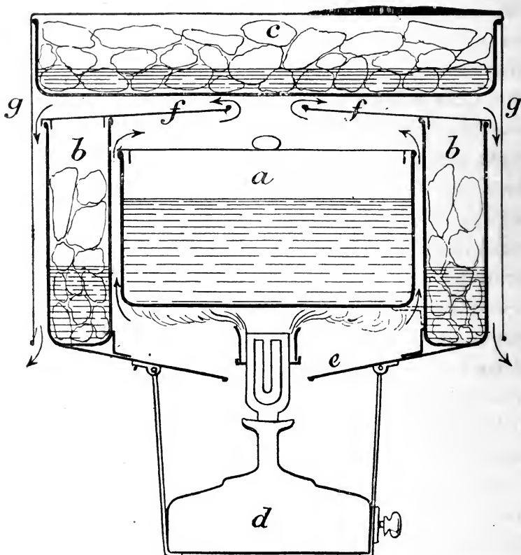
THE COOKING APPARATUS.
