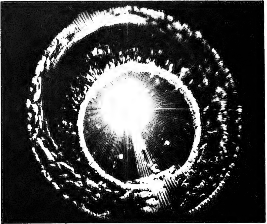
Figure 17. AGS display showing 10-foot diameter wooden water tank at a depth of 10 feet. (From Reference 20.)
