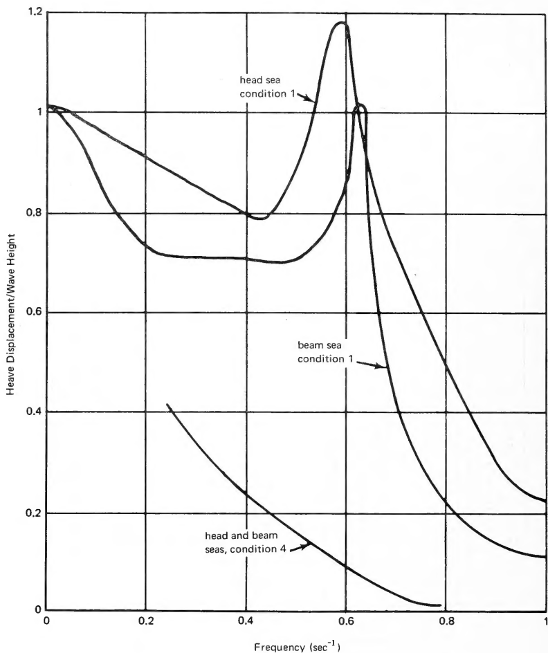
Figure B-16. Heave response of FORDS in regular waves of small amplitude.
