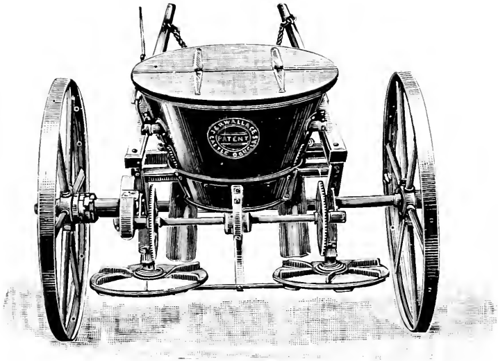
FIG. 9.—BROADCAST MANURE SOWER WITH REVOLVING DISCS FOR DISTRIBUTION.
