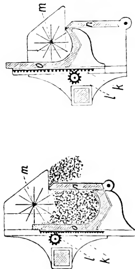
FIG. 6.—DIAGRAMMATIC SECTION OF MANURE DISTRIBUTOR—SEED DRILL TYPE.
