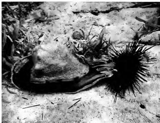
Figure 3. Helmet changes attack mode. Note trail of urchin spines and angle of urchin such that most tube feet are not in contact with the substrate.
