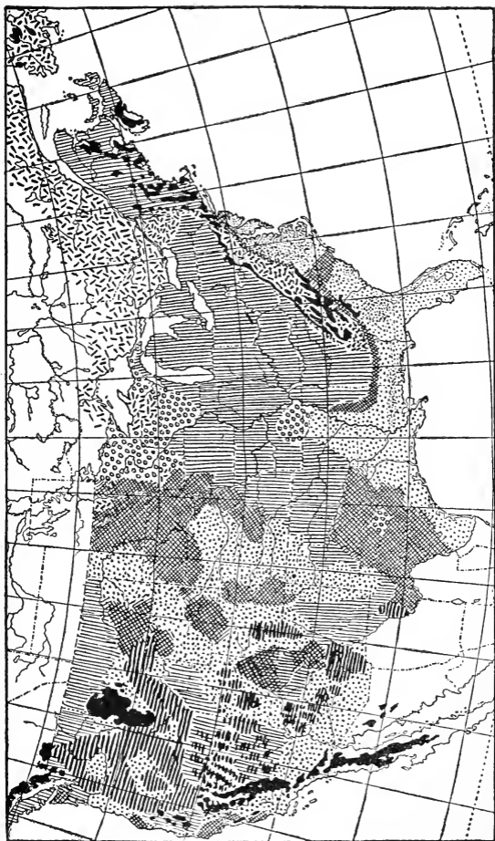
GEOLOGICAL STRUCTURE
