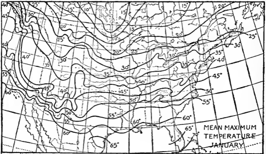
ISOTHERMAL LINES FOR JANUARY
