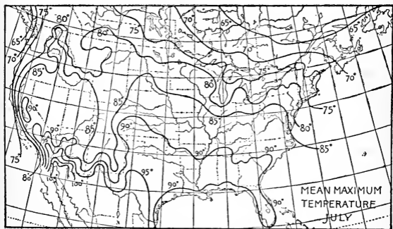
ISOTHERMAL LINES FOR JULY
