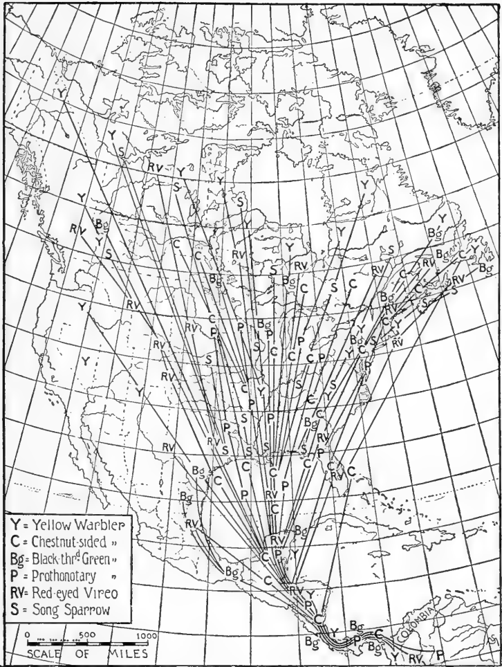
MIGRATORY ROUTES OF THE BLACK-THROATED GREEN, CHESTNUT-SIDED, YELLOW, AND PROTHONOTARY WARBLERS, RED-EYED VIREO AND SONG SPARROW. Only the four species, Bg, C, S & P, halt short of the limits of Colombia. The eighteen other species (see maps) fly on, many hundreds of miles beyond.
