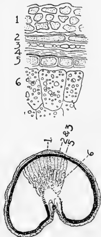
FIG. 53. — Cross-section and transverse section of grain of wheat. Below: transverse section of an unripe grain. (1) Ovary wall or pericarp; (2) outer integument; (3) inner integument; (4) remains of nucellus; (5) aleurone cells; (6) starch cells.
