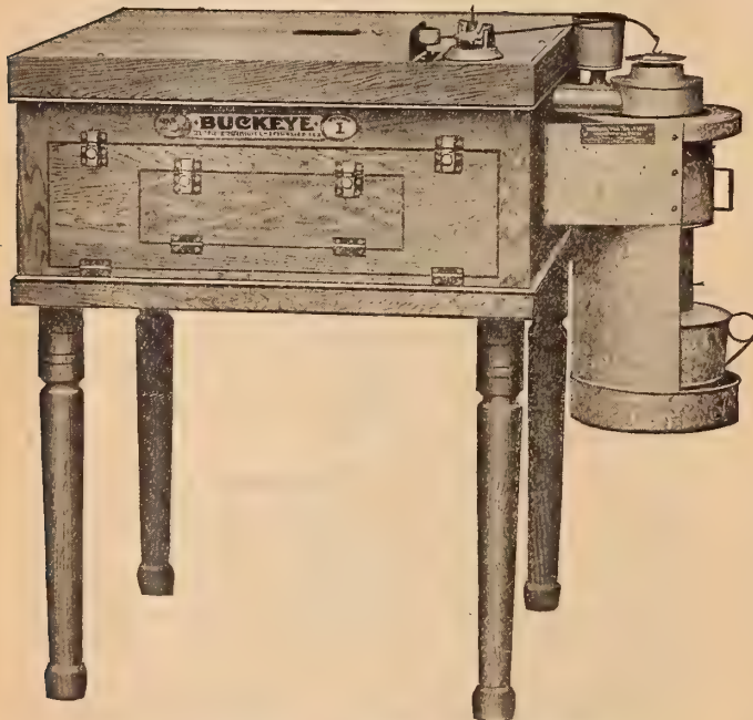
Buckeye No. 1, Standard 110-Egg Incubator
