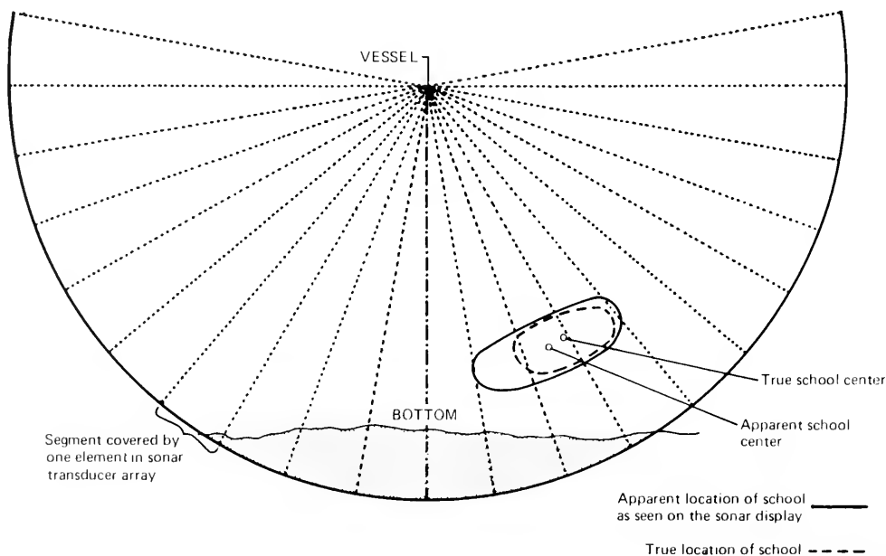
FIGURE 12.—A facsimile of the sector scanning sonar output display exemplifying biases in apparent school locations resulting from the limited resolution of the instrument.
