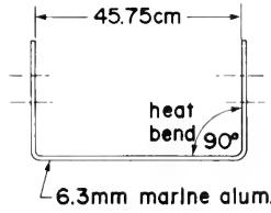
DEPRESSOR-FRONT ELEVATION
