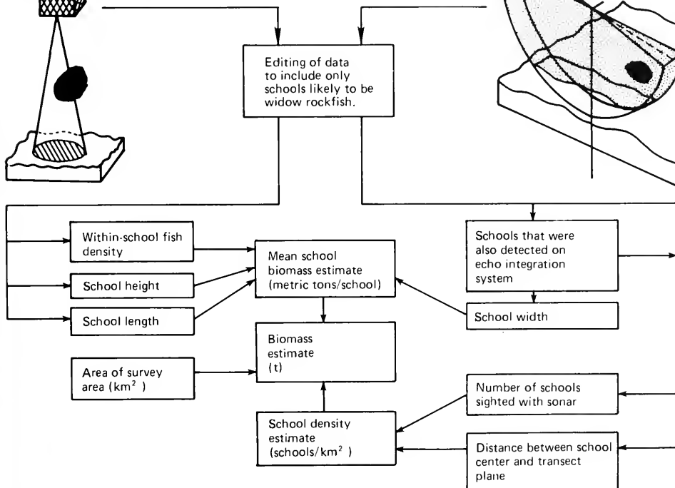
FIGURE 9.—Schematic diagram depicting the analysis of echo sounder and sonar data collected during hydroacoustic line transect surveys.
