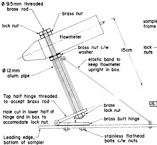
FLOWMETER ATTACHMENT DETAIL
