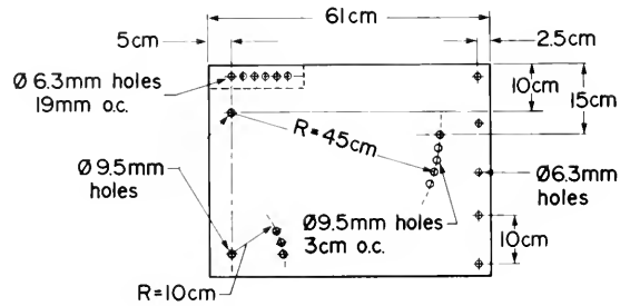
FIGURE 2.—Scale drawings of the sampler body and float, and net attachment detail.
