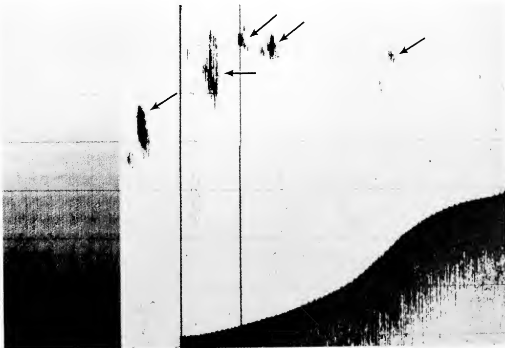
FIGURE 6.—Echogram showing the configuration of "evening and morning" widow rockfish schools (arrows).
