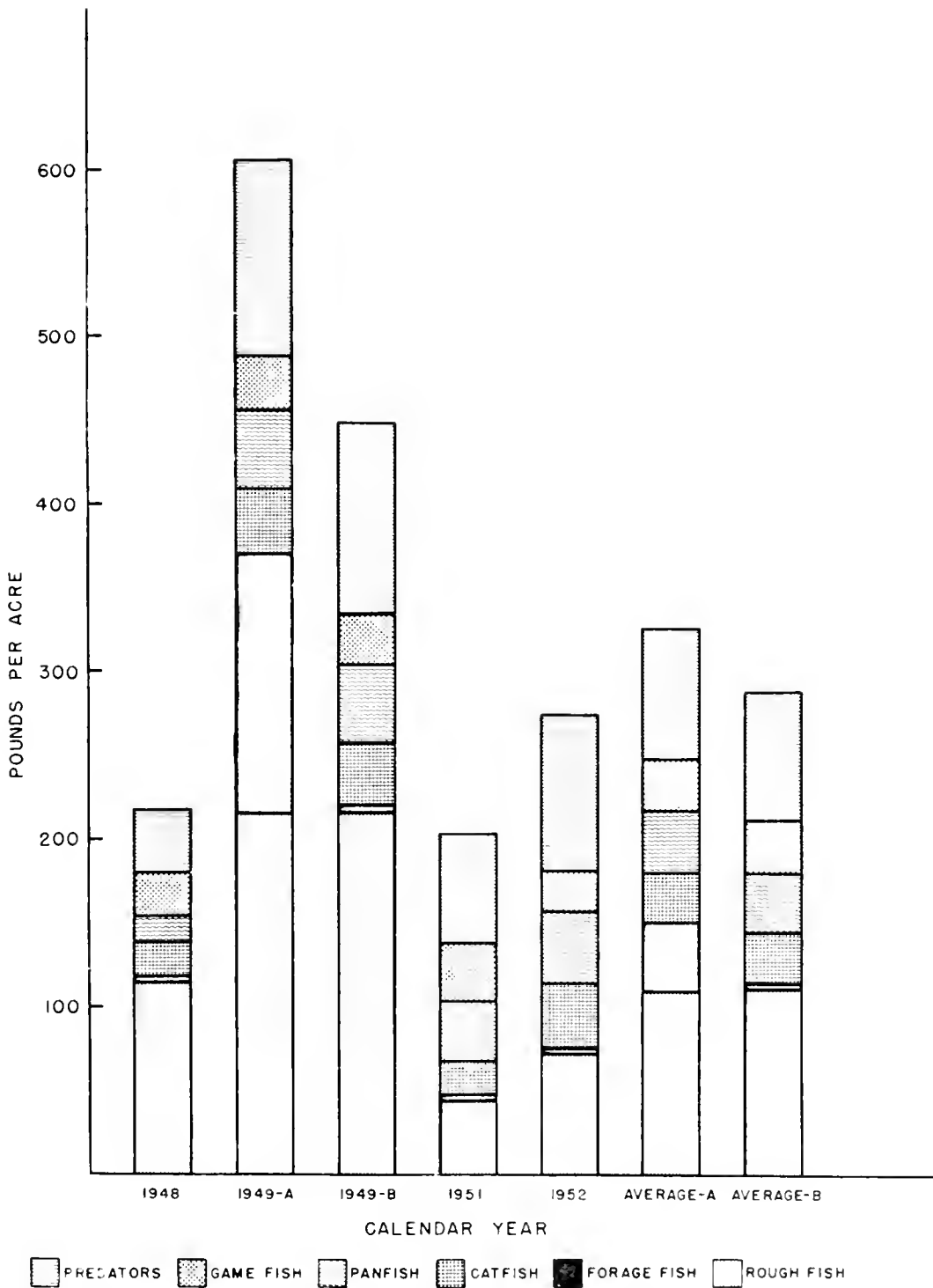
Figure 5:--Standing crops of fish in area P in 1948, 1949, 1951, and 1952 expressed as pounds per acre of the various species groups. The 1949-A and Average-A columns include adult gizzard shad collected in 1949. The 1949-B and Average-B columns represent the adjusted standing crops when adult gizzard shad are excluded.
