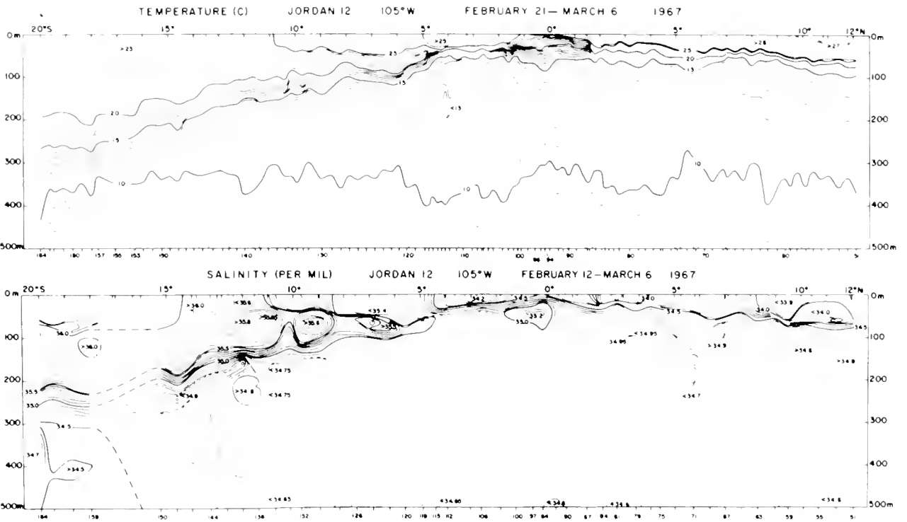
Hand drawn vertical sections of temperature and salinity for leg 3 of David Starr Jordan's EASTROPAC 12 cruise, including STD and XBT data.
