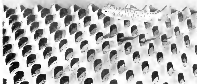
FIGURE 44.—Expanded metal plate attached to surface of horizontal conduit (in turbine intake model). The configurations of the plate change water flow and may enable fish to swim away from a turbine intake.
