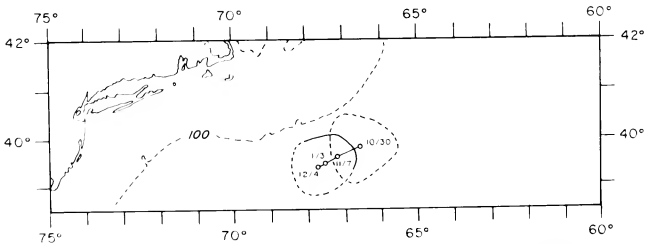
Figure 15.7.—Track line for anticyclonic eddy 76G (27 October 1976-13 May 1977). Surface boundaries, as seen on satellite imagery, are shown for some positions.
