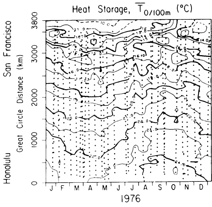
Figure 7.4.—Heat storage for the surface to 100-m layer, expressed as average temperature ( \bar{T} ) 0-100 m in degrees Celsius (C), between San Francisco and Honolulu during 1976. Symbols (+) indicate the locations of the expendable bathythermograph observations. Contour interval is 1.0C.
