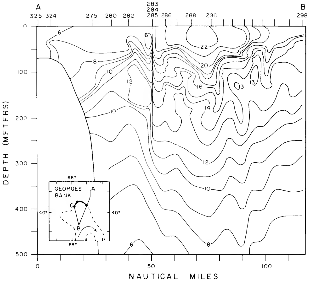
Figure 15.9.--Expendable bathythermograph (XBT) section (degrees C) from RV Albatross IV in Gulf Stream meander (or eddy) on 2-3 April 1976 that had been pushed into proximity with Georges Bank. Section is not given for line B to C on inset map. The three dots on the map inset correspond to the locations where the thermal front was defined by the XBT survey. See text for discussion.
