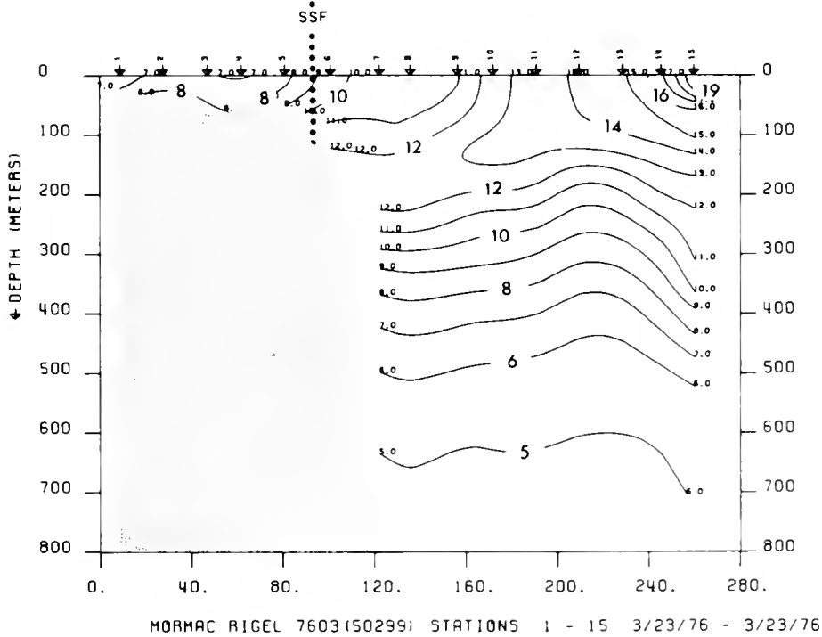
Figure 14.7.—Horizontal distribution of sea surface temperature (degrees C) and sea surface salinity (‰) and vertical distribution of temperature (degrees C) in the upper 200 and 800 m; Mormac Rigel 76-03, 23 March 1976.
