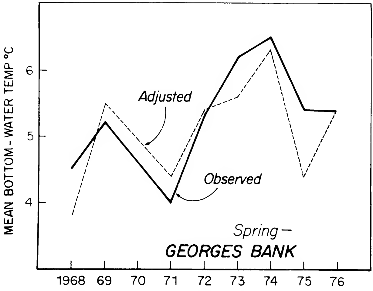
Figure 22.5.—Observed and adjusted mean bottom-water temperatures on Georges Bank during spring 1968-76.
