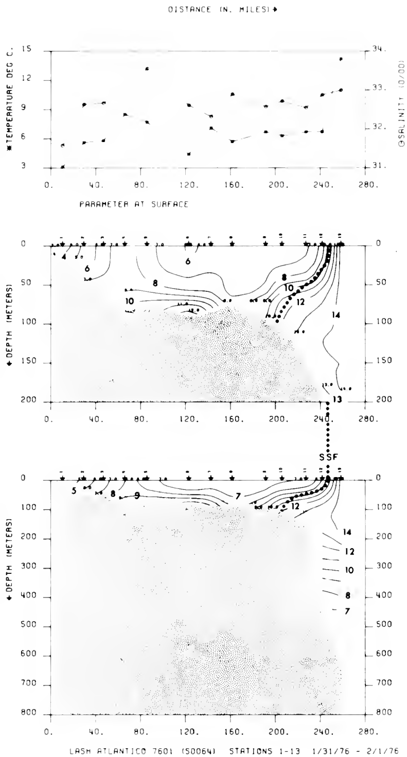
Figure 14.3.—Horizontal distribution of sea surface temperature (degrees C) and sea surface salinity (‰) and vertical distribution of temperature (degrees C) in the upper 200 and 800 m; Lash Atlantic 76-01, 31 January-1 February 1976.
