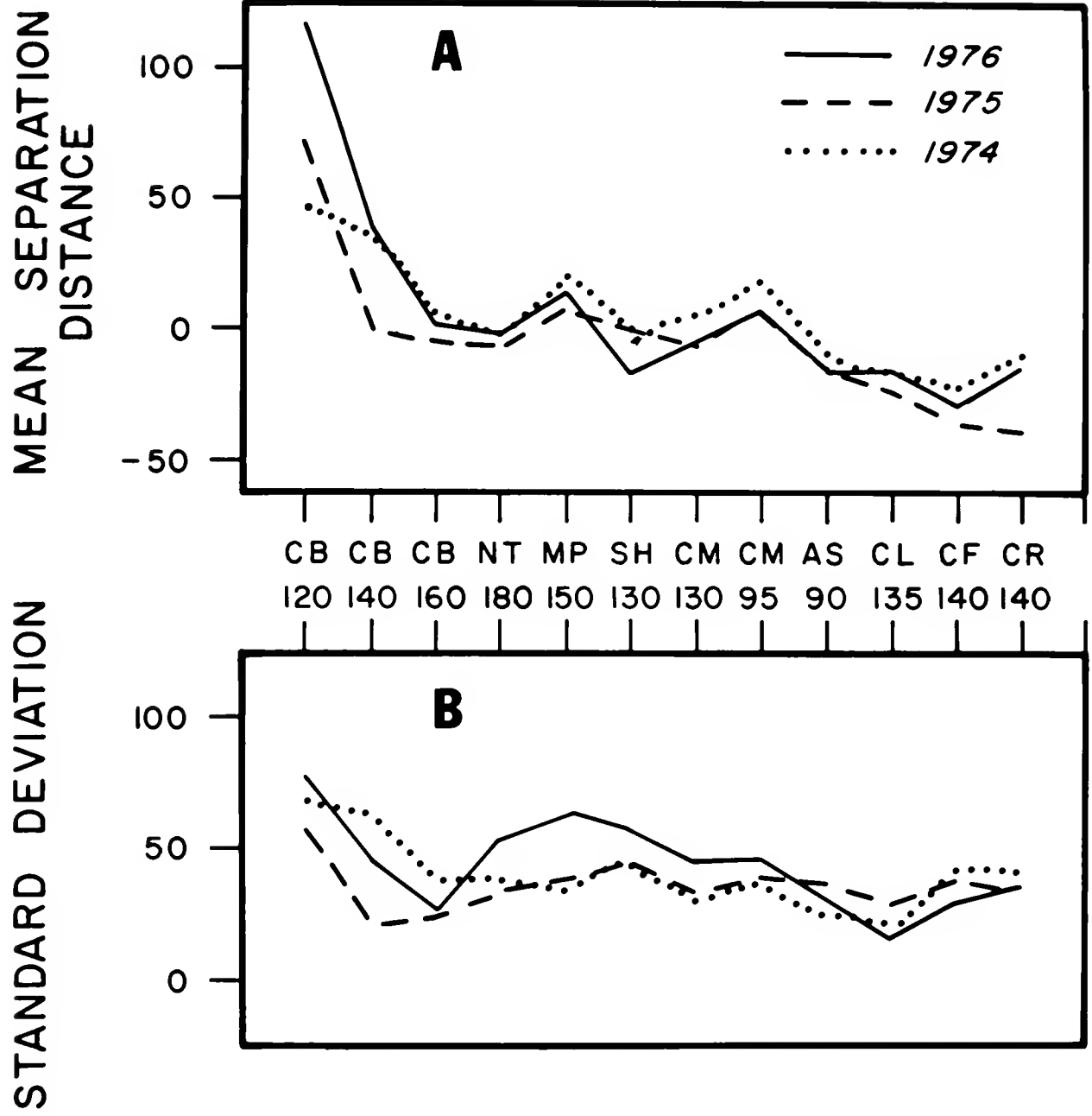
Figure 18.7.—Annual mean Shelf Water front positions relative to 200-m isobath (positive is seaward) and standard deviation of position at each standard bearing line, 1974-76.
