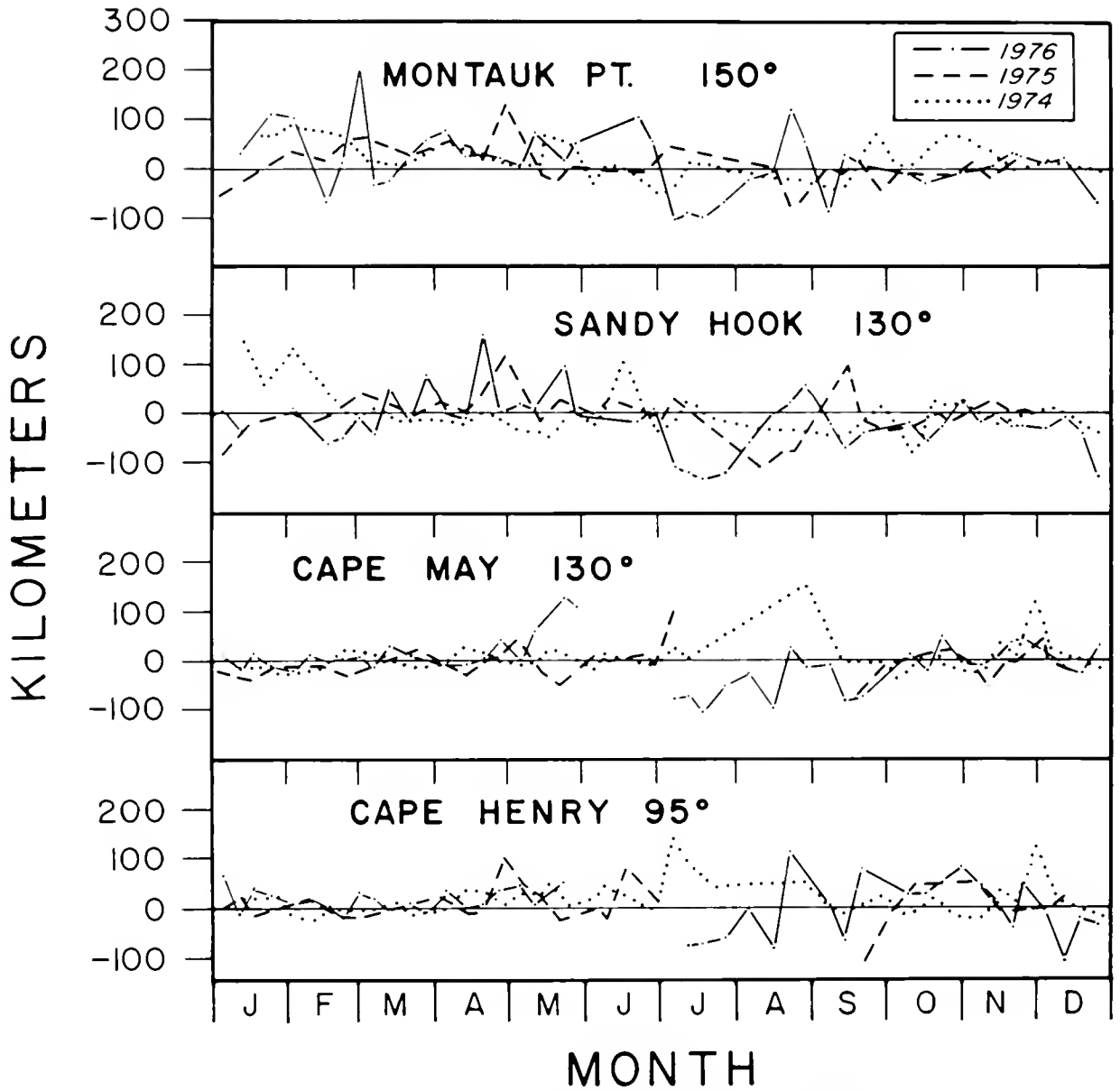
Figure 18.1.—Annual march of Shelf Water front positions relative to the 200-m isobath (positive is seaward), 1974-76, along standard bearing lines off the Middle Atlantic region.
