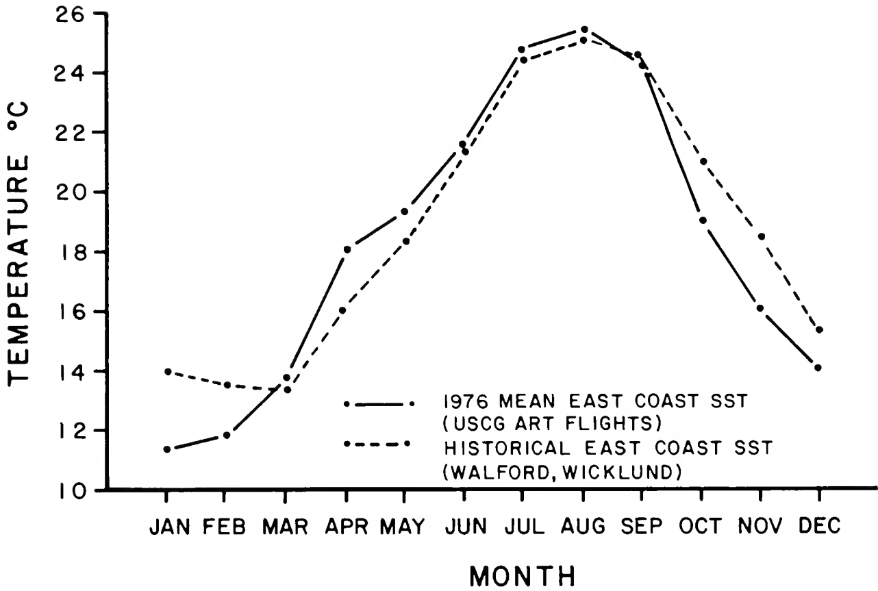
Figure 13.3.—East coast average monthly mean sea surface temperature (SST) (degrees C) for 1976 and the historical average.
