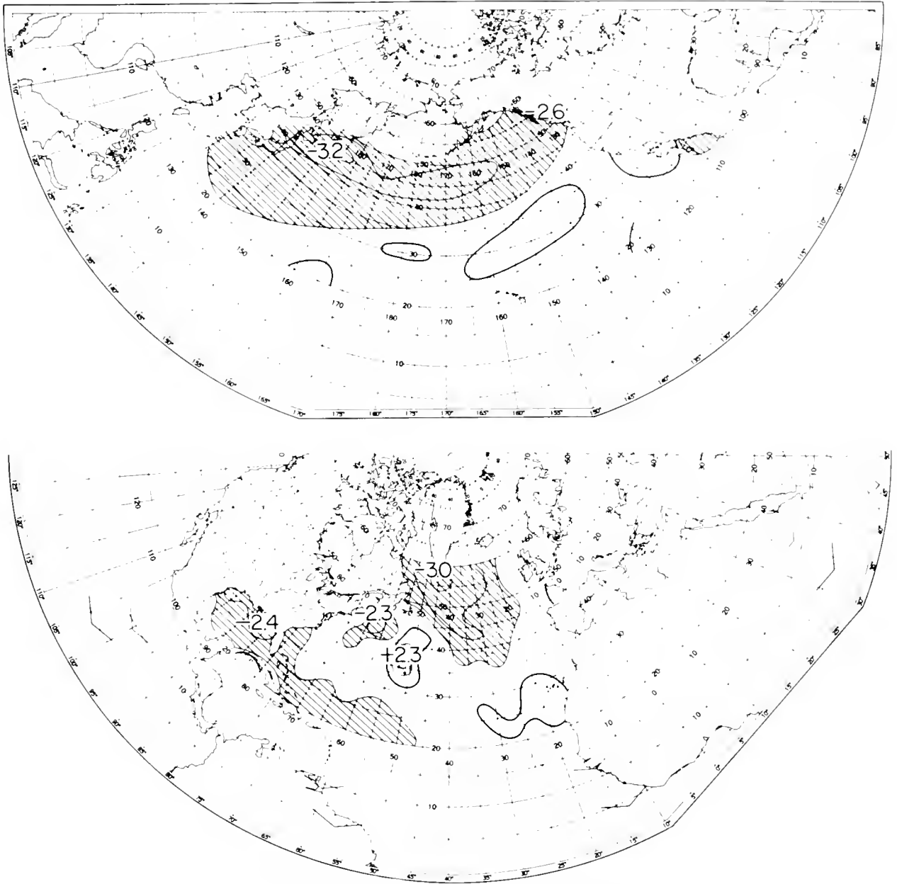
Figure 2.6—Mean annual anomaly from the long-term, 1948-67, mean of sea surface temperature in degrees F for the North Pacific Ocean (upper) and the North Atlantic Ocean (lower). Anomalies >+1^{\circ}\text{F} are stippled, >-1^{\circ}\text{F} are hatched.
