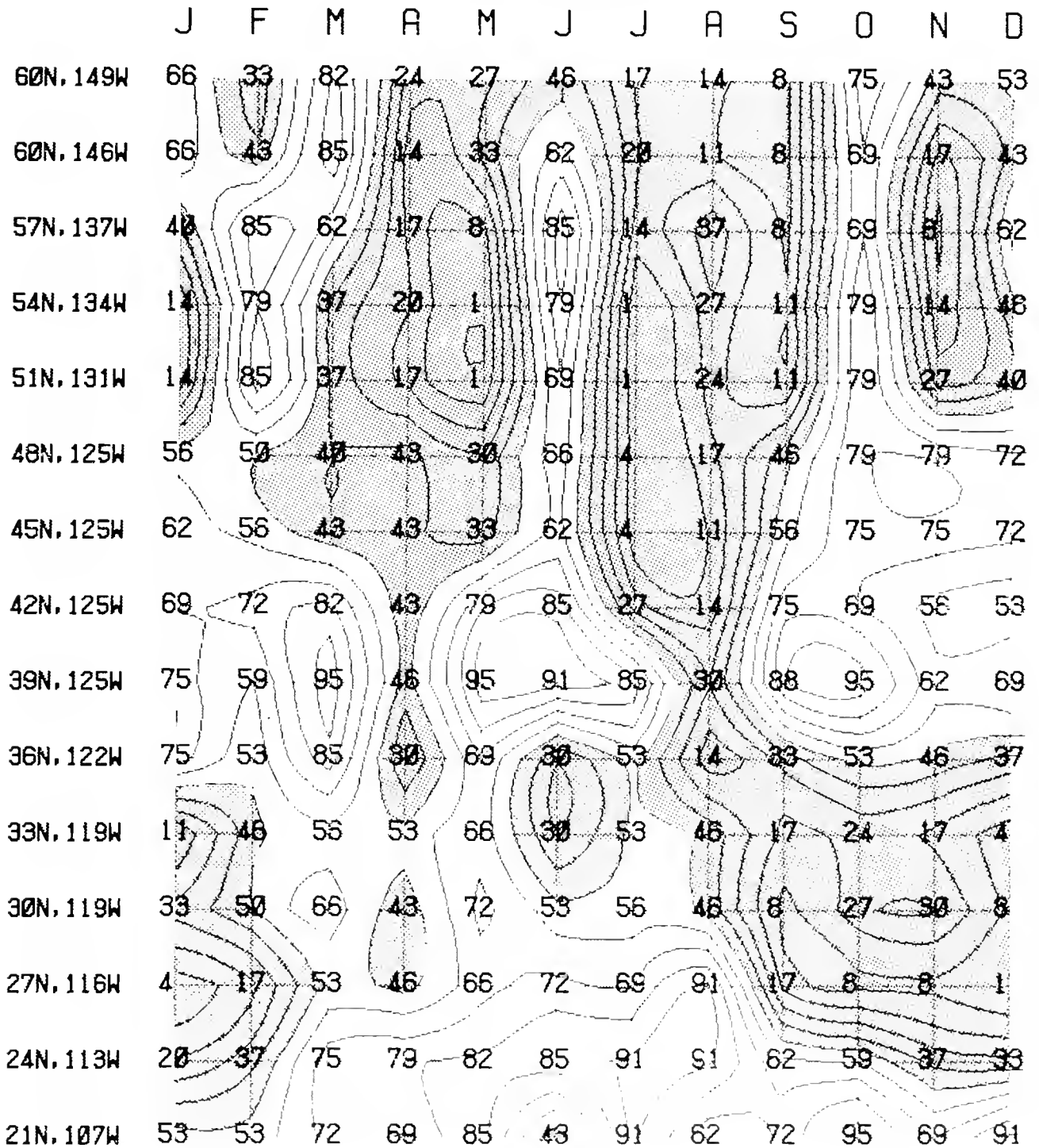
Figure 6.2.—Percentalized upwelling index values for 1976. Percentiles indicate relative ranking within the 31-yr data set for each month and location. The contour interval is 10 percentile units. Values below the median (50th percentile) are shaded.
