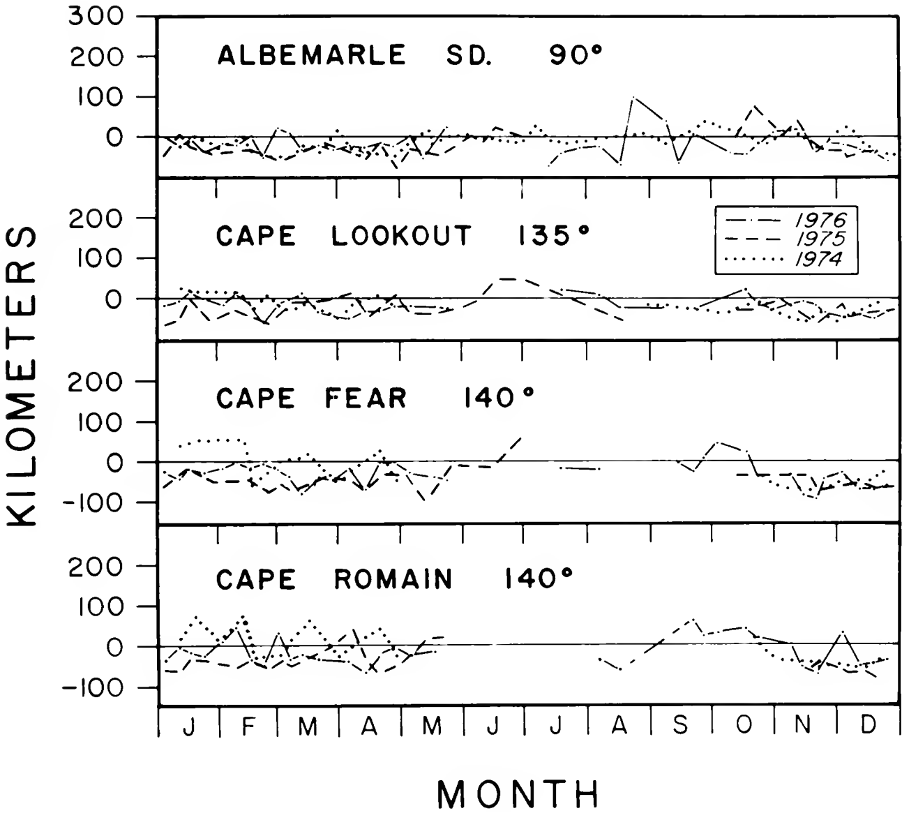
Figure 18.5.—Annual march of Shelf Water front positions relative to the 200-m isobath (positive is seaward), 1974-76, along standard bearing lines off the Middle Atlantic and southern regions.
