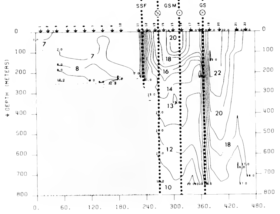
Figure 14.8.—Horizontal distribution of sea surface temperature (degrees C) and sea surface salinity (‰) and vertical distribution of temperature (degrees C) in the upper 200 and 800 m; Export Defender 76-01 , 3-4 April 1976.
