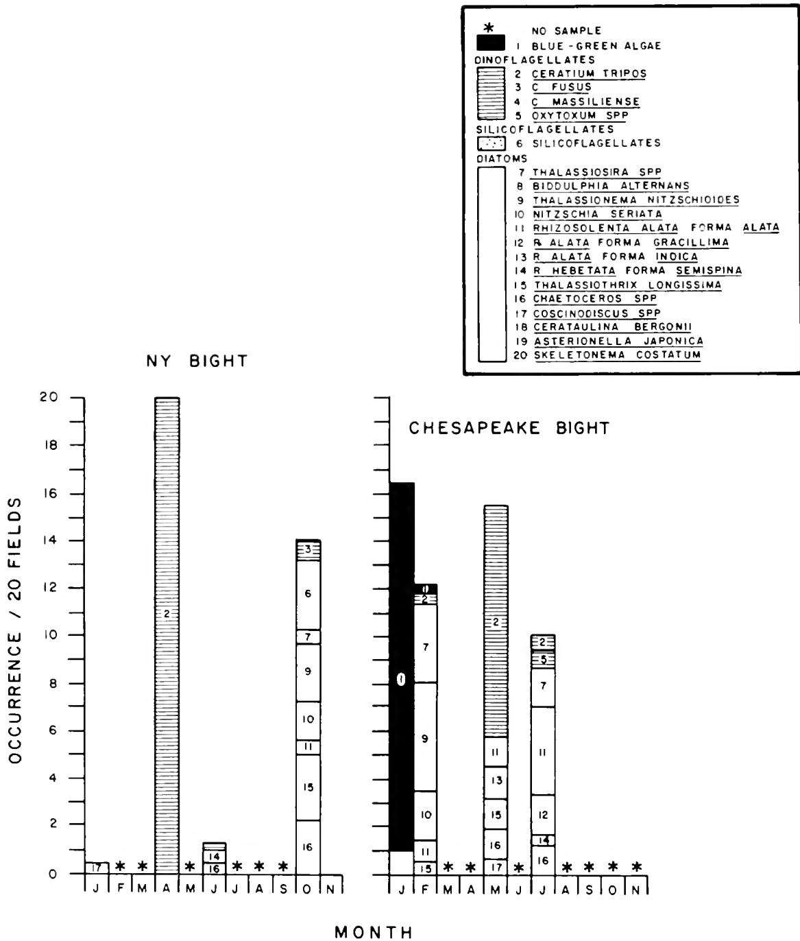
Figure 20.2.—Net phytoplankton abundance in Slope Water to the seaward of the New York and Chesapeake Bights, 1976. See text for explanation of abundance units.
