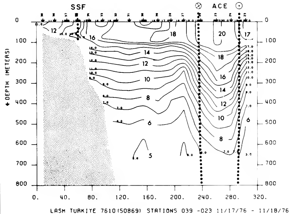
Figure 14.17.—Horizontal distribution of sea surface temperature (degrees C) and sea surface salinity (‰) and vertical distribution of temperature (degrees C) in the upper 200 and 800 m; Lash Turkiye 76-10, 17-18 November 1976.
