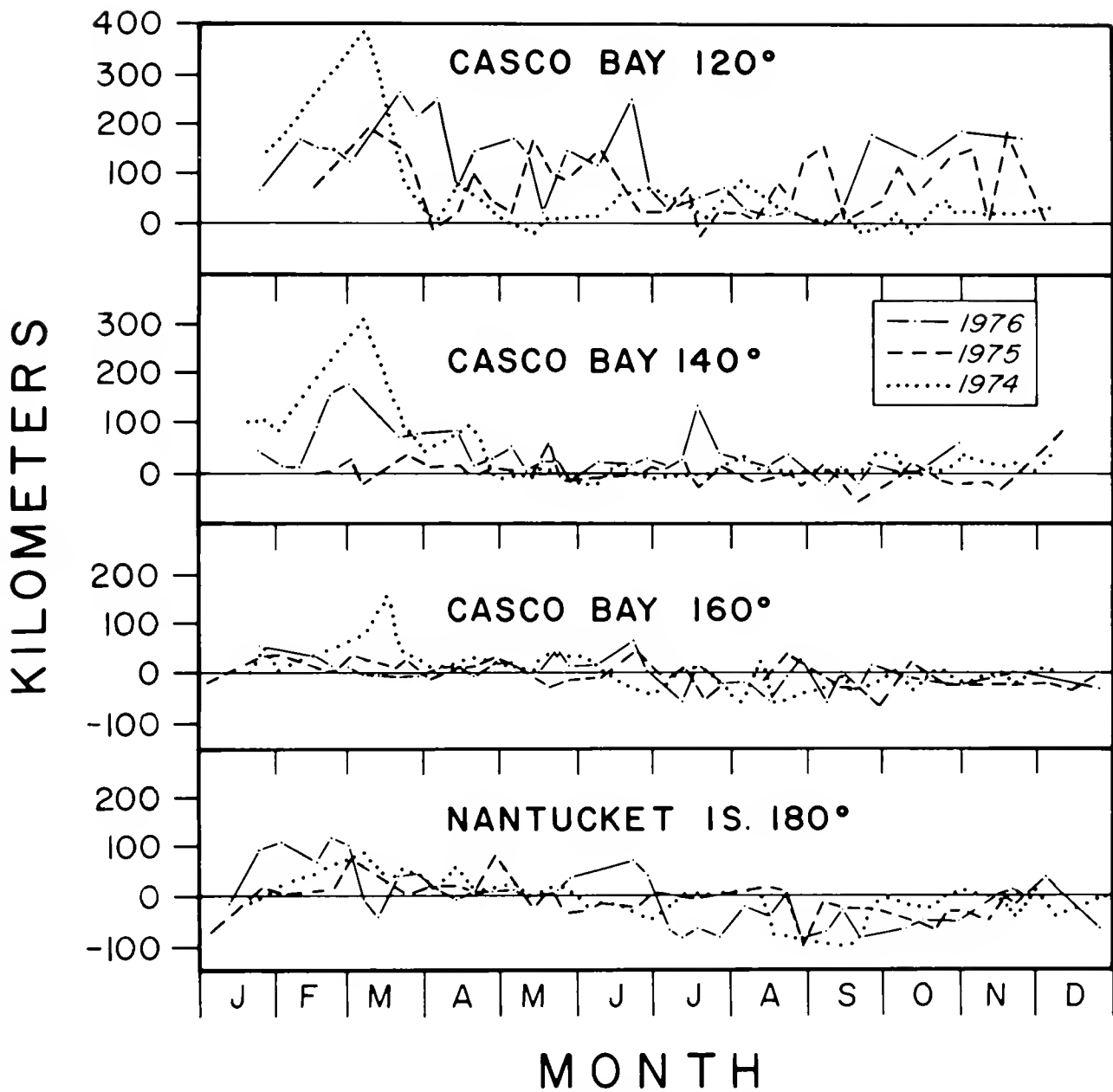
Figure 18.3.—Annual march of Shelf Water front positions relative to the 200-m isobath (positive is seaward), 1974-76, along standard bearing lines for New England and the Middle Atlantic regions.
