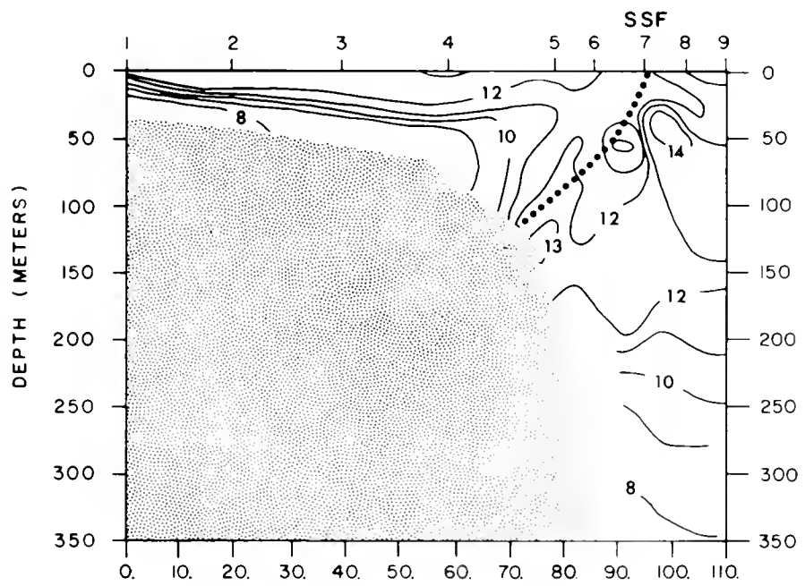
Figure 14.11.—Horizontal distribution of sea surface temperature (degrees C) and sea surface salinity (‰) and vertical distribution of temperature (degrees C) in the upper 100 and 350 m; Delaware II 76-05, 17-24 May 1976.
