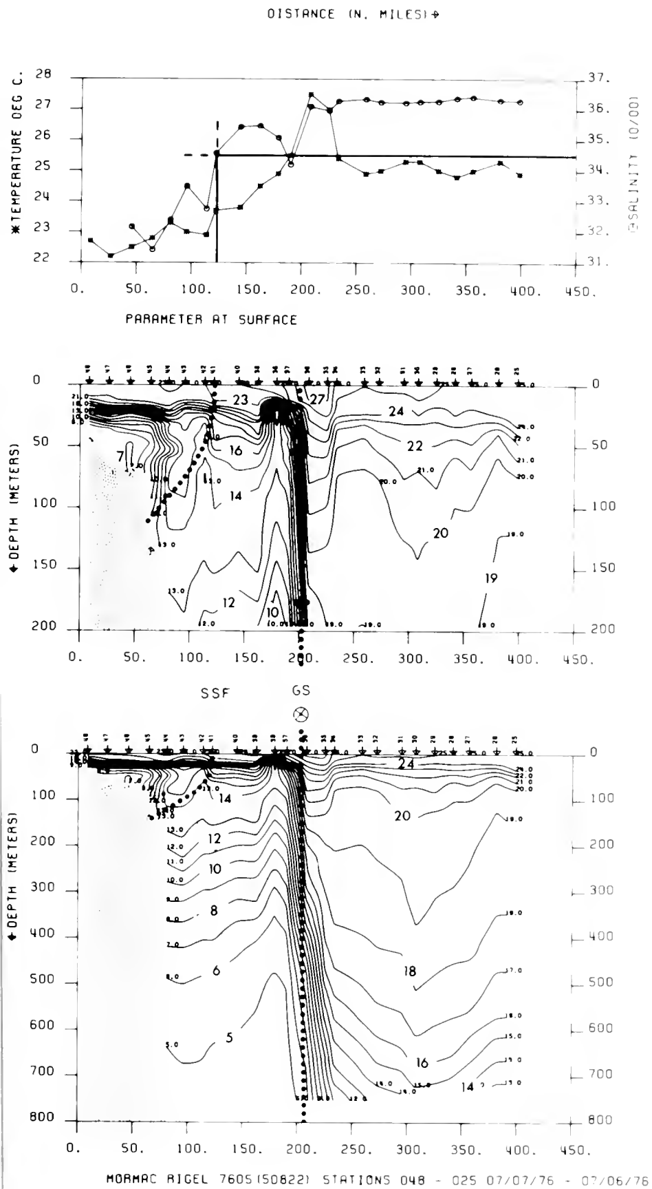
Figure 14.13.—Horizontal distribution of sea surface temperature (degrees C) and sea surface salinity (‰) and vertical distribution of temperature (degrees C) in the upper 200 and 800 m; Mormac Rigel 76-05 , 6-7 July 1976.
