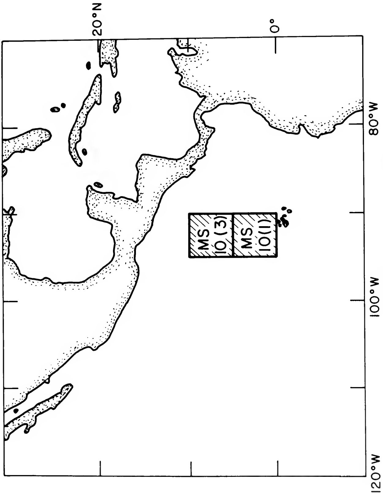
Figure 8.1.—Locations of Marsden Square quadrants 10(1) and 10(3). See Table 8.1.
