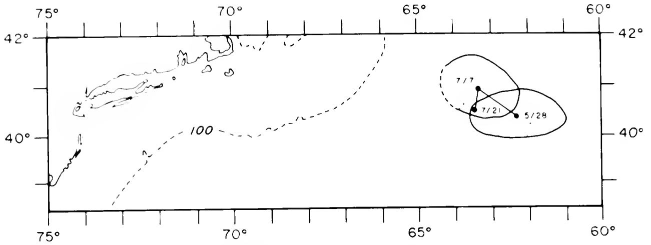
Figure 15.5.—Track line for anticyclonic eddy 76E (28 May-24 July 1976). Surface boundaries, as seen on satellite imagery, are shown for some positions.
