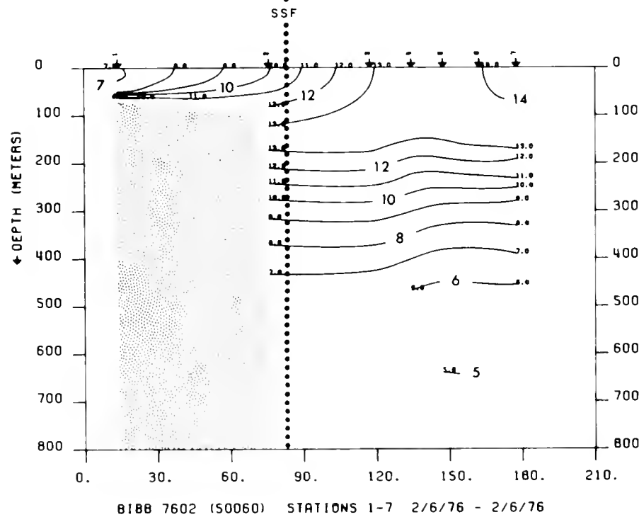
Figure 14.4—Horizontal distribution of sea surface temperature (degrees C) and sea surface salinity (‰) and vertical distribution of temperature (degrees C) in the upper 200 and 800 m; USCGC Bibb 76-02, 6 February 1976.
