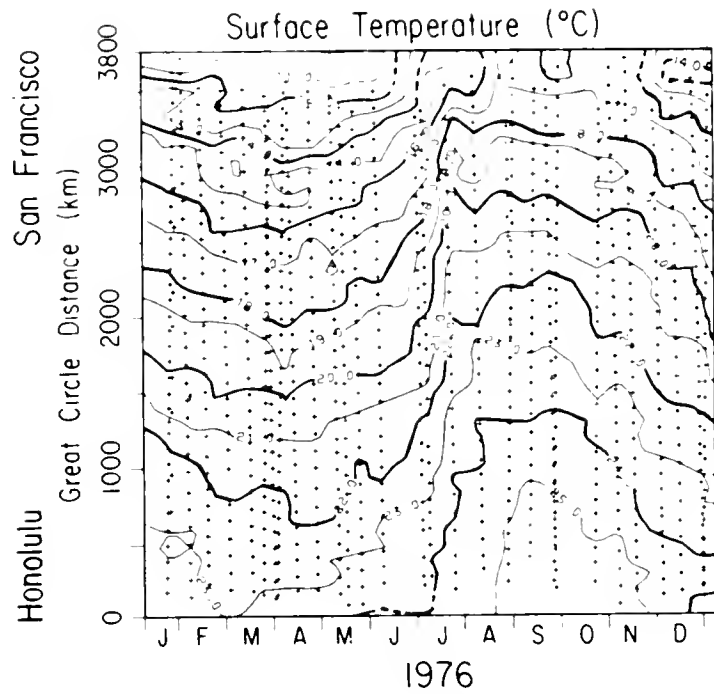
Figure 7.3.—Sea surface temperature in degrees Celsius (C) between San Francisco and Honolulu during 1976. Symbols (+) indicate the locations of observations in time and distance. Contour interval is 1.0C.
