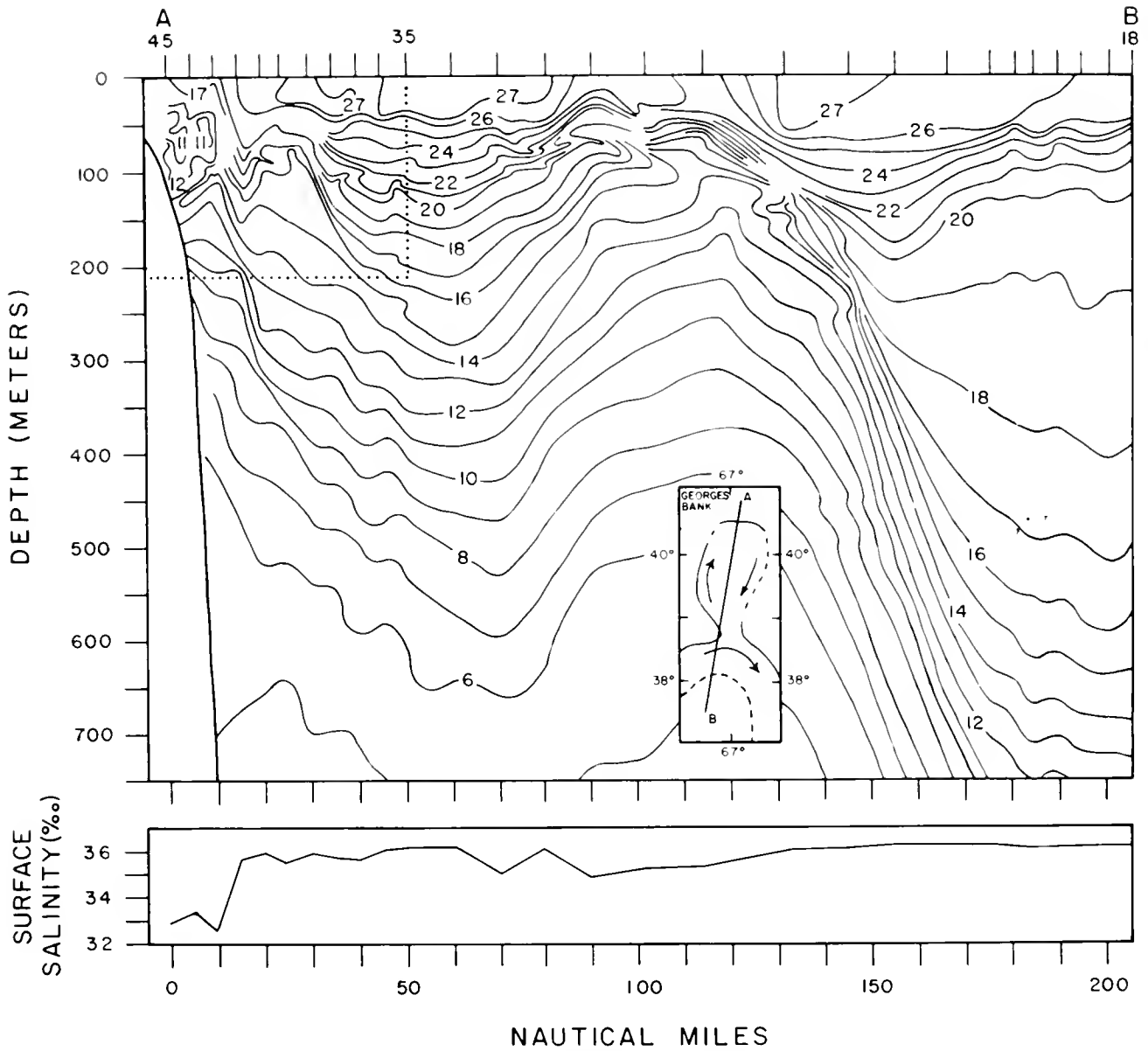
Figure 15.13.—Expendable bathythermograph section (degrees C) and surface salinities (‰) through eddy 76D and the Gulf Stream on 5-6 September 1976 from RV Belogorsk . See Figure 15.14 for detail of upper left corner of section. Location of section is shown on inset map.
