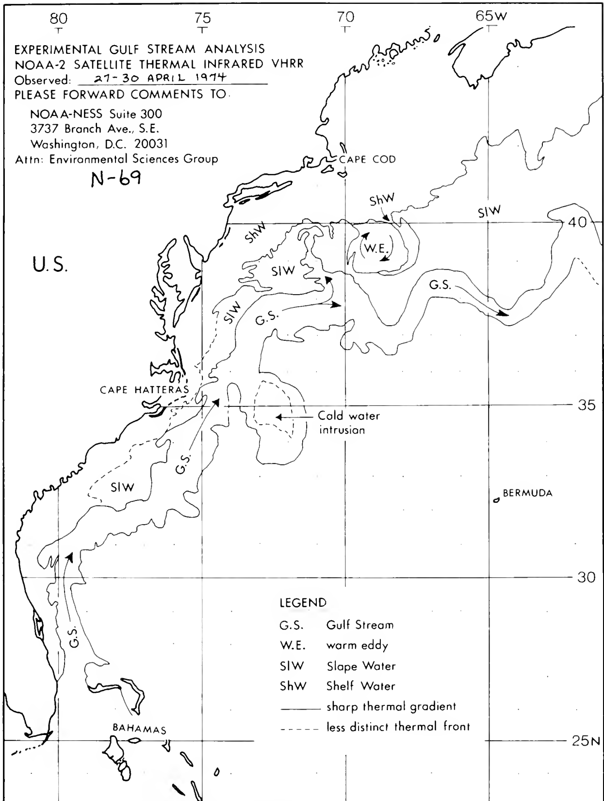
Figure 18.1.—Example of weekly Experimental Gulf Stream Analysis chart produced by Environmental Sciences Group, NESS, NOAA, Washington, DC.
