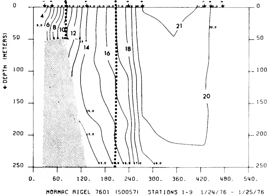
Figure 14.1.—Horizontal distribution of sea surface temperature (degrees C) and sea surface salinity (‰) and vertical distribution of temperature (degrees C) in the upper 50 and 250 m; Mormac Rigel 76-01 , 24-25 January 1976.
