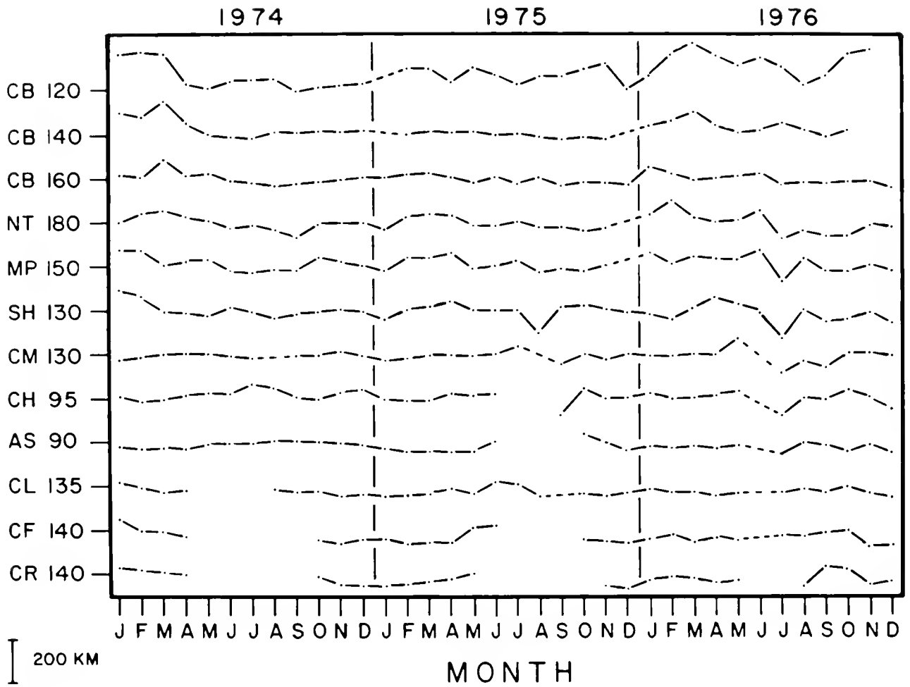
Figure 18.6.—Monthly mean Shelf Water front positions, relative to 200-m isobath (positive is seaward), 1974-76, along standard bearing lines.
