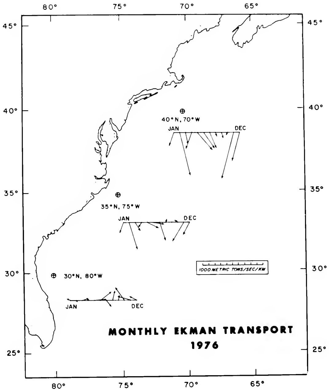
Figure 12.1.—Mean monthly Ekman transports for three representative points off the U.S. Atlantic coast for 1976.
