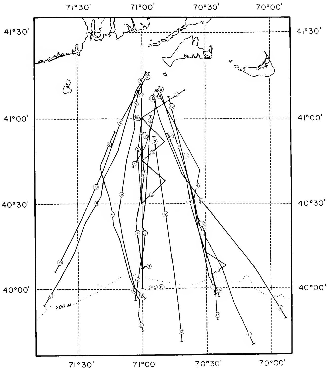
Figure 19.1.—Locations of vertical temperature sections included in this report. Sections are numbered chronologically. See Appendix 19.1 for identification of sections.
