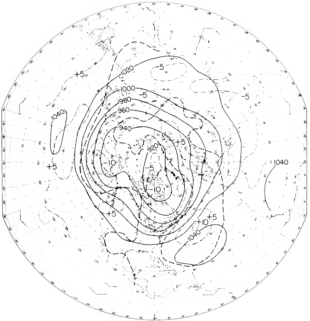
Figure 2.1.—Mean annual height of 700 mb pressure surface and its anomaly (departure from the long-term, 1948-72, mean) in ft/10.
