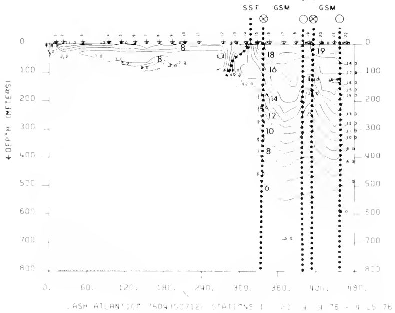
Figure 14.9.—Horizontal distribution of sea surface temperature (degrees C) and sea surface salinity (‰) and vertical distribution of temperature (degrees C) in the upper 200 and 800 m; Lash Atlantic 76-04, 24-25 April 1976.
