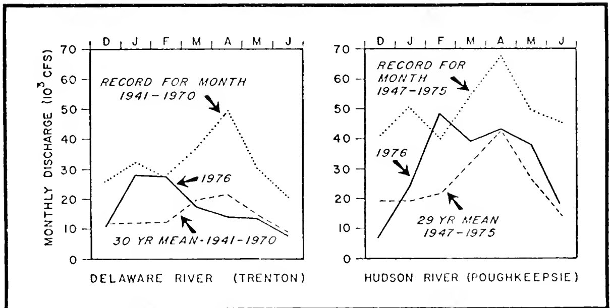
Figure 17.3.—Monthly river discharge rates for 1976 and long-term means and extremes (from U.S. Geological Survey provisional records).
