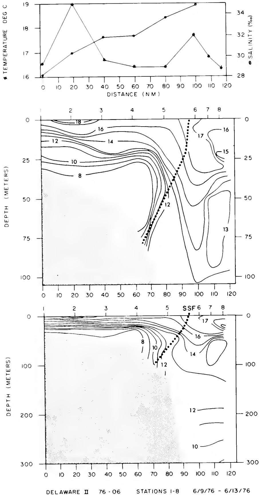
Figure 14.12.—Horizontal distribution of sea surface temperature (degrees C) and sea surface salinity (‰) and vertical distribution of temperature (degrees C) in the upper 100 and 300 m; Delaware II 76-06, 9-13 June 1976.
