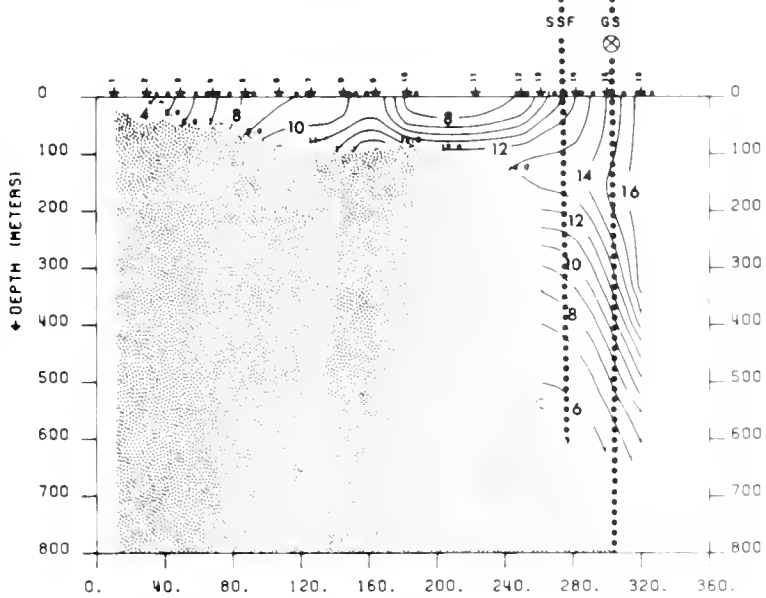
Figure 14.5.—Horizontal distribution of sea surface temperature (degrees C) and sea surface salinity (—) and vertical distribution of temperature (degrees C) in the upper 200 and 800 m; Export Defender 76-02 , 7-8 February 1976.
