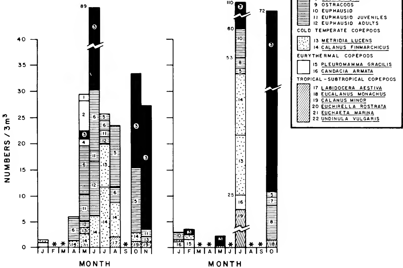
Figure 20.6.—Zooplankton (> mm) abundance per 3 m 3 in Shelf Water of the New York and Chesapeake Bights, 1976. See text for explanation of abundance units.
