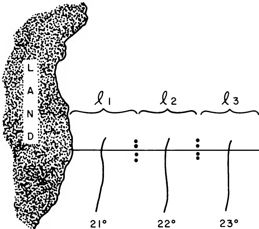
Figure 13.1.—Formula and graphic portrayal of method used to calculate distance weighted mean sea surface temperature from contoured isotherm chart.
