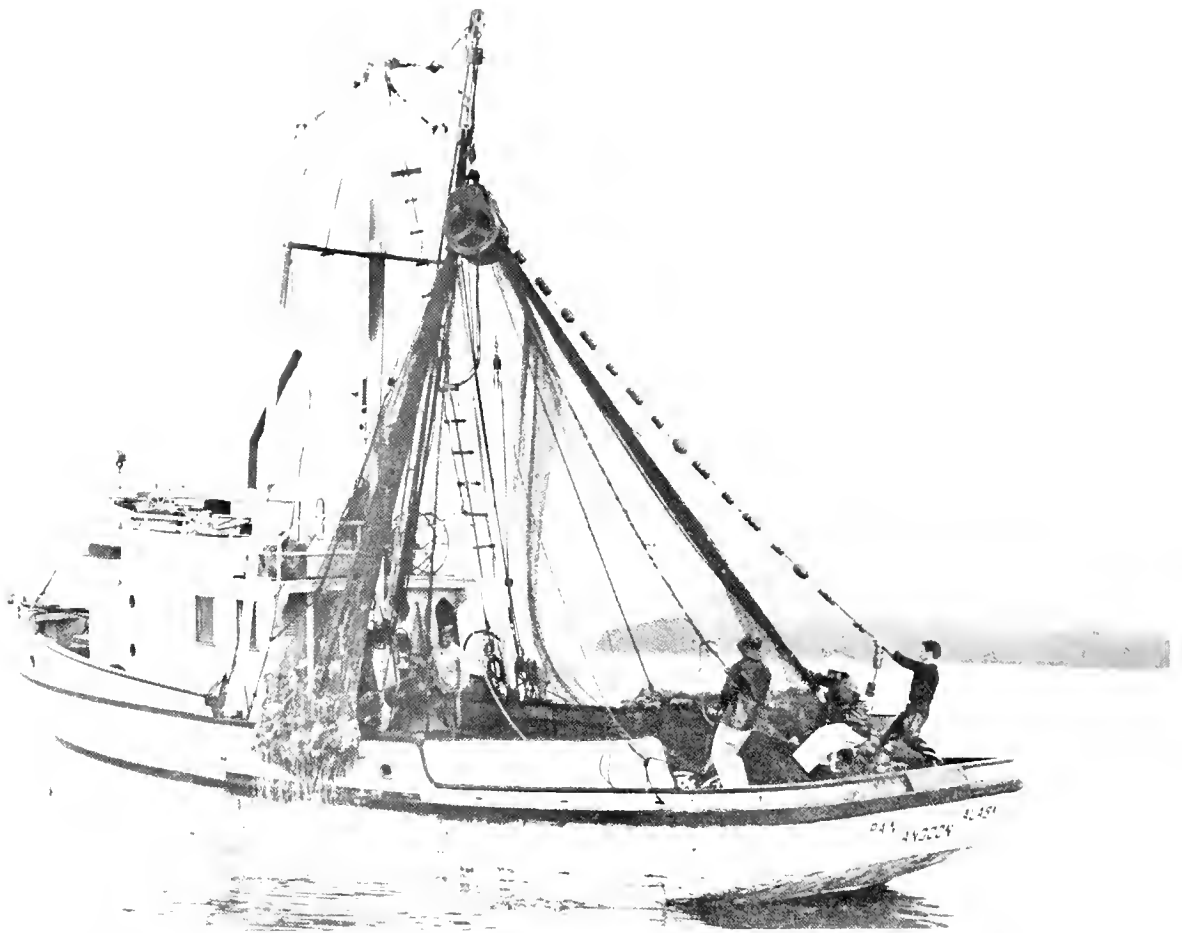
Figure 5.—Hauling in the net on a pink salmon purse seiner. When set for fishing, the net encloses an area of about 2 acres.
