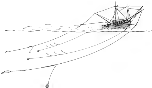
Salmon troll line
