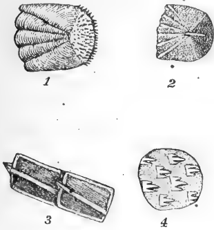
Fig. 5. 1, Ctenoid scale from perch; 2, Cycloid scale from lateral line of gold carp; 3, Ganoid scales from anablypterus; 4, Placoid scales from small-spotted dog-fish.
