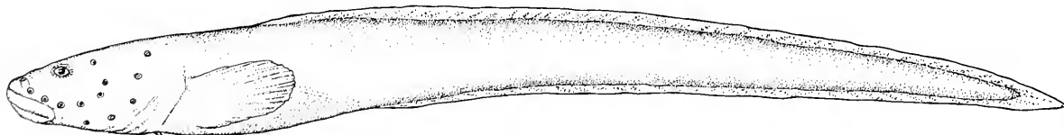
Fig. 4. Lycenchelys argentina , 26 cm TL, drawn from a photograph of the holotype in Marschoff et al. (1977)
