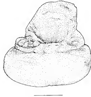
Fig. 22. Representative otolith of N. ionah ; fish length 46 cm SL; scale bar 1 mm
