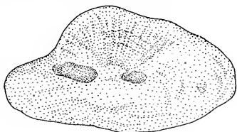
Fig. 14. Representative otolith of H. velifer ; fish length 129 mm TL; scale bar 1 mm
