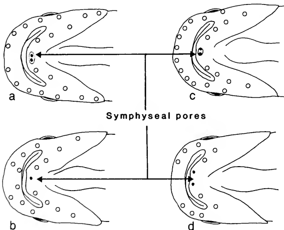
Fig. 3. Various conditions of the preopercular-mandibular symphyseal pores in Antarctic liparidid fishes: Careproctus (a); Genioliparis and Notoliparis (b); Paraliparis (a-d)
