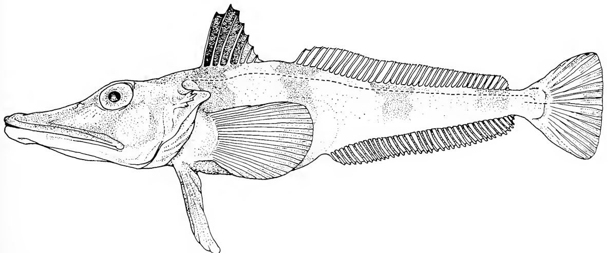
Fig. 1. Chanocephalus aceratus IBUT 82–702, 45 cm SL, off South Shetland Islands (61°15'S, 55°02' W)
