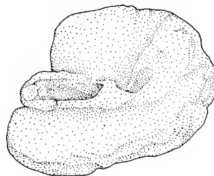
Fig. 53. Representative otolith of T. nicolai ; fish length 22 cm SL; scale bar 1 mm
