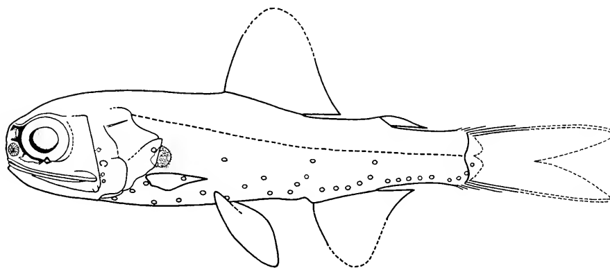
Fig. 4. Diaphus hudsoni , 30 mm SL (from Smiths' Sea Fishes )
