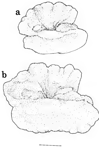
Fig. 9. Representative otoliths of C. rhinocerus ; fish lengths: (a) 24 cm, (b) 50 cm TL; scale bar 1 mm
