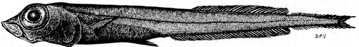
Fig. 2. Leptoderma sp. A, from a photograph of Leptoderma sp. 1 of Sazonov & Ivanov (1980)
