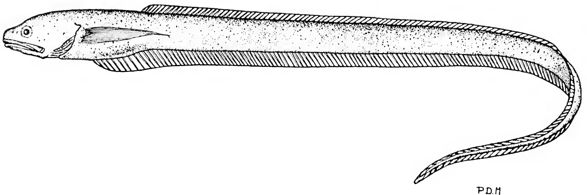
Fig. 1. Echiodon cryomargarites LACM 42953-001, 30.8 mm HL, 34 cm TL, female (53°13'–16'S, 75°41'W)
