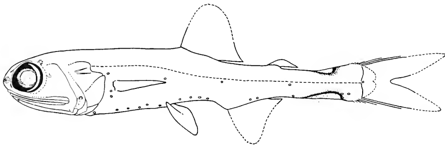
Fig. 56. Taaningichthys bathyphilus , 50 mm SL (from Smiths' Sea Fishes )
