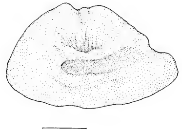
Fig. 5. Representative otolith of B. antarcticus ; fish length unknown; scale bar 1 mm
