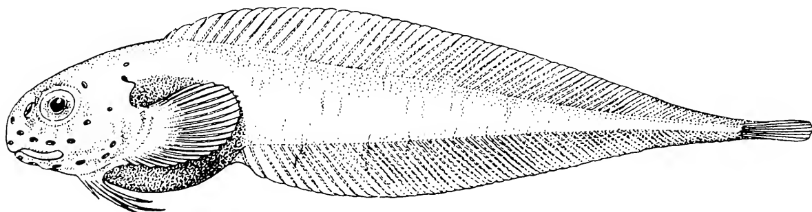
Fig. 32. Paraliparis tetrapteryx ZIN 44095, 110 mm SL, holotype, male (from Andriashev, 1986)
