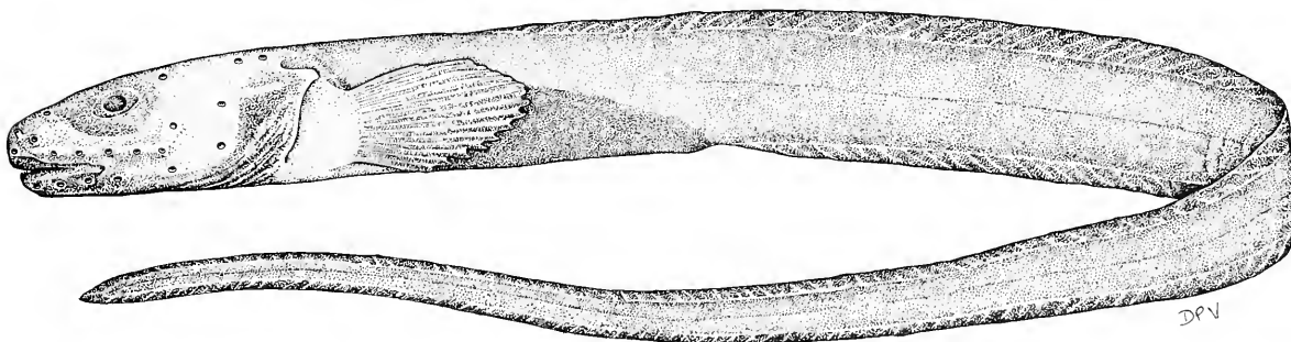
Fig. 6. Lycenchelys hureaui MNHN 1984-727, 26 cm SL, Kerguelen Islands
