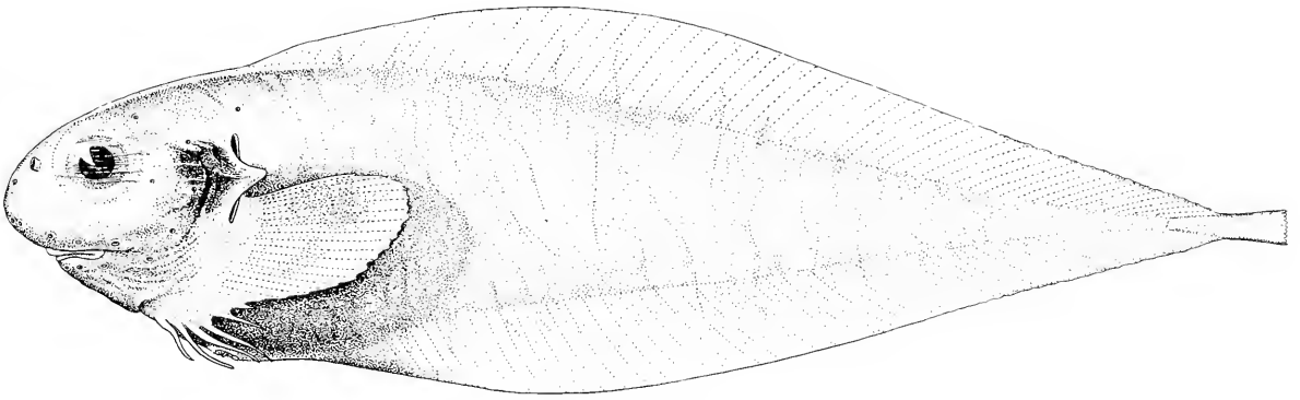
Fig. 29. Paraliparis somovi ZIN 44100, 192 mm SL, holotype, female (from Andriashev, 1986)
