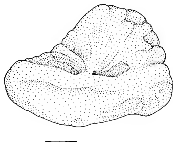
Fig. 55. Representative otolith of T. pennellii ; fish length 190 mm SL; scale bar 1 mm
