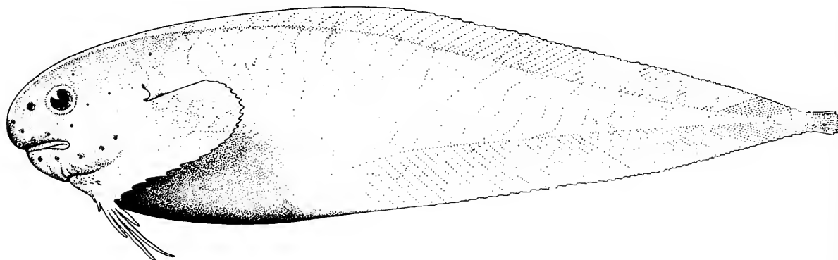
Fig. 26. Paraliparis monoporus ZIN 44094, 24 cm SL, holotype, female (from Andriashev, 1986)
