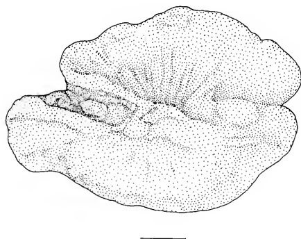
Fig. 3. Representative otolith of A. mitopteryx ; fish length 37 cm TL; scale bar 1 mm
