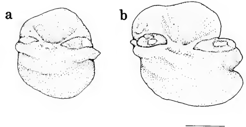
Fig. 20. Representative otoliths of D. hunteri ; fish lengths: (a) 22 cm, (b) 24 cm TL; scale bar 1 mm
