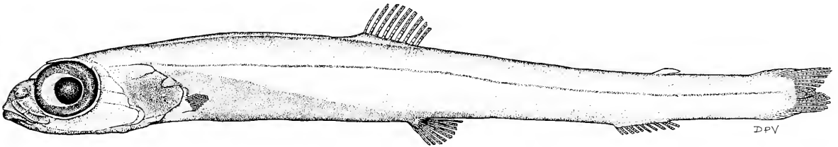
Fig. 1. Nansenia antarctica BAS 831406, 108 mm SL (56°06'S, 37°22'W)
