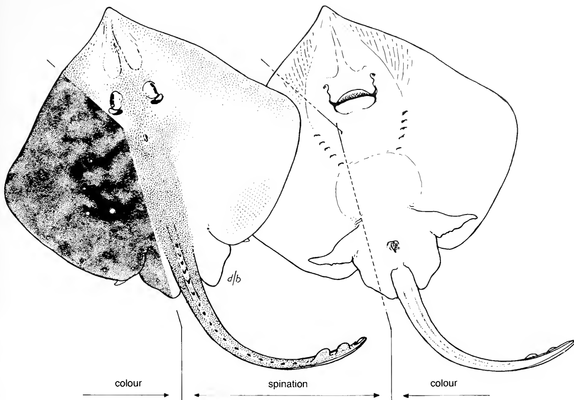
Fig. 3. Bathyraja eatonii ISH 277/81, 287 mm TL, juvenile female, off South Shetland Islands ( 61^{\circ}05.2'S , 56^{\circ}03.5'W ), 200–250 m
