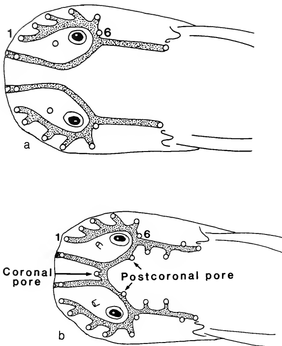
Fig. 2. Dorsal view of head sensory canals of Antarctic liparidid fishes: (a) pattern of pores in Careproctus , Genioliparis , and Paraliparis ; (b) pattern of pores in Notoliparis . Note: the coronal pore is also present in some Antarctic Paraliparis
