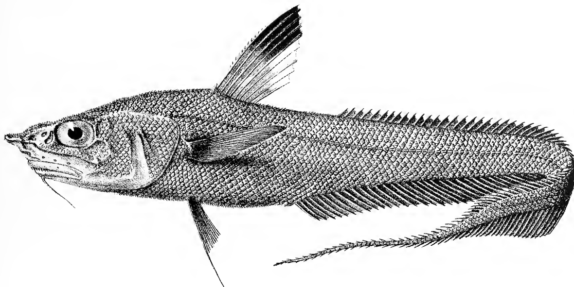
Fig. 7. Coryphaenoides ferrieri holotype, 23 cm TL (71°21'S, 16°34'W) (from Regan 1913)
