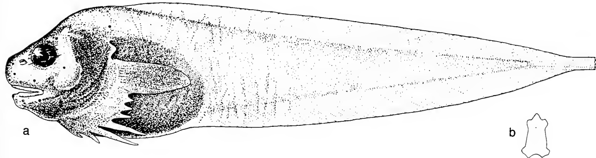
Fig. 33. (a) Paraliparis thalassobathyalis ZIN 45811, 103 mm SL, holotype; (b) premaxillary tooth of a paratype (from Andriashev, 1986)
