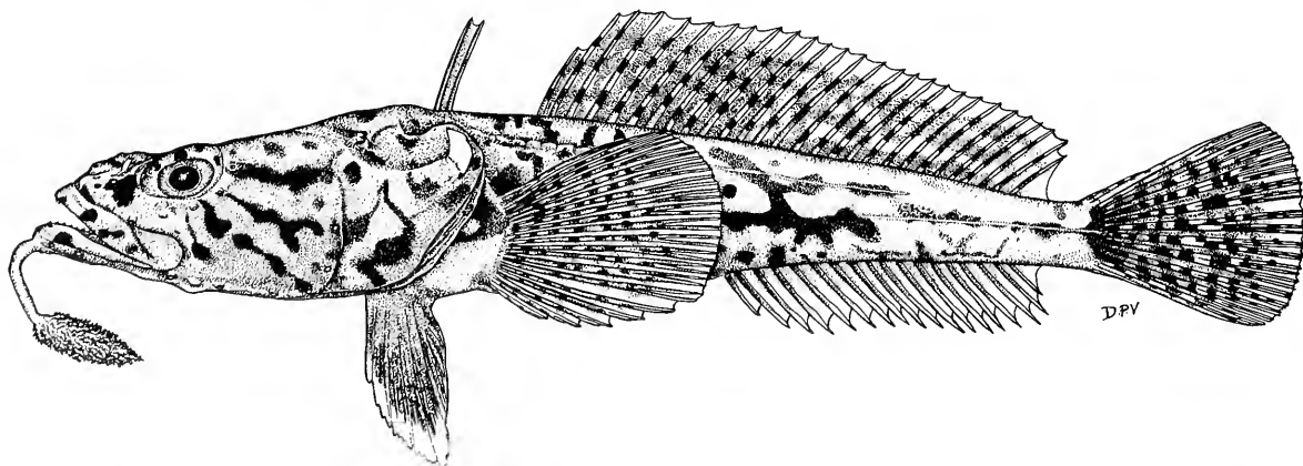
Fig. 26. Pogonophryne lanceobarbata ISH 78/85, 153 mm SL, paratype, female, Weddell Sea (77°17.6'S, 41°24.4'W)
