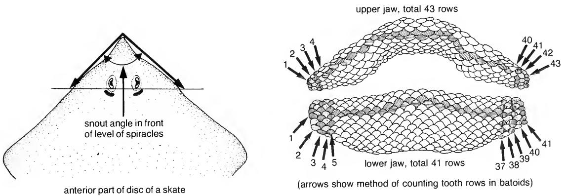
Fig. 1. Technical terms and method of measurements used in the study of skates
