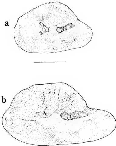
Fig. 8. Representative otoliths of A. shackletoni ; fish lengths: 91 mm (a) and 129 mm (b) TL; scale bar 1 mm
