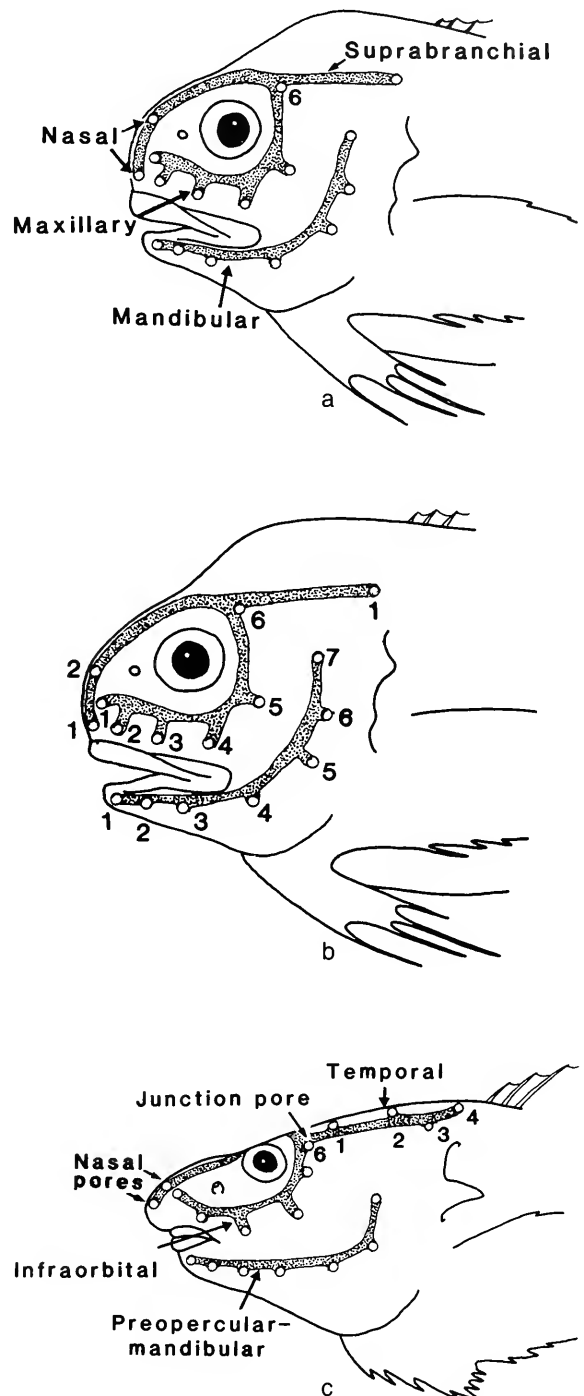
Fig. 1. Lateral view of head sensory canals of Antarctic liparidid fishes: (a) terminology of Burke (1930); (b) pattern of pores in Careproctus , Genioliparis , and Paraliparis ; (c) pattern of pores in Notoliparis and new terminology (also applies to (b))
