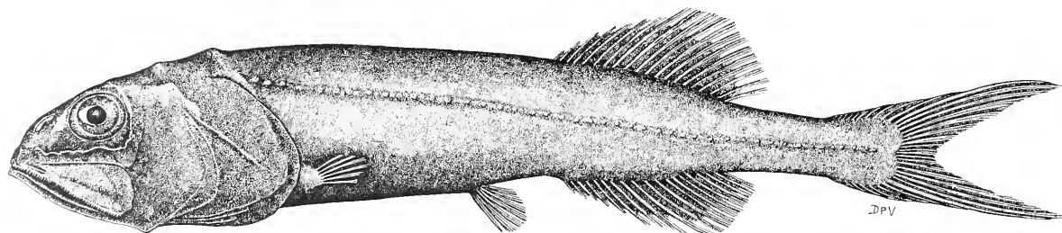
Fig. 4. Rouleina atrita USNM 215481, 37.5 cm SL, Atlantic Ocean (36°40.1'N, 74°25.4'W)
