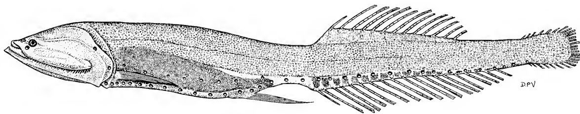
Fig. 9. Cyclothone pseudopallida ADH ex-S85/0013–0027, 42 mm SL (66°00.2'S, 67°58.1'E)
