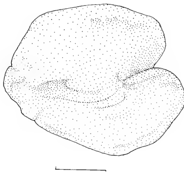
Fig. 49. Representative otolith of P. (P.) gemmatum ; fish length 64 mm SL; scale bar 1 mm
