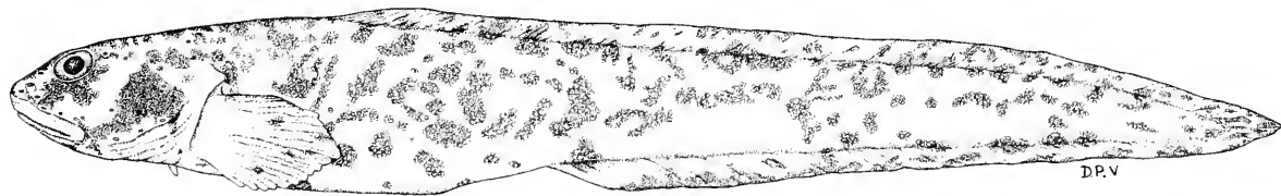
Fig. 13. Lycodichthys antarcticus AMS IA.440, 186 mm SL, Queen Mary Coast (66°18'S, 94°58'E)
