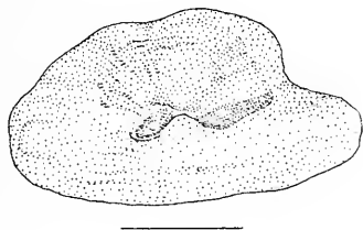
Fig. 10. Representative otolith of A. skottsbergi ; fish length 101 mm TL; scale bar 1 mm
