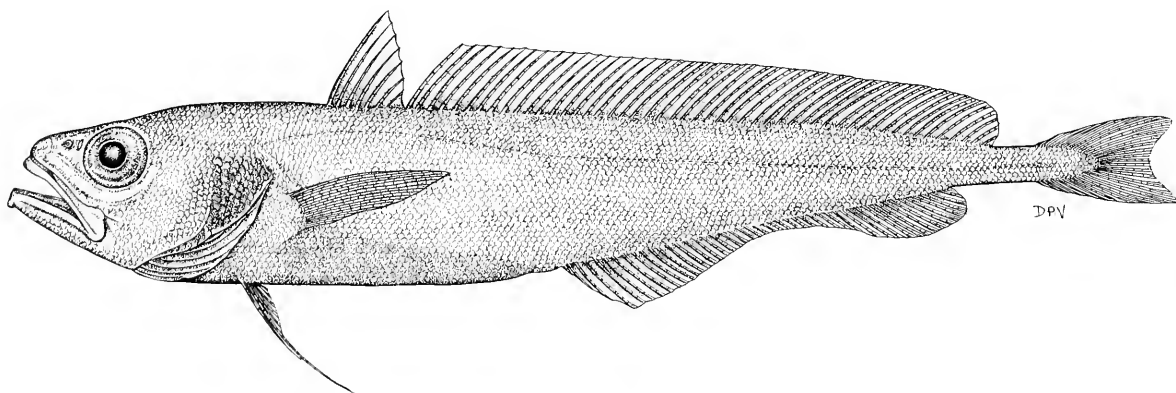
Fig. 3. Halargyreus johnsonii LACM 10985–4, 28 cm SL (52°20'S, 158°29'E)
