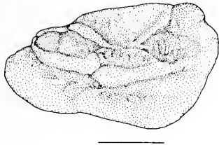
Fig. 33. Representative otolith of P. borchgrevinki ; fish length unknown; scale bar 1 mm
