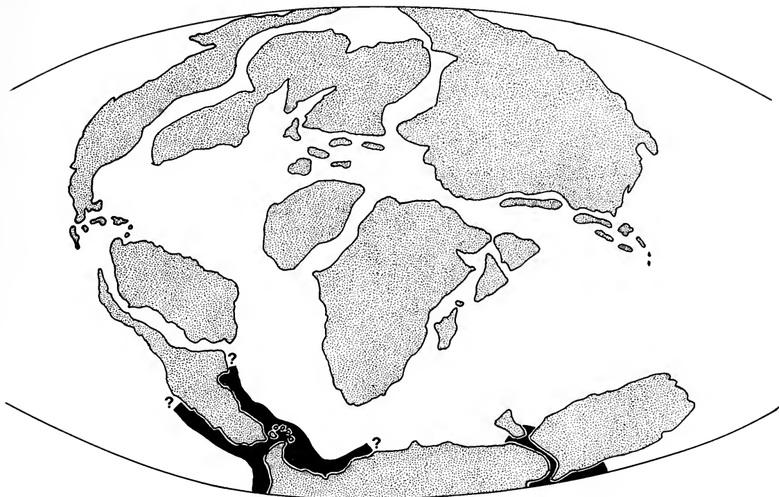
Fig. 1. Continental reconstruction during Late Cretaceous times showing the Weddellian Province (in black) of Zinsmeister (1976). Redrawn after Dietz & Holden (1970), Pindell & Dewey (1982), and Barron (1987)
