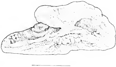
Fig. 36. Representative otolith of P. magellanica ; fish length 24 cm SL; scale bar 1 mm
