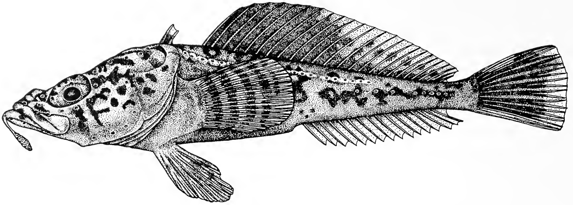
Fig. 28. Pogonophryne marmorata 176 mm (65°18'S, 91°41'E) (redrawn from Andriashev 1967)
