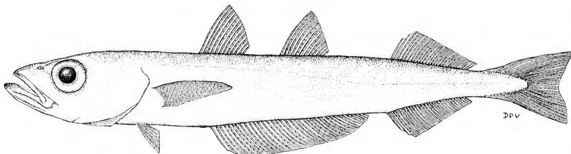
Fig. 1. Micromesistius australis LACM 10988–2, 97.7 mm SL, juvenile (50°52'S, 166°42'E)
