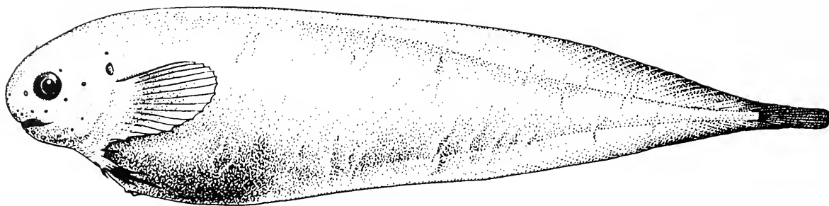
Fig. 13. Paraliparis copei kerguelensis ZIN 45825, holotype, 123 mm SL (from Andriashev, 1986)
