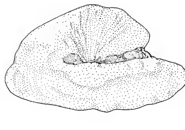
Fig. 22. Representative otolith of P. evansii ; fish length 143 mm TL; scale bar 1 mm
