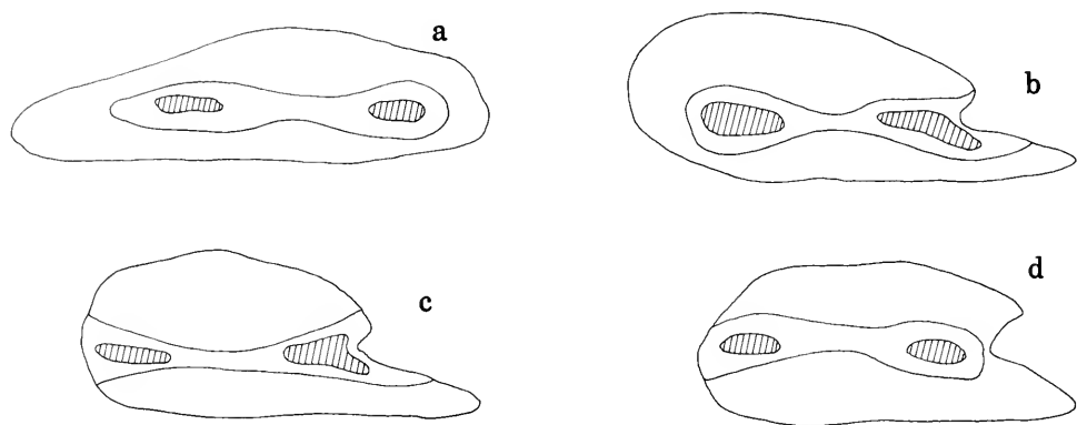
Fig. 3. Schematic diagrams of the different types of sulcus acusticus openings. a—medial (sulcus acusticus does not open onto anterior and posterior margin), b—ostial (sulcus acusticus opens only onto anterior margin), c—ostio-caudal (sulcus acusticus opens onto anterior and posterior margins), d—caudal (sulcus acusticus opens only onto posterior margin). The sulcus acusticus is outlined and the colliculi are hatched for orientation purposes
