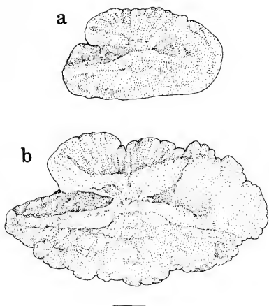
Fig. 29. Representative otoliths of N. coriiceps ; fish lengths: (a) 21 cm and (b) 46 cm TL; scale bar 1 mm
