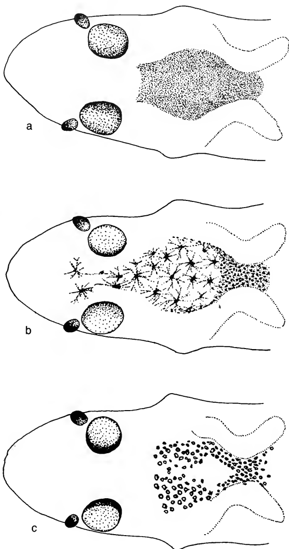
Fig. 4. Pigment pattern of the meningeal membrane (dorsal view) of Southern Ocean Cyclothone : a. acclinidens , microdon and pallida ; b. braueri ; and c. pseudopallida .
