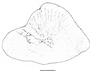
Fig. 33. Representative otolith of P. phyllopogon ; fish length 152 mm SL; scale bar 1 mm
