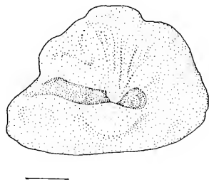
Fig. 9. Representative otolith of B. marri ; fish length 196 mm SL; scale bar 1 mm
