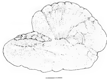
Fig. 20. Representative otolith of P. georgianus ; fish length 51 cm TL; scale bar 1 mm
