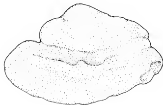
Fig. 57. Representative otolith of T. scotti ; fish length 123 mm SL; scale bar 1 mm
