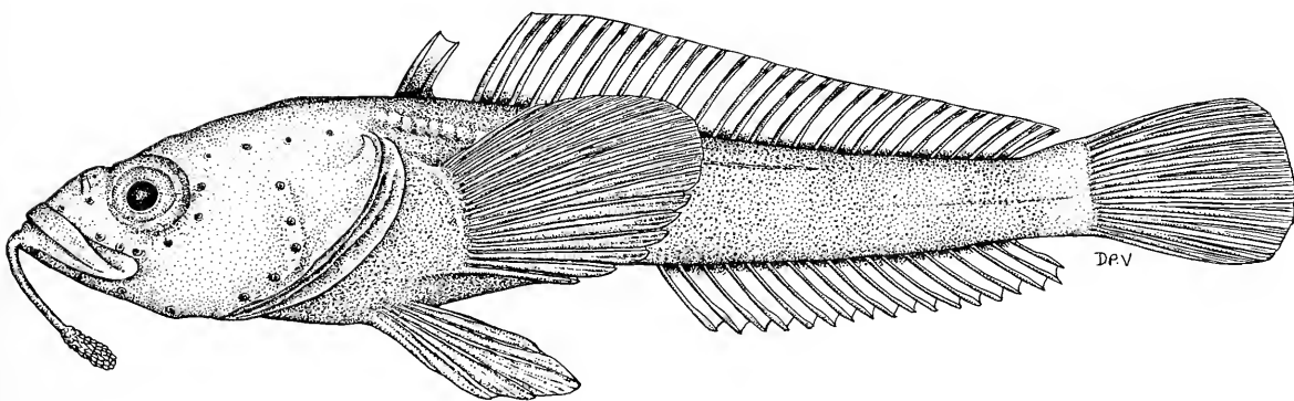
Fig. 17. Pogonophryne albipinna LACM 11353–1, 37.5 mm SL, holotype, juvenile
