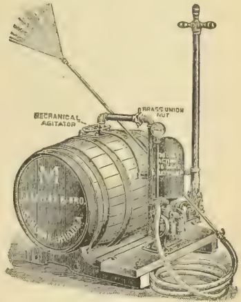
Fig. 1518. Pressure Gauge, 15 foot seven ply hose, one nozzle, one eight foot extension pipe with lever shut off and mechanical agitator. Ready to spray. Delivered any where in America—$53.50.
