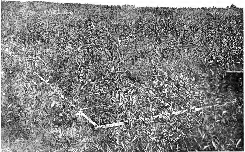
FIG. 2.—Late serotinal aspect: Solidago rigida and Helianthus scaberrimus on upper slope.
