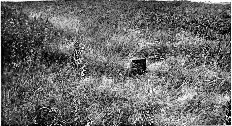
FIG. 1.—Serotinal aspect: Bouteloua curtipendula sod on upper slope; Solidago rigida to the left; Helianthus scaberrimus to the right; admixture in the background.
