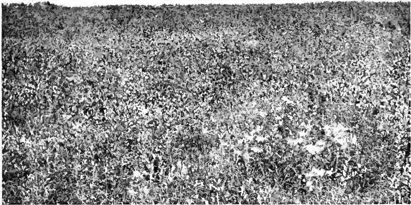
FIG. 1.—Late estival aspect; Ratibida columnaris upon a middle slope; the ruderal Hordeum jubatum in right foreground.
