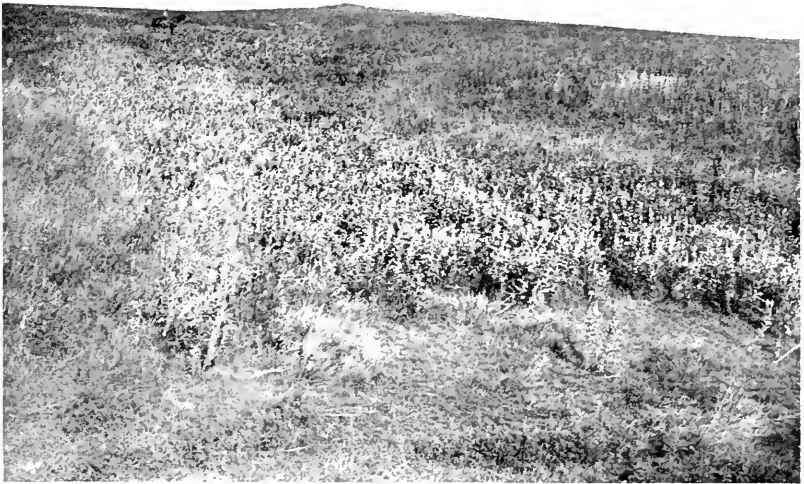
FIG. 2.—Late estival aspect; Symphoricarpus association in a depression of a northwest exposure; Poa sod in foreground.
