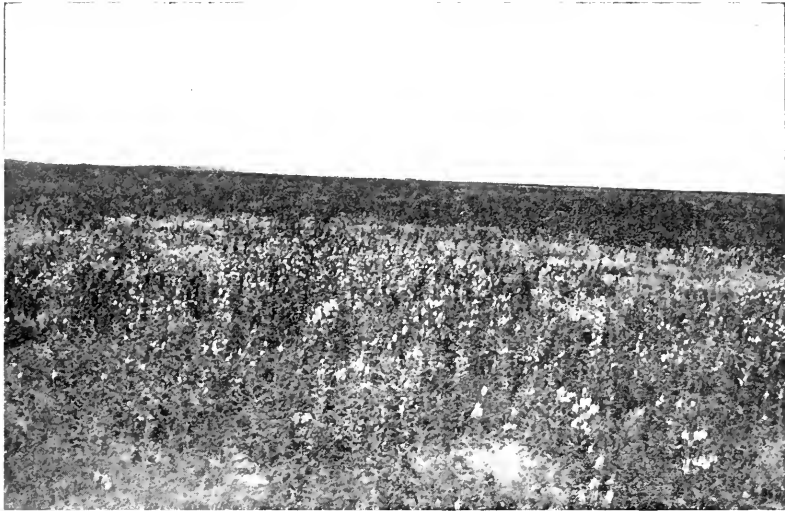
FIG. 3.—Late estival aspect; Verbena stricta determining the tone of a lower slope; the white patches are the ruderal Hordeum jubatum .
