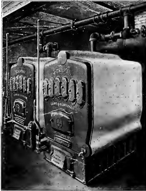
Get it out of your mind that setting boilers in battery requires complicated piping. This battery of two replaced one large tubular boiler in a greenhouse at Allegheny, Pa.
