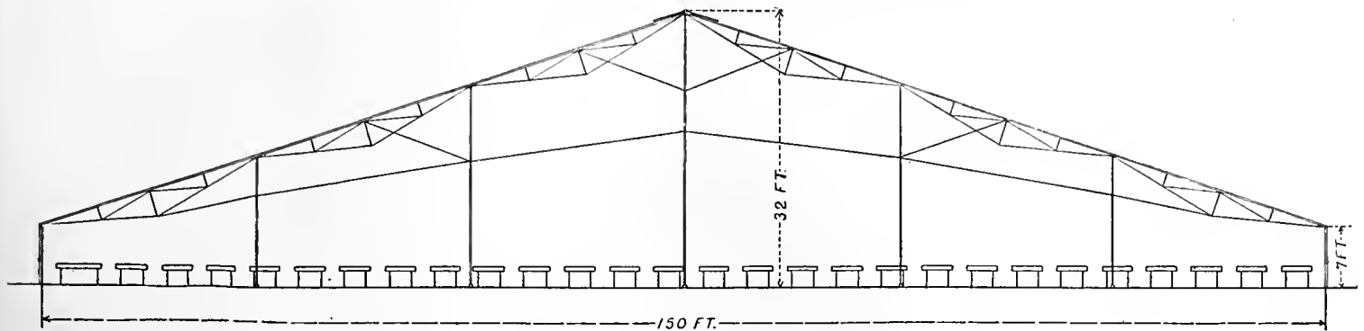
Greenhouse Construction—Design of Even Span 150-Foot House
