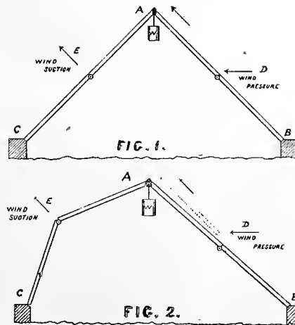
Wind and Greenhouse Roofs.
