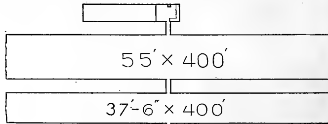
Plan of Coddington Wide Greenhouse
