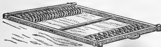
Meeker's Disc Smoothing Harrow.
