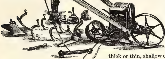
"PLANET JR." No. 25 SEEDER.
