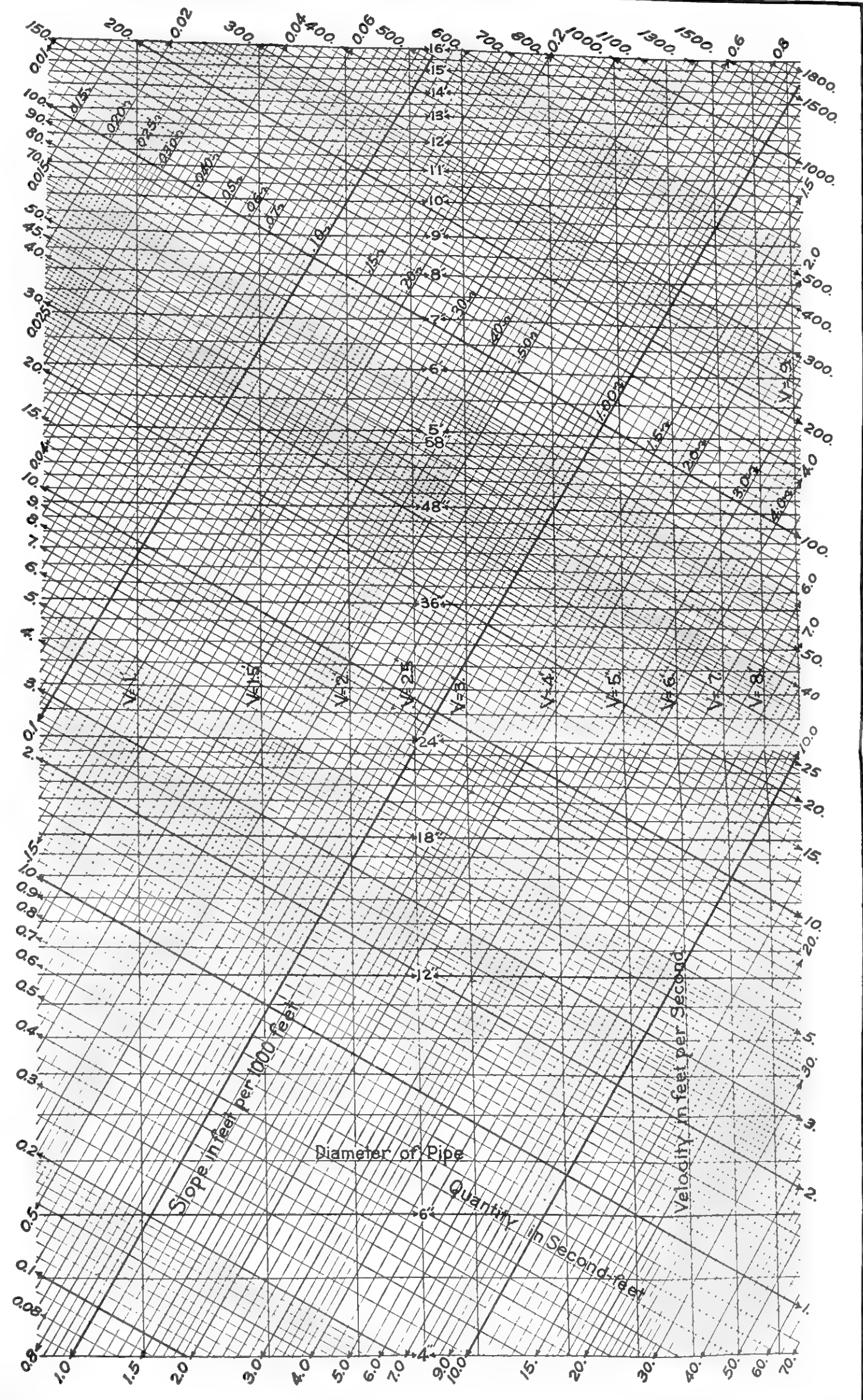
LOGARITHMIC DIAGRAM FOR USE IN DESIGNING WOOD-STAVE PIPE. BASED ON FORMULA: Q = 1.272D^2 \cdot H^{0.54} .
