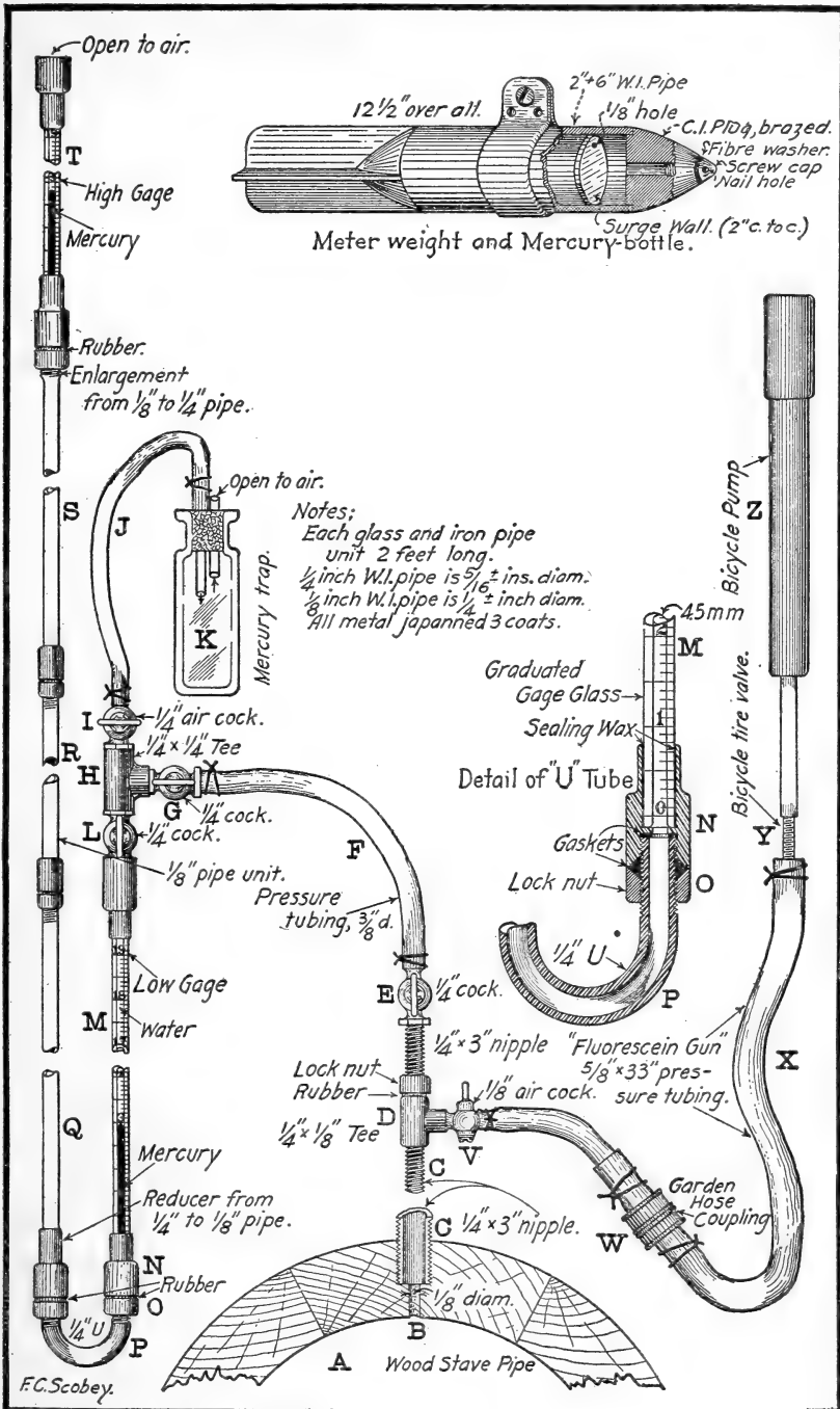
FIG. 3.—Method of attaching mercury manometers to wood-stave pipes. Details of manometers, fluorescein gun, and combined current meter weight and mercury bottle.
