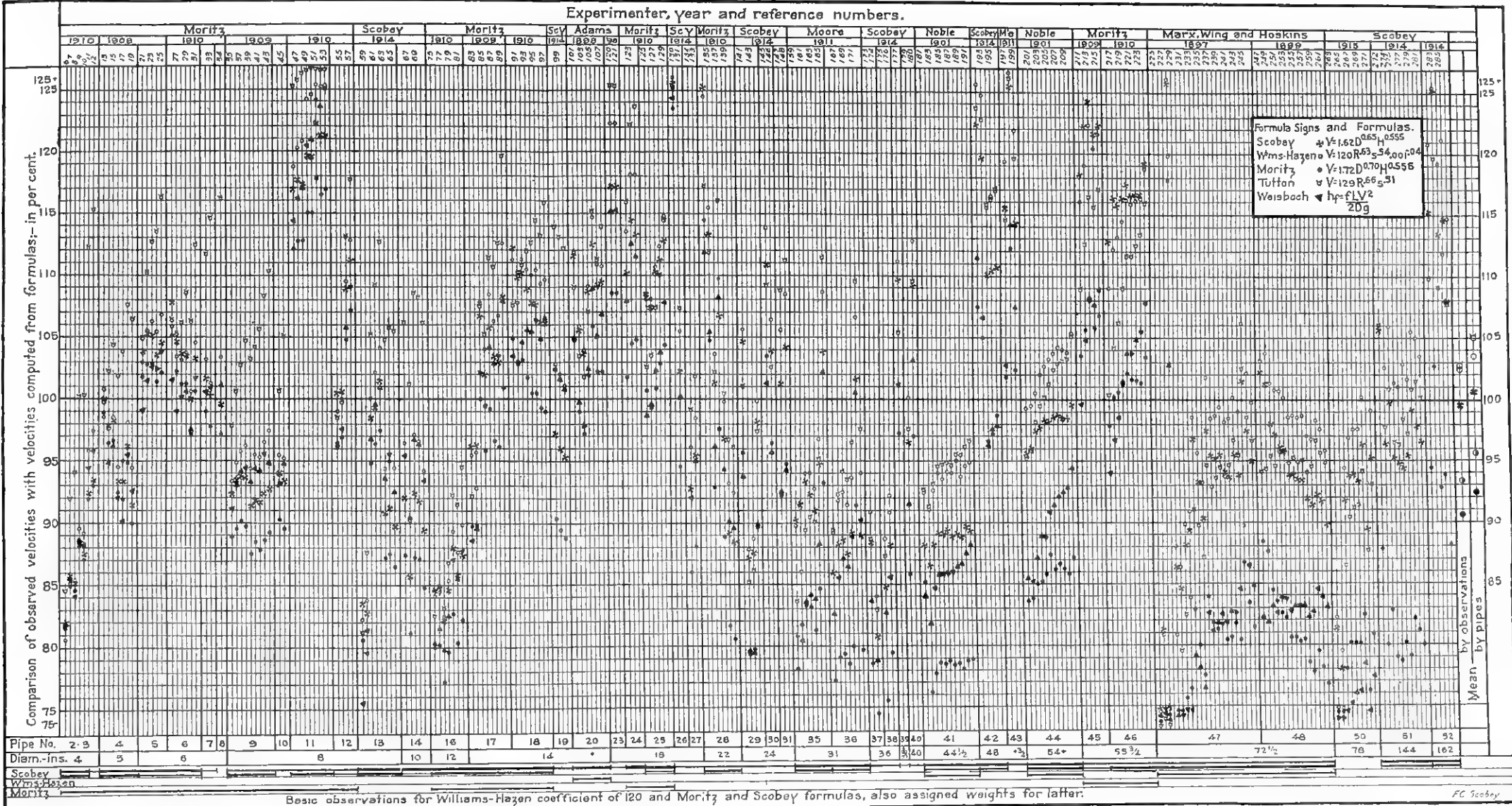
CHART SHOWING DEGREE OF CONFORMITY OF OBSERVED VELOCITIES OF WATER IN WOOD-STAVE PIPES TO CALCULATED VELOCITIES FOR GIVEN LOSS OF HEAD, BY SCOBEY, WILLIAMS-HAZEN (C w =120), MORITZ, TUTTON, AND WEISBACH FORMULAS. 08796-25. (Page p. 54.)
