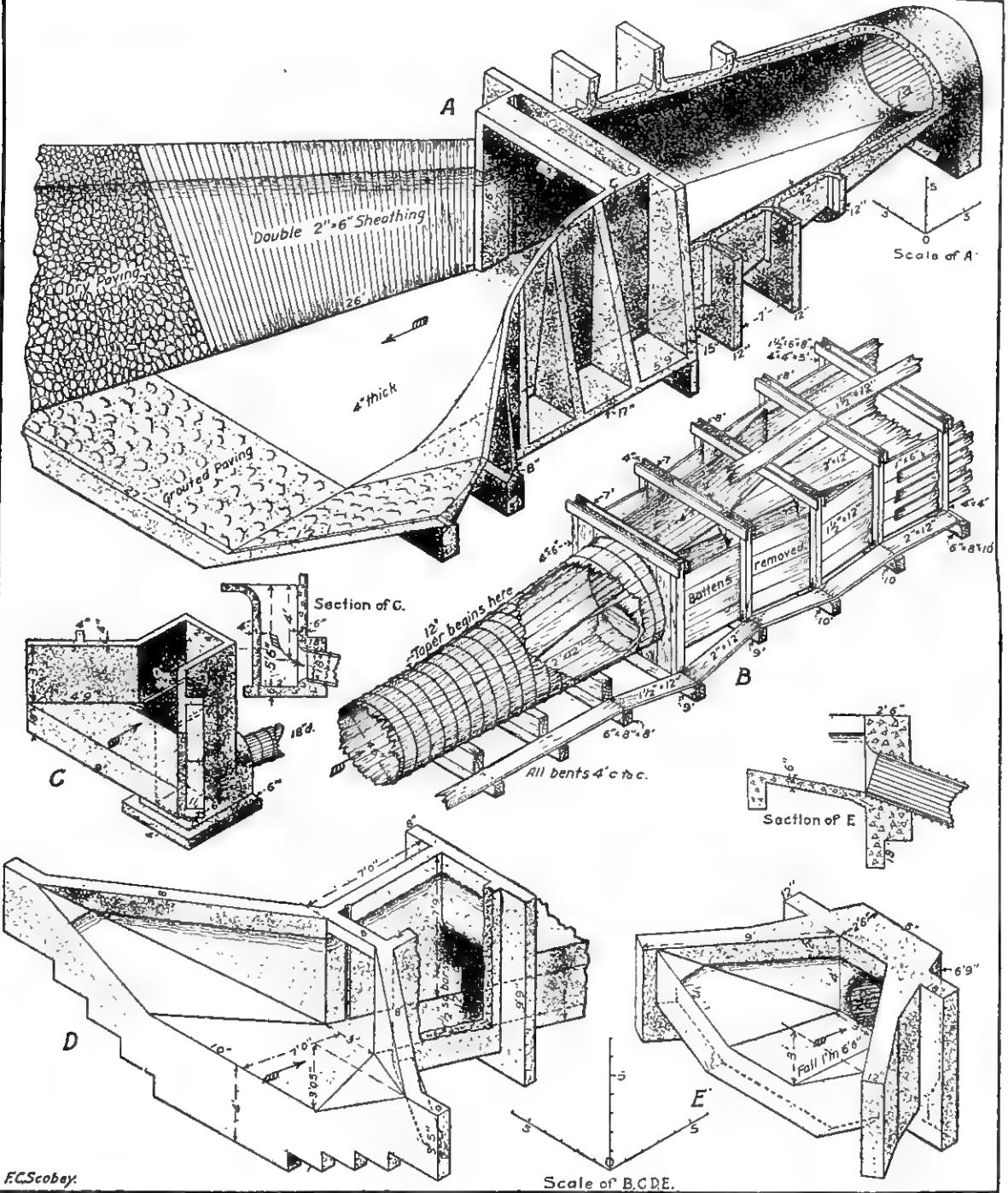
SUGGESTIVE INLET AND OUTLET STRUCTURES FOR INVERTED SIPHONS.
