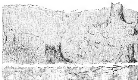
SECTION OF A BOG CONTAINING FILL-STUMPS.
