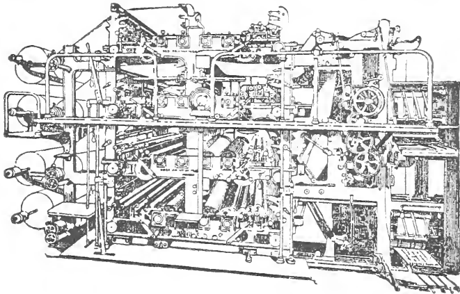
THE GOSS STRAIGHT LINE FOUR DECKER.
