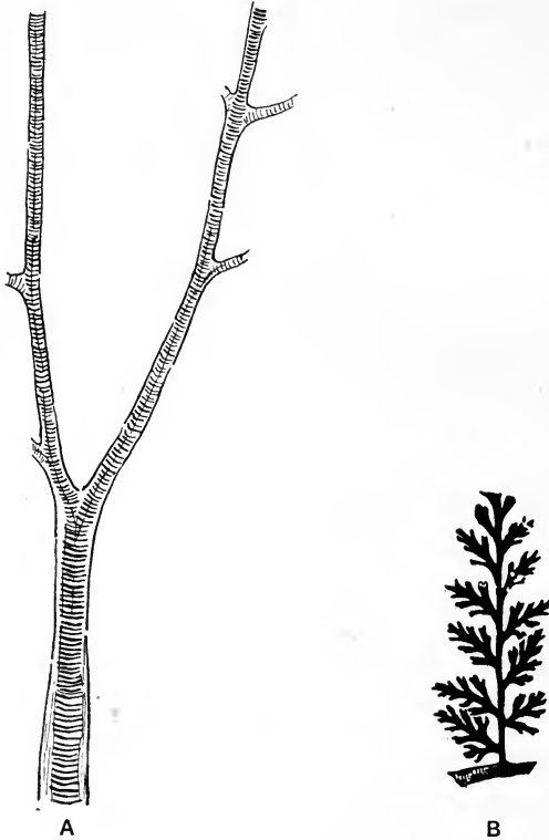
FIG. 413. Sphenopteris ( Diplomema ) elegans . A. Forked rachis with bases of lateral branches (Kidston Coll.); B, pinna. (After Stur.)
