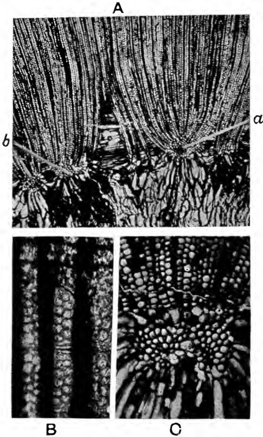
FIG. 489. Callixylon Triflievi . A, C, the inner margin of the secondary xylem showing strands of primary xylem, a , b , and C. B, tracheids of the secondary xylem. (A, C, from photographs supplied by Prof. Zalessky; B, Cambridge Botany School.)
