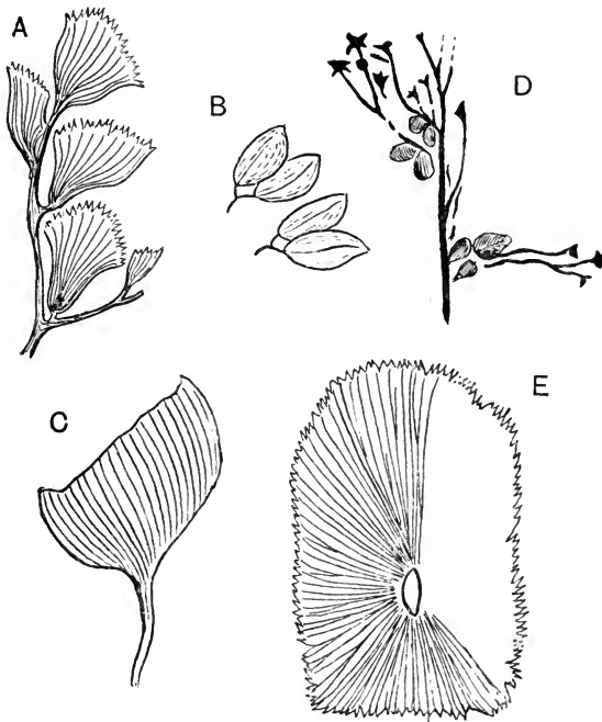
FIG. 421. A. Potonia adiantiformis Zeill. (very slightly enlarged). B. Microsporangia of Potonia (enlarged). C. Linopteris obliqua ; side-view of microsporophyll. D. Neuropteris heterophylla , pinnules and microsporangia (?). E. Linopteris obliqua , surface-view of microsporophyll. (A, C, E, after P. Bertrand; B, after Carpentier; D, after Kidston.)
