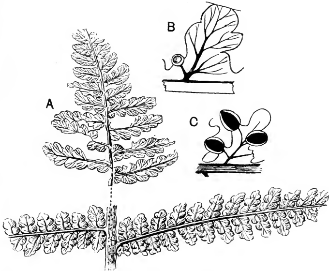
FIG. 442. Pecopteris Pluckenetii . A, apex and lower pinnae (Kidston Coll., 234); B, pinnule with supposed sori (after Sterzel); C, pinnule with seeds (after Zeiller).
