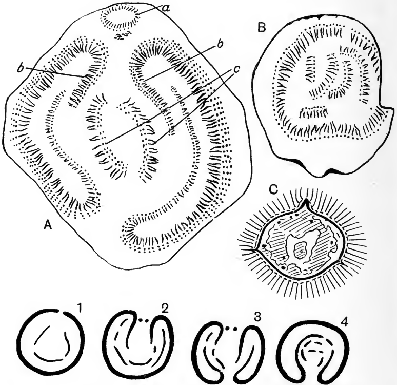
FIG. 453. A. Ptychoxylon Levyi ; transverse section of stem; a, stela of branch. (After Renault.) B. Cycadoxylon Fremyi ; transverse section of stem. (After Renault.) C. Cycadoxylon robustum ; centre of stem. 1—4, diagrams of sections of the stem of Ptychoxylon at different levels. (Simplified from Renault)
