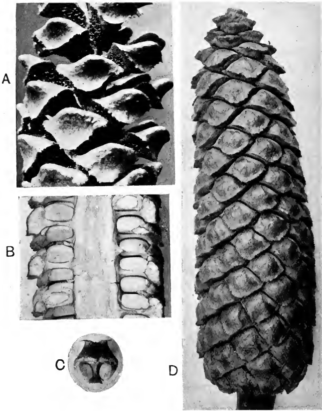
FIG. 393. A. Stangeria paradoxa , part of microstrobilus. B, D. Encephalartos villosus , megastrobilus in surface-view and in section. ( \frac{1}{4} nat. size.) C. Ceratozamia mexicana , single megasporophyll.
