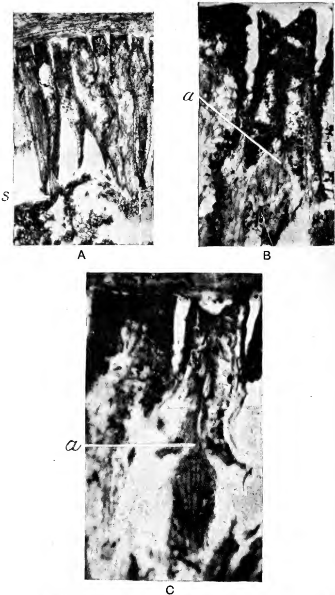
FIG. 563. Williamsonia scotica . Megasporophylls and interseminal scales in longitudinal section. A, part of the axis showing the attachment, s , of a scale and megasporophyll. B, apex of micropylar tube showing funnel-shaped cavity and papillose epidermal cells on the integument and on the adjacent scale; a , apex of nucellus. C, upper part of a scale and megasporophyll; a , apex of nucellus. (A, ca. \times 20 ; B, C, \times 100 .)
