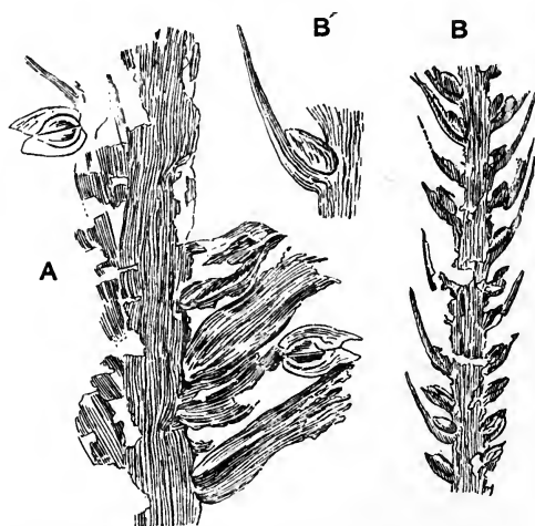
FIG. 480. A, Cordaianthus Pitcairniae with Samaropsis seeds. B, Cordaianthus Volkmani . B', portion of B enlarged. (A, B, nat. size; Kidston Coll. 2374, 1174.)
