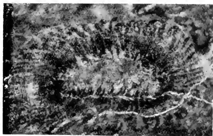
FIG. 511. Cycadeoidea Gibsoniana . Stele in the cortex. (British Museum, 8406.)
