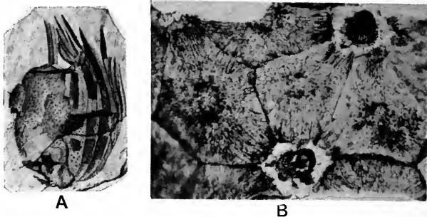
FIG. 568. Wielandiella angustifolia . A, conical receptacle with bracts. B, surface-view of scales and micropylar tubes. (After Nathorst; A, \frac{2}{3} nat. size.)
