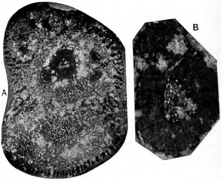
FIG. 455. Calamopitys Saturni . A, stem with leaf-bases; \times 5 . B, stele showing leaf-trace after emerging from the secondary xylem; \times 16 . (After Zalessky.)
