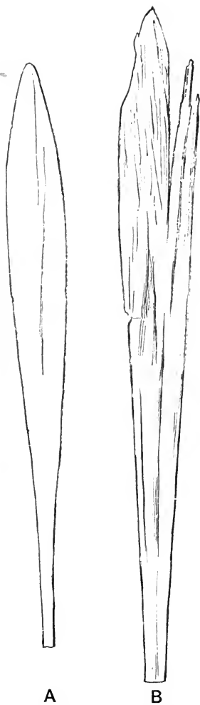
FIG. 471. Cordaites (Noeggerathiopsis) Hislopi . From Vereeniging. (A, ca. \frac{1}{3} nat. size; B, ca. \frac{1}{8} nat. size.)
