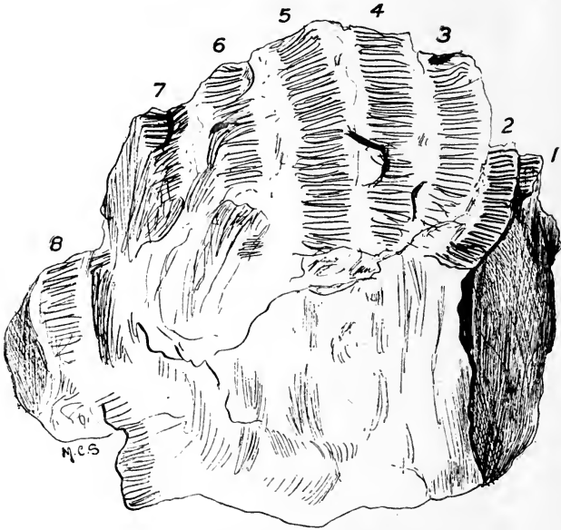
FIG. 578. Bucklandia buzzardensis . Rough sketch of a block of wood showing parts of at least eight concentrically arranged rings of secondary wood. (After Stopes; \times \frac{3}{2} .)
