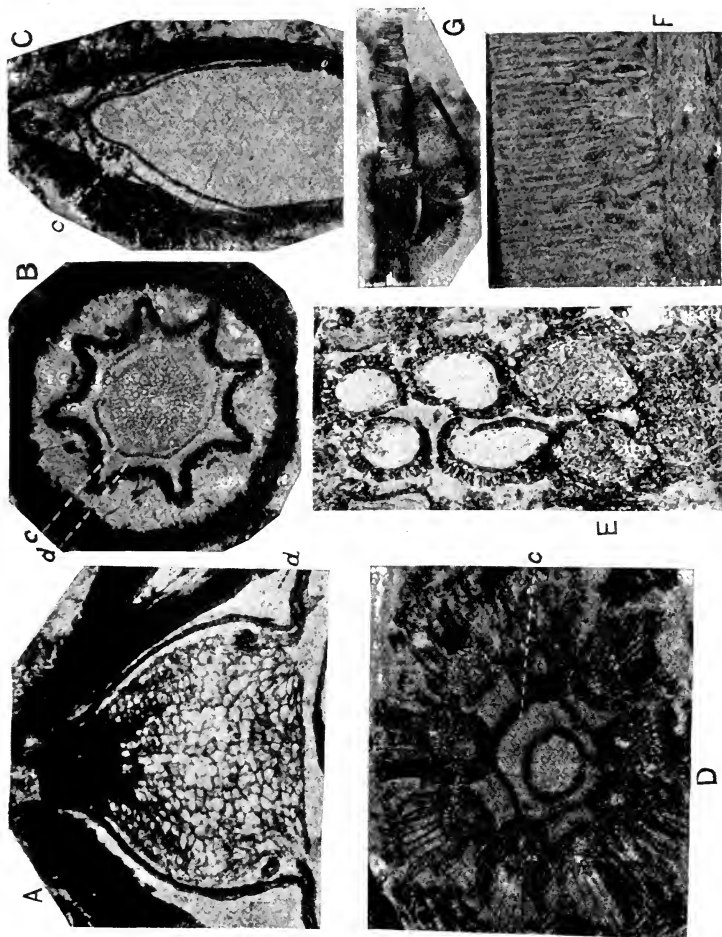
FIG. 493. A, Lagenostoma ovooides , longitudinal section of the lagenostome. B, Lagenostoma Lomari , transverse section of the lagenostome and canopy; c, pollen-chamber; d, space between the nucellus and integument. (A, after Miss Prankerd; B, from a section in the Manchester Museum, R 1048.) C, Physostoma elegans , longitudinal section showing microspores in the pollen-chamber, c. (From a section in the University College Collection.) D, Physostoma elegans , transverse section of the apical region showing the tentacles, pollen-chamber, c, etc. E, Telan-gium Scotti , transverse section of sporangia (Manchester Coll. R 1047). F, G, Stephanospermum akenioides . F, section of sclerotesta. G, tra- cheids from the nucellus. (Uni- versity College Coll.)
