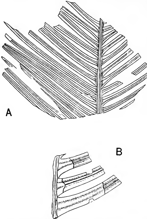
FIG. 617. Pseudocycas insignis . From the Lias of Hör. A, \frac{5}{8} nat. size; B, ca. \times 2 . (After Nathorst.)
