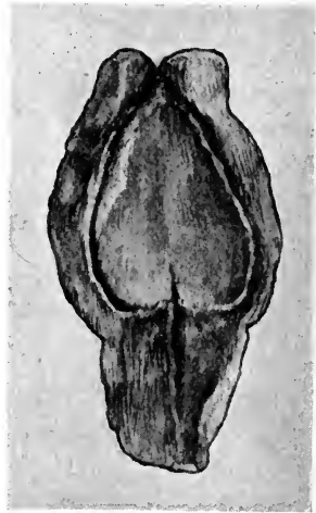
FIG. 503. Samaropsis Lesliei . From Vereeniging, S. Africa. (Mr Leslie's Collection; nat. size.)
