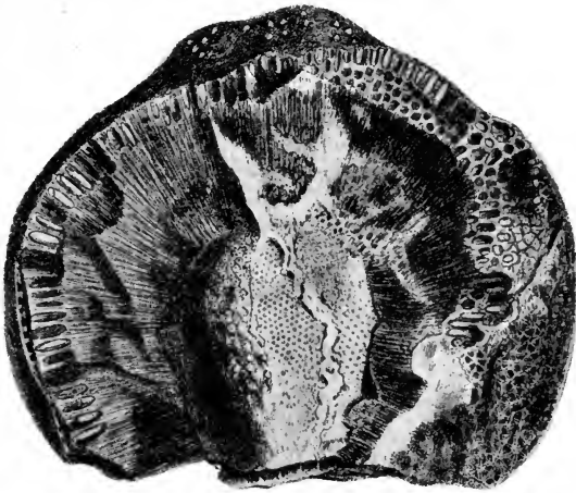
FIG. 560. Williamsonia Bucklandi . (After Buckland; \frac{5}{8} nat. size.)
