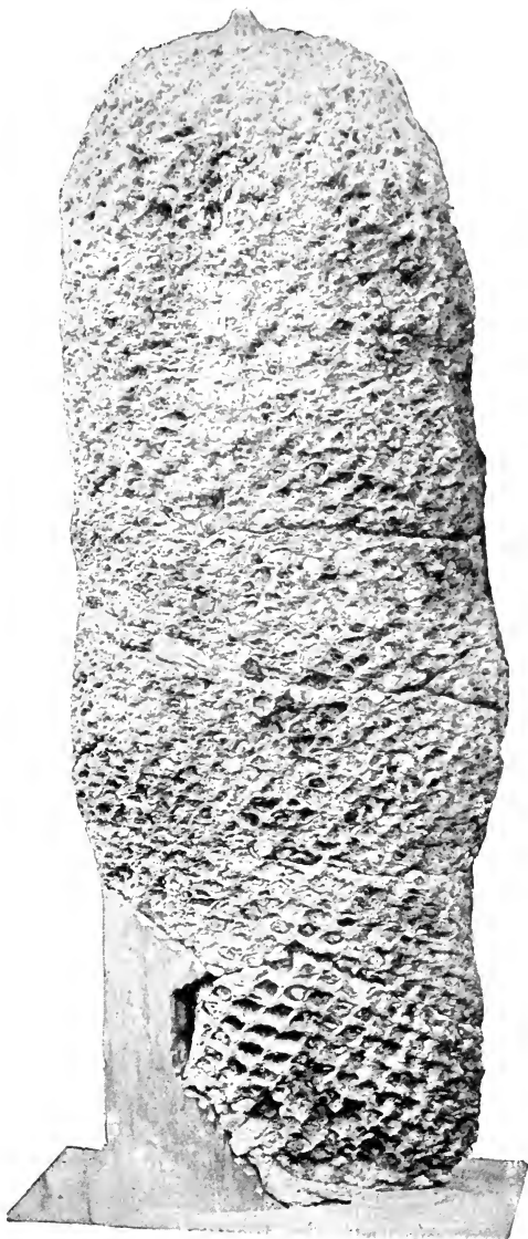
FIG. 536. Cycadeoidea gigantea . (The original is in the British Museum; 1/3 nat. size.)
