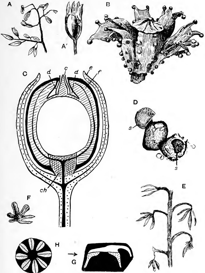
FIG. 408. A, A', Lagenospermum Sinclairi . B, Lagenostoma , restoration. C, Lagenostoma Lomaxi ; c , micropyle; d , space between integument and nucellus; e , cupule; f , integument; ch , chalaza. D, microspores of Lagenostoma ovoides . E, F, Calymmatotheca Stangeri . G, H, Crossotheca Hoeninghausi . H, section of G in line of arrow. (A, after Arber; B, C, E, F, after Oliver; D, after Benson; G, H, after Kidston.)
