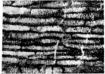
FIG. 520. Cycadeoidea Gibsoniana . Ground-tissue of bract. (British Museum, 41388.)
