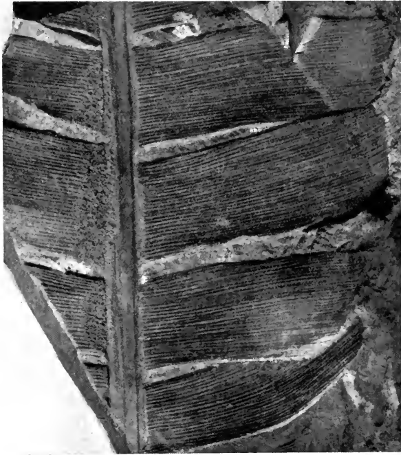
FIG. 623. Nilssonia princeps . (Slightly reduced; Indian Geological Survey, Calcutta.)
