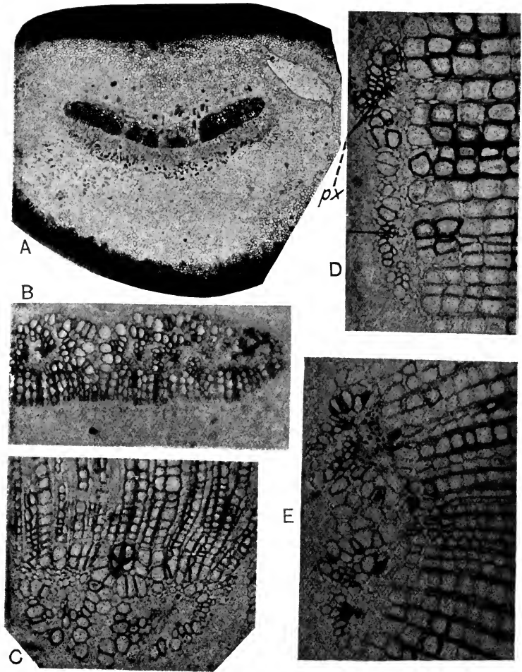
FIG. 464. Poroxylon . A, B, Poroxylon Boysseti . A, transverse section of leaf in the region of lateral expansion of the petiole; B, portion of vascular tissue of A. C—E, Poroxylon Edwardsii . C, leaf-trace showing recent separation of the two protoxylems; D, leaf-trace at a lower level with more widely separated protoxylems, px ; E, leaf-trace intermediate between C and D. (From photographs supplied by Prof. Bertrand.)
