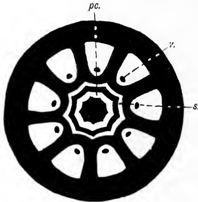
FIG. 409. Lagenostoma . Transverse section near the micropyle, showing the pollen-chamber, pc , the space, s , between the nucellus and integument, the fluted canopy with vascular bundles, v . (After Oliver.)
