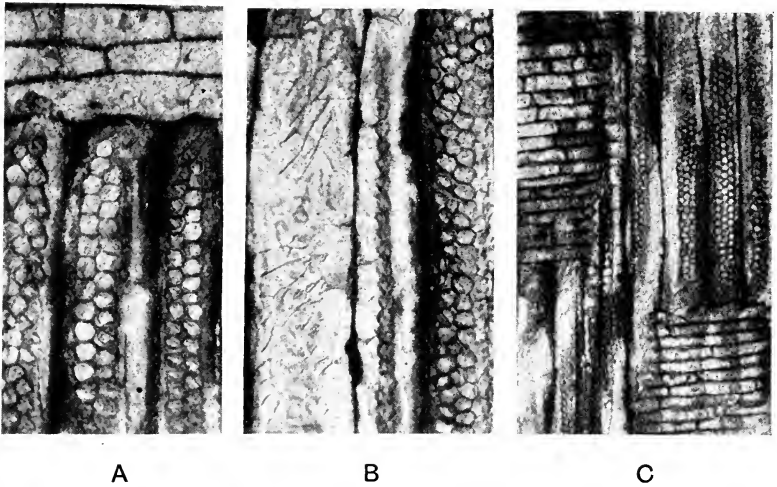
FIG. 475. Dadoxylon materiaram . A—C radial longitudinal sections of the secondary xylem. (Kidston Coll. 225.)
