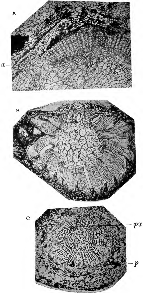
FIG. 415. A, B, Heterangium . A, H. Grievii , a , leaf-traces. B, H. tiliacoides . C, root of Lyginopteris . (A, B, Kidston Coll., 529, 294; C, Williamson Coll., 1631.)
