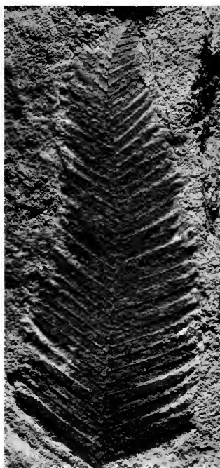
FIG. 595. Ptilophyllum pecten . The specimen figured by Sternberg as Polypodiolites pectiniformis . (Oxford Museum; \frac{2}{3} nat. size.)
