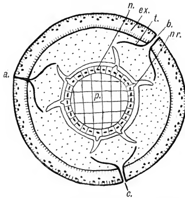
FIG. 497. Pachytesta . Transverse section of a seed showing the exotesta, ex , with sclerous layers and vascular strands (black), the endotesta (dotted), the nucellus with its ring of vascular bundles, n , and the prothallus, p . The three radial plates in the exotesta are seen at a , b , c , with the trabeculae, t , and internal to these are the grooves in the endotesta engaging with ribs on the nucellus, nr . (After Oliver.)
