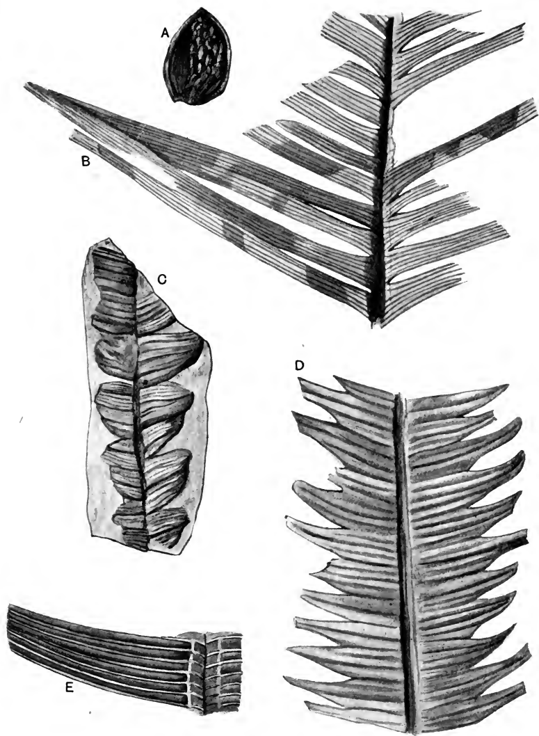
FIG. 619. A, seed ( Nilssonia ?); B, Nilssonia pterophylloides ; C, D, Nilssonia brevis ; E, N. polymorpha . (A—D \frac{3}{8} nat. size; E, slightly enlarged; after Nathorst.)
