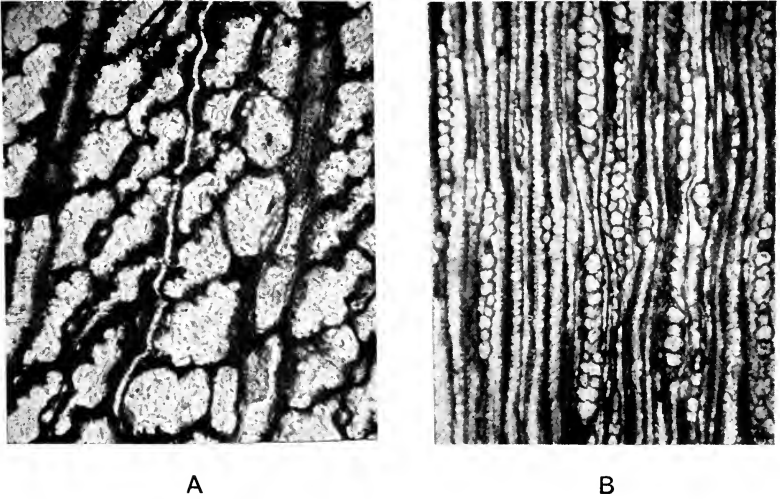
FIG. 474. Dadoxylon materiaram . Transverse (A) and tangential (B) sections of the secondary xylem. (Kidston Coll. 222, 224.)
