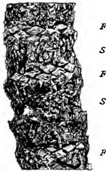
FIG. 380. Cycas circinalis . Stem showing alternate zones of leaf-bases (F) and scale-leaf bases (S). (From the Encyclopaedia Britannica .)
