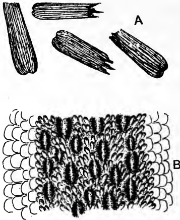
FIG. 485. Titanophyllum Grand'Euryi . A, leaves \frac{1}{3} nat. size; B, stomata on the lower surface of the lamina. (After Renault and Zeiller.)
