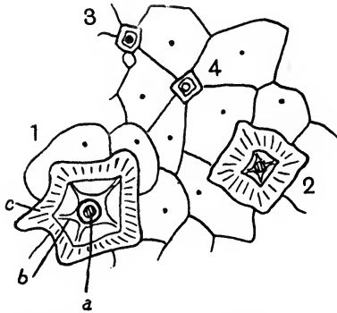
FIG. 527. Cycadeoidea Morierii . Transverse section of interseminal scales and seeds near the apex of the latter; seeds 1 and 2 show the pollen-chamber, a ; the fibrous layer, b , forming wings and extending across the fleshy tissue; c , the radial layer; seeds 3 and 4 are aborted. (After Lignier.)
