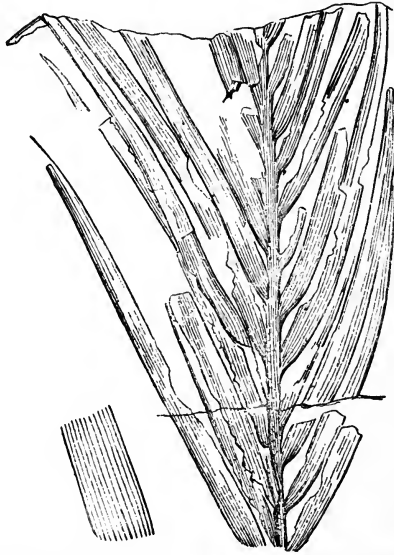
FIG. 627. Pseudoctenis eathiensis . (British Museum, No. V. 2744; \frac{1}{2} nat. size.)
