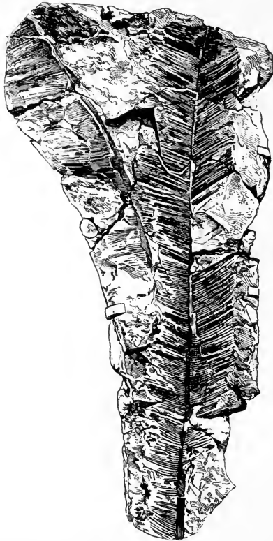
FIG. 618. Pseudocycas Saportae . From the Wealden, near Hastings. (British Museum, V. 2777; \frac{1}{2} nat. size.)
