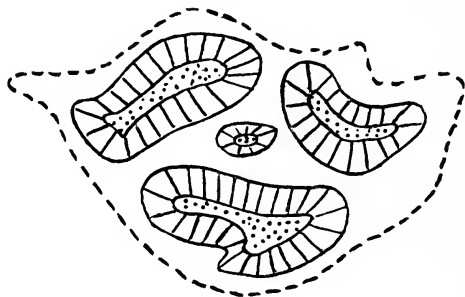
FIG. 417. Medullosa centroflis . Transverse section showing the deep-seated 'periderm' (broken line) surrounding four steles. (After de Fraine.)
