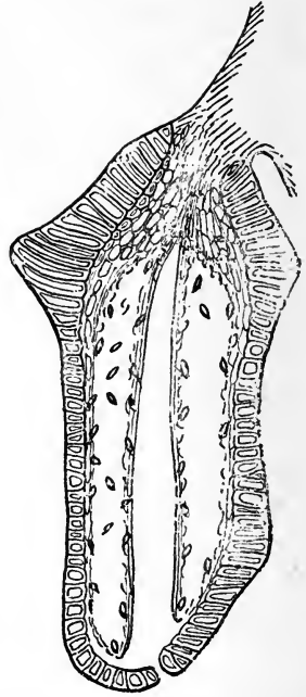
FIG. 532. Cycadeoidea dacotensis . Synangium in longitudinal section showing the thick pedicel, the line of dehiscence, and two loculi with a few microspores. (After Wieland; \times 40 .)
