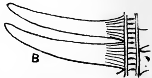
FIG. 613. Pterophyllum Braunianum . (A, nat. size; B, enlarged; after Schenk.)
