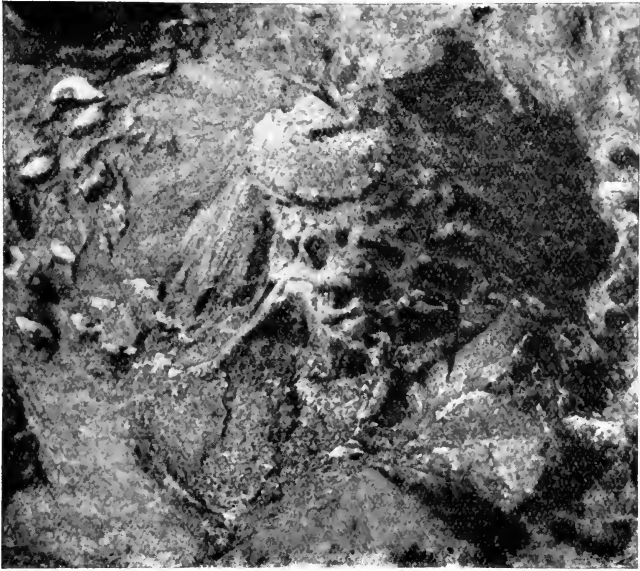
FIG. 534. Cycadeoidea Reichenbachiana . Cup-like cavity on the stem showing the axis and surrounding bracts of a lateral fertile shoot. (After Schuster, from a block kindly supplied by Prof. Rothpletz.)
