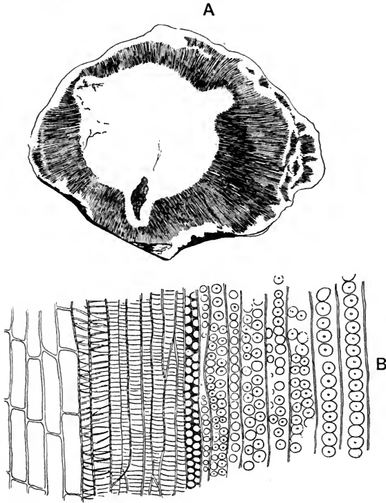
FIG. 476. Dadoxylon Pedroi . A, transverse section showing the pith and part of the secondary wood. B, longitudinal section of part of the secondary wood. (After Zeiller.)
