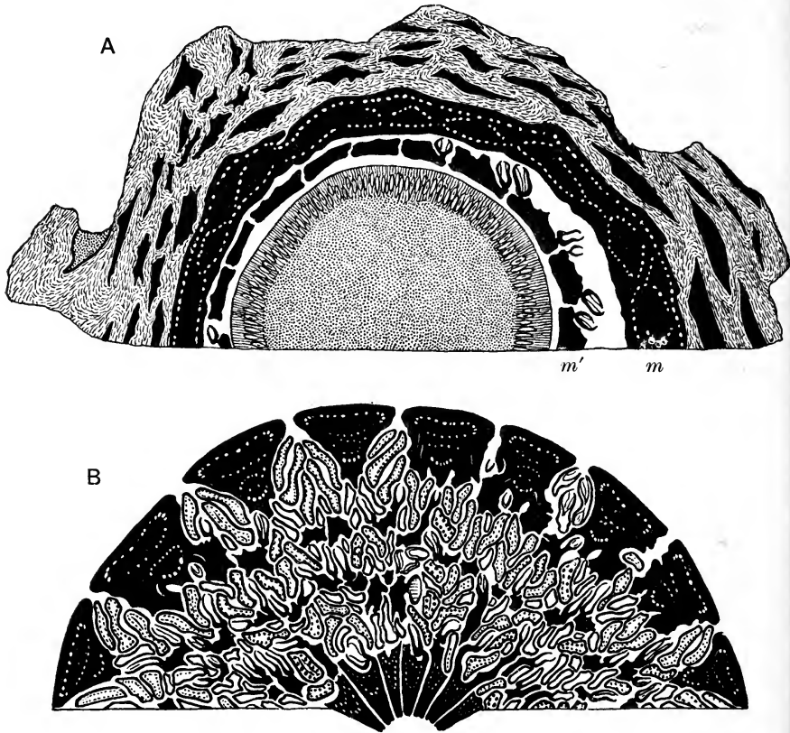
FIG. 530. Cycadeoidea dacotensis . Transverse sections through a bisporangiate strobilus. A, showing the receptacle with its interseminal scales and ovules, the continuous disc of microsporophylls, m , with vascular bundles, and the separate ( m' ) infolded portions of the microsporophylls with some synangia; bracts and rammenta. B, this section, cut above the apex of the receptacle, shows the microsporophylls and synangia. (After Wieland.)
