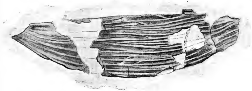
FIG. 624. Ctenis sp. Single pinna. (Manchester Museum, No. 53.)
