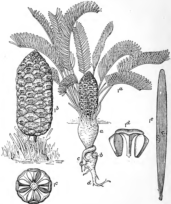
FIG. 395. Zamia floridana . 1 a, complete plant; a, main trunk; b, branch-scar; c, secondary root; d, primary tap-root. ( \frac{1}{8} nat. size.) 1 b, 1 c, megastrobilus. ( \frac{1}{2} nat. size.) 1 d, megasporophyll. ( \frac{1}{2} nat. size.) 1 e, pinna. ( \frac{2}{3} nat. size. After Wieland.)
