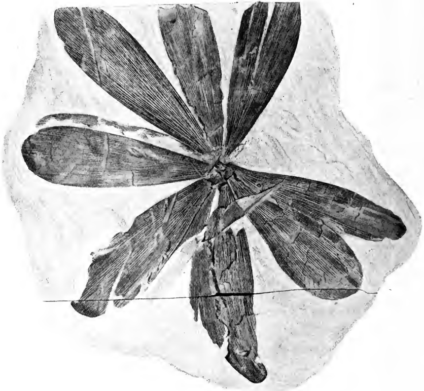
FIG. 472. Cordaites ( Noeggerathiopsis ) Hislopi . From India. (Calcutta Museum; \frac{2}{3} nat. size.)
