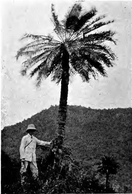
FIG. 377. Cycas circinalis . From a photograph taken by Mr A. Malins Smith at Teldeniya (Ceylon).
