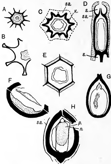
FIG. 495. A, Polyptospermum Renaultii . B, Ptychotesta tenuis . C, D, Polylophospermum stephanense ; sa, sarcotesta; s, spaces; v, vascular bundles. E, Hexapterospermum stenopterum . F, Diplotesta avellana . G, Taxospermum Grüneri . H, Diplotesta Grand'Euryana . (After Brongniart; C, after Oliver.)
