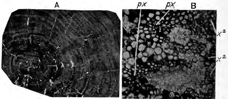
FIG. 490. Mesopitys Tchihatcheffi . A, transverse section showing rings of growth in the wood. B, primary xylem with protoxylem, px , and the edge of the secondary xylem, x^2 . (Kidston collection, 2156.)
