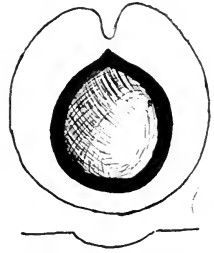
FIG. 499. Samaropsis emarginata , from the Westphalian series, Yorkshire. (Kidston Coll., 4227; \times 2 .)
