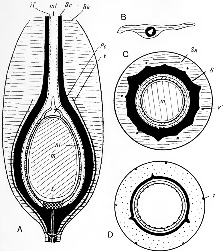
FIG. 426. Trigonocarpus Parkinsoni . A, longitudinal section; Sa, Sc, if, sarcotesta, sclerotesta, inner flesh; mi, micropyle; Pc, pollen-chamber; v, vascular bundles; m, megaspore and prothallus; t, tracheal disc; nt, tracheids in the nucellus. B, transverse section of the upper region showing the sarcotesta, sclerotesta (black) and the micropyle. C, transverse section of T. Parkinsoni . D, transverse section of Trigonocarpus shorensis . (A, C, after Scott; B, after Wild; D, after Salisbury.)
