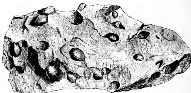
FIG. 423. Casts of the seed-cavity of Trigonocarpus Parkinsoni . (Manchester Museum. \frac{1}{2} nat. size.)
