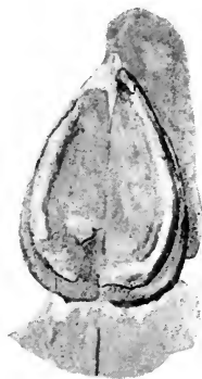
FIG. 504. Samaropsis Milleri . (Indian Geological Survey, Calcutta; nat. size.)
