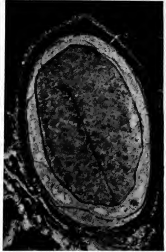
FIG. 523. Cycadeoidea Gibsoniana . Seed with embryo. (British Museum, 41388.)
