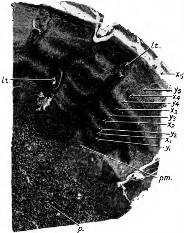
FIG. 580. Colymbetes Edwardsi . Transverse section showing ten alternating zones of wood outside the perimedullary zone, pm ; y_1 , y_2 , etc., vertically running xylem series; x_1 , x_2 , etc., horizontally running xylem series; p , pith; lt , leaf-traces. (After Stopes; \times 2 .)
