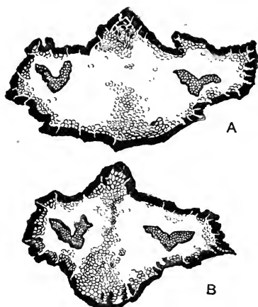
FIG. 406. Lyginopteris oldhamia . Transverse section illustrating branching of petiole. \times 5 . (From a drawing supplied by Prof. Oliver.)
