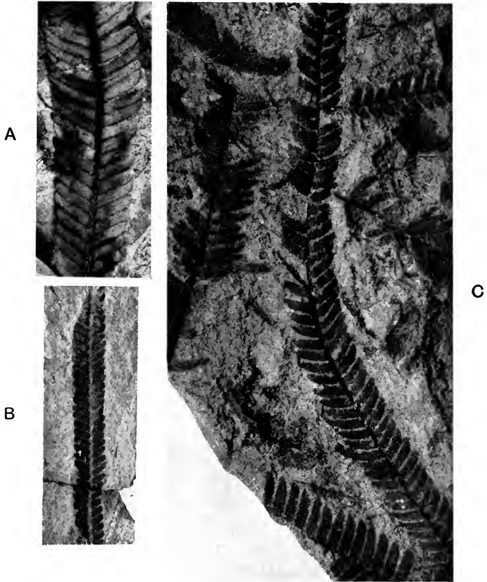
FIG. 588. Ptilophyllum pecten . A, C, specimens figured by Feistmantel as Ptilophyllum cutchense . B, Feistmantel's Otozamites angustatus . ( \frac{1}{5} nat. size; Calcutta Museum.)
