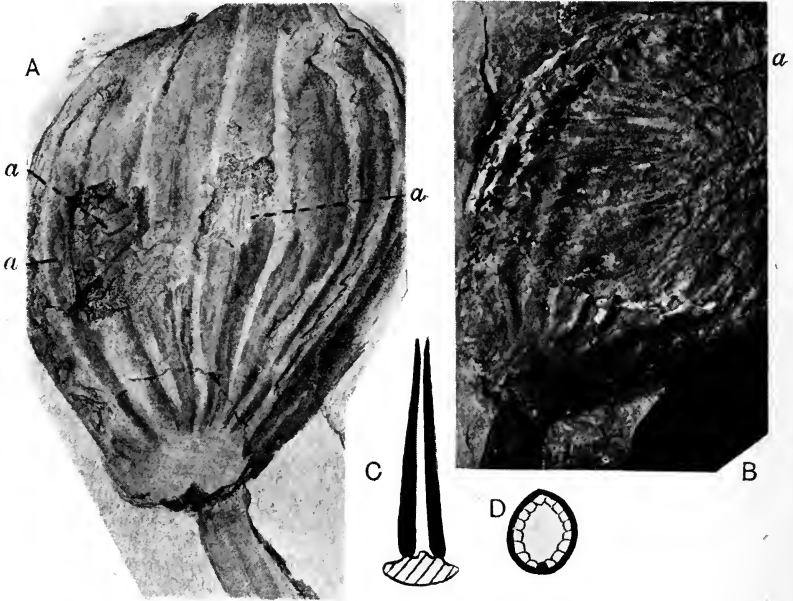
FIG. 574. Cycadocephalus Sewardi . A, surface-view; a, appendages. B, the same specimen, after the removal of some of the microsporophylls, showing the appendages. C, section of a microsporophyll showing the attachment of appendages. D, section of an appendage. (After Nathorst. A, B, \frac{3}{4} nat. size.)
