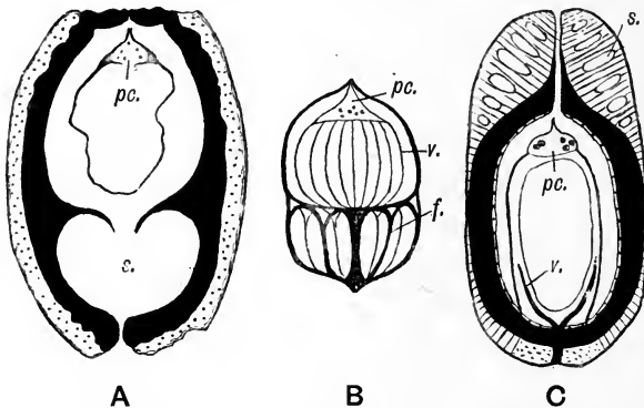
FIG. 498. A, B, Codonospermum . A, C. olivaeforme , longitudinal section showing the seed-proper and the air-chamber, s ; pc , pollen-chamber. B, Diagrammatic sketch of a Codonospermum showing the vascular supply, v , and the fibrous arcs, f , in the wall of the lower part of the seed. C, Aetheotesta elliptica , s , sarcotesta with lacunae; v , vascular supply. (After Renault.)
