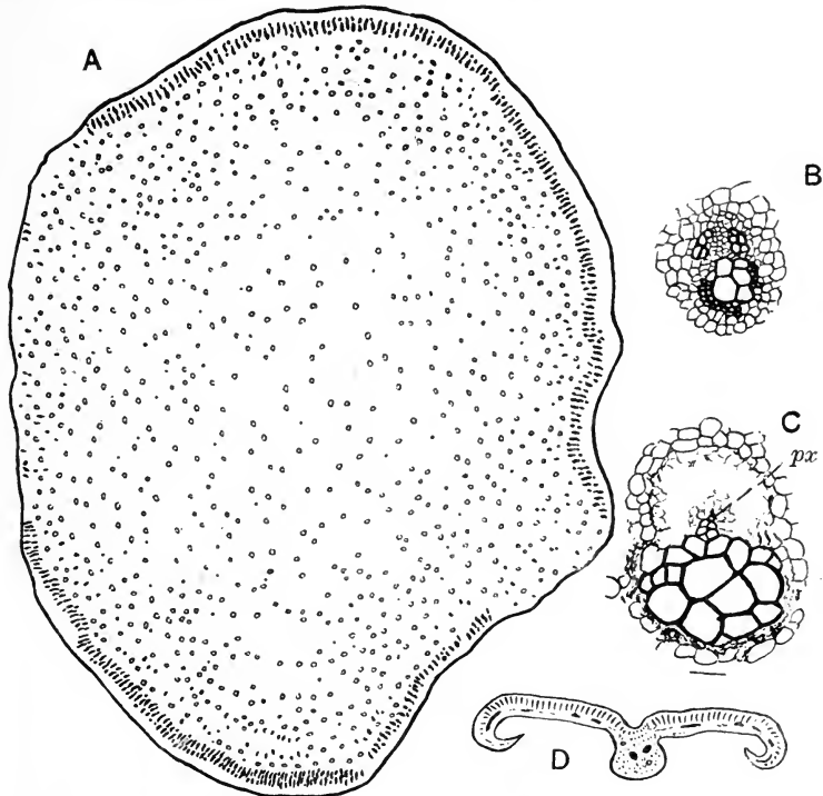
FIG. 420. A, B, Myeloxylon radiatum ; A, petiole \frac{2}{3} nat. size; B, vascular bundle. C, Myeloxylon sp. vascular bundle; px, protoxylem. D, Medullosa anglica ; section of pinnule. (A, B, after Zeiller; D, after Scott.)
