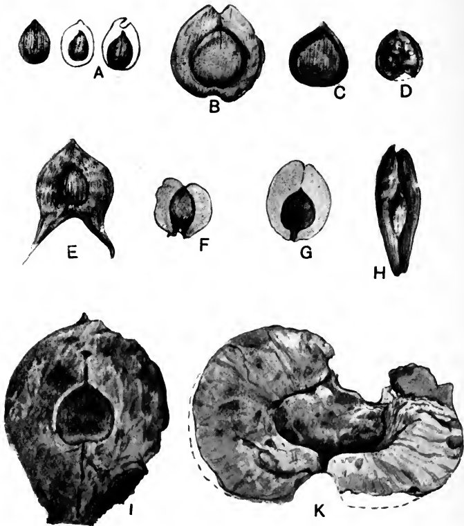
FIG. 502. A, Samaropsis fluitans . B, Samaropsis emarginata . C, D, Cordaicarpus Cordai . E, Samaropsis bicaudata . F, Samaropsis Seixasi . G, Samaropsis barcellosa . H, Samaropsis moravica . I, Samaropsis bignonioides . K, Samaropsis Newberryi . (A, after Dawson; B, R. K. 1576; C, R. K. 1899; D, R. K. 4647; E, after Kidston; F, G, after White; H, after Zeiller; I, after Fiedler; K, R. K. 2313. All nat. size.)
