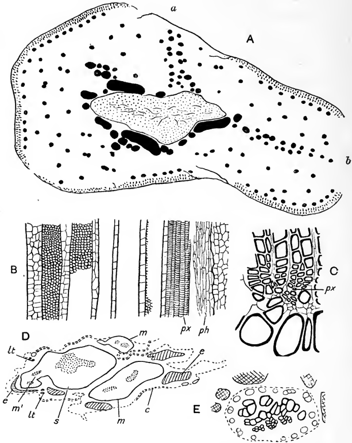
FIG. 439. Sutcliffia insignis Scott. A, B, E, forma a . (After Scott.) C, D, forma β . (After de Fraine.)
