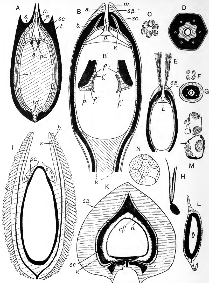
FIG. 494. A, Stephanospermum akenioides ; s , space between integument and nucellus; n , nucellus; e , inner part of testa; sc , sclerotesta; t , t , tracheidal mantle; pc , pollen-chamber; a , archegonia; td , tracheidal pad. B—D, Conostoma oblongum ; a , level of the transverse section shown in fig. C; b , level of transverse section D; m , lobes of tissue surrounding the micropyle; sa , sarcotesta; v , vascular bundles; p , plinth. B', section of lagenostome and part of the integument; f , f' , flanges; v' , wall of micropyle-funnel. E, F, G, Gnetopsis elliptica ; t , tent-pole. F, section of the plumes. G, section through the lagenostome. H, Gnetopsis from Barnsley, Yorkshire, slightly enlarged. I, Physostoma elegans ; h , hairs. K, L, Mitrospermum compressum ; cf , inner flesh; n , nucellus and megaspore. L, transverse section. M, microspores and (?) male gametes of Physostoma elegans . N, microspore of Physostoma showing part of exine and the internal cells. (A—I, N, M, after Oliver; H, Kidston Coll. No. 1255; K, L, after Mrs Arber.)
