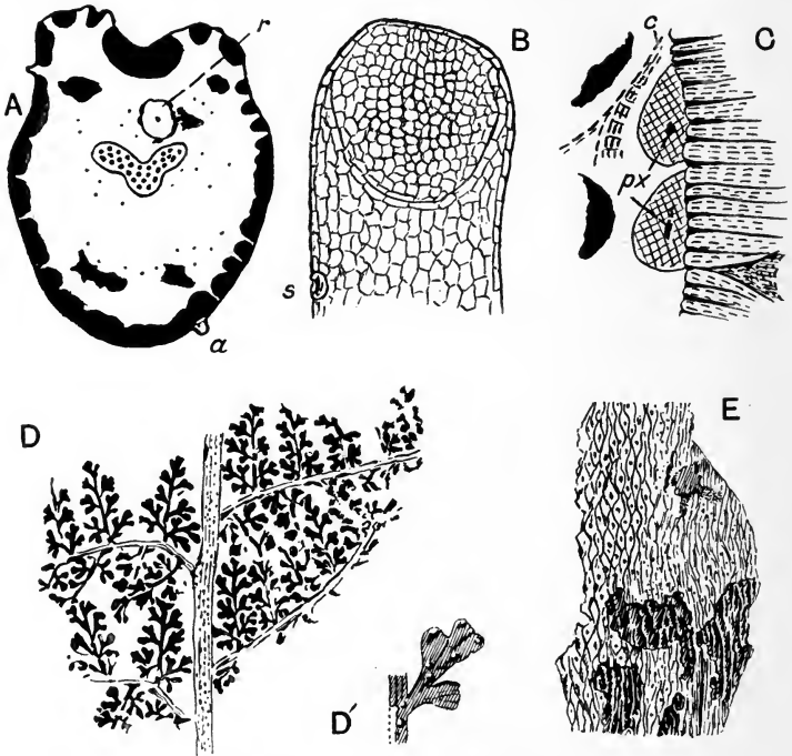
FIG. 405. Lyginopteris oldhamia . A, petiole section; a , glandular emergence; r , root. B, stalked gland; s , stoma. C, inner edge of wood of a stem; c , arc of inversely orientated vascular tissue. D, D', part of a frond of Sphenopteris Hoeninghausi . E, part of axis of D. (A, C, D, Kidston Coll.; B, Manchester Coll. R. 645.)
