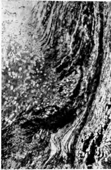
FIG. 522. Cycadeoidea Gibsoniana . Longitudinal section of flower showing half the receptacle with part of the absciss-layer, a . (British Museum.)
