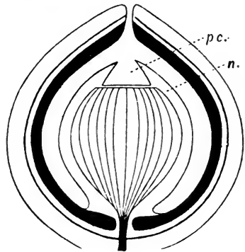
FIG. 492. 'A conjectural synthetic type of seed embodying the characters of such a seed as Stephanospermum with those of a Cardiocarpus '; n , nucellus; pc , pollen-chamber. (After Oliver.)
