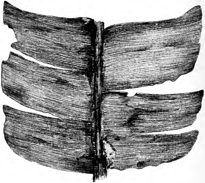
FIG. 622. Nilssonina compta . (Whitby Museum; nat. size.)
