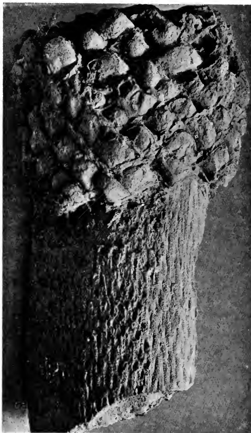
FIG. 577. Bucklandia Yatesii . Type-specimen in the British Museum.
