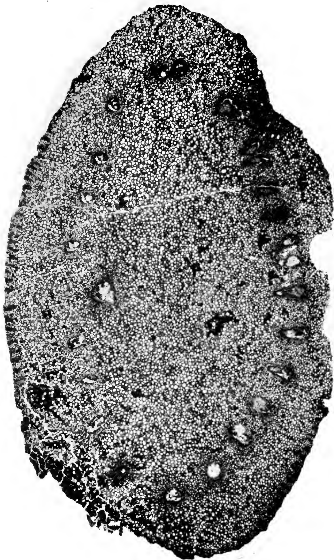
FIG. 456. Kalymma grandis . (From a section in the possession of Prof. Bower; \times 4 .)
