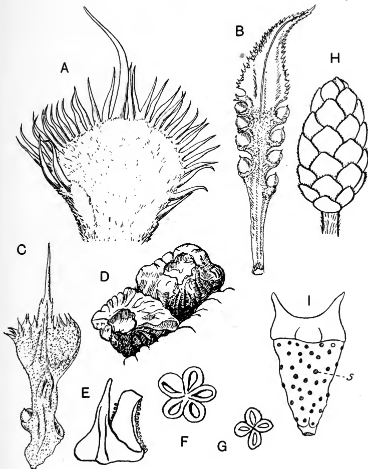
FIG. 392. A. Cycas pectinata , apex of megasporophyll. ( \frac{2}{3} nat. size.) B, C. Cycas Ruminiana , megasporophyll. ( \frac{2}{3} nat. size.) D. Encephalartos Altensteinii . Distal end of megasporophylls. (From the Gardeners' Chronicle .) E, F. Cycas angulata , microsporophyll and sorus. G, I. Ceratozamia mexicana , I, microsporophyll with scars of sori ( s ); G, sorus. (After Thibout.) H. Stangeria paradoxa , megastrobilus.
