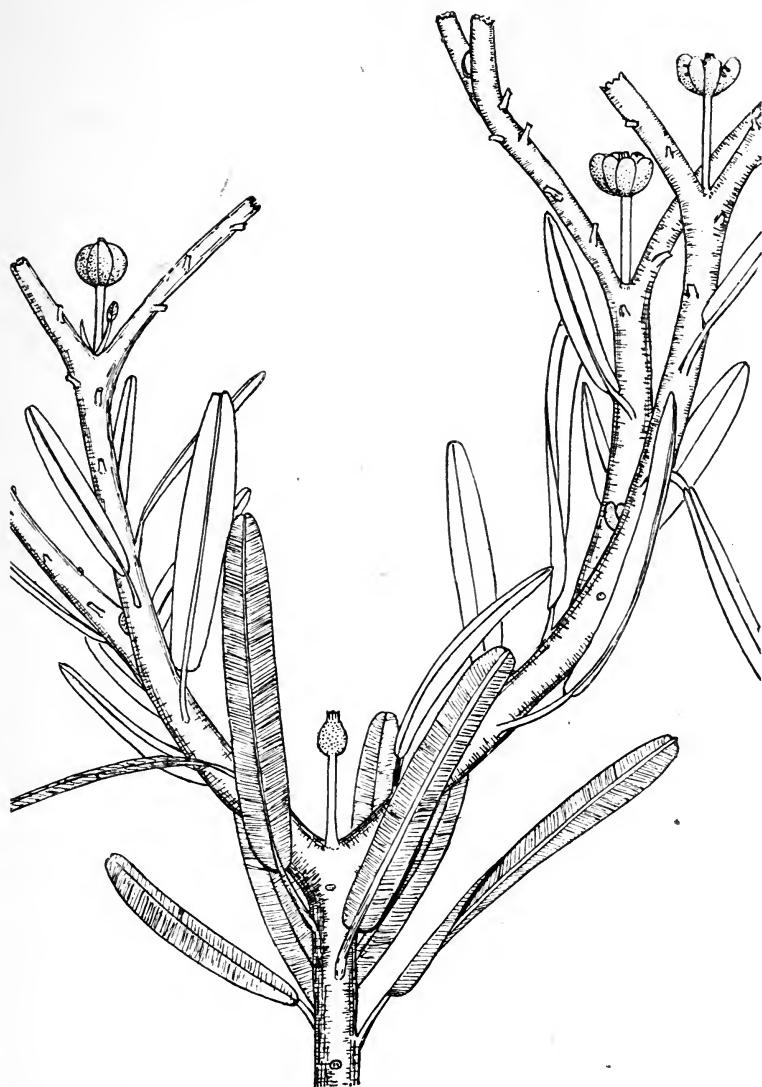
FIG. 573. Williamsoniella coronata . Restoration of part of a plant: the upper leaves are represented only by the petiole-bases. (After Thomas; ca. \frac{3}{8} nat. size.)
