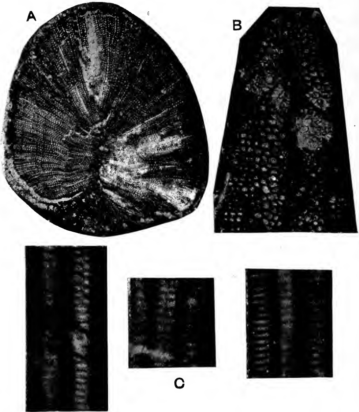
FIG. 460. A, C. A single stele and tracheids of Cladoxylon Kidstoni . (Kidston Coll. 630 B, 630 C.) B. Cladoxylon mirabile , part of a stele. (Museum of Practical Geology, 15872.)
