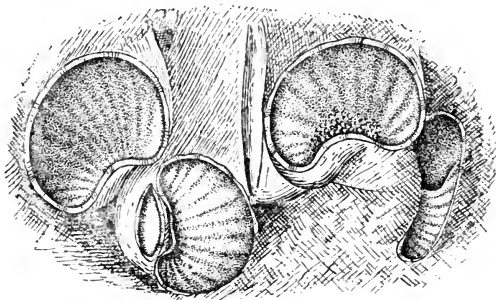
FIG. 531. Cycadeoidea dacotensis . Synangia exposed by weathering and showing the radially disposed loculi. (After Wieland; \times 6 .)
