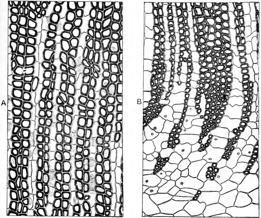
FIG. 508. Cycadeoidea Wielandi . Transverse sections of the secondary xylem of the stem. A, the middle region; B, the inner edge of the xylem. (After Wieland; \times 100 .)
