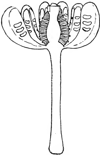
FIG. 569. Williamsoniella coronata . Vertical section of the flower showing the pyriform axis with small megasporophylls and interseminal scales and the microsporophylls with synangia. (After Thomas; \times 2 .)
