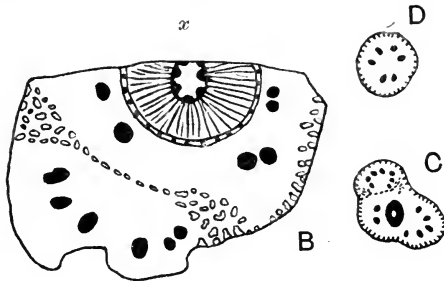
FIG. 454. Calamopitys Saturni . B, stem with leaf-base; x, primary xylem and pith; black patches represent leaf-traces; C, stem with two leaf-bases; D, section of petiole. (After Solms-Laubach.)
