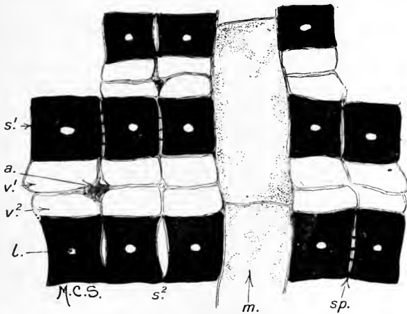
FIG. 540. Vectia lucombensis . Transverse section showing the alternation of fibres, s^1 , s^2 , and radial pairs of pitted elements, v^1 and v^2 ; m , medullary-ray cells; a , parenchyma cell between four thin-walled elements; sp , pits between adjacent fibres; l , much reduced lumen of fibre. (After Stopes.)
