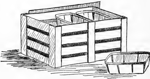
FIG. 26—SIX-BASKET CARRIER
