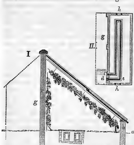
Fig. 92. Plan and section of a vinery, with fire-heat.
