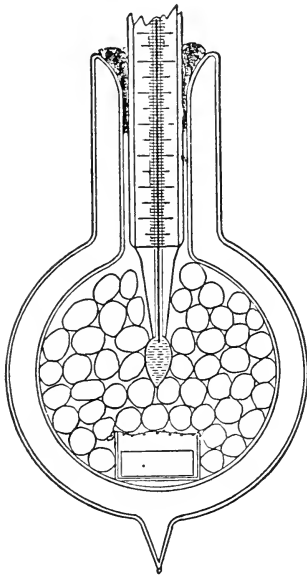
FIG. 69.—A simple calorimeter for studying the temperature transformations in respiration. Respiring seeds are placed in the Dewar bulb (double walled, with a vacuum between the walls). At the bottom of the bulb is a dish containing caustic potash; cotton wool is packed between the thermometer and the neck of the bulb. (After Ganong.)
