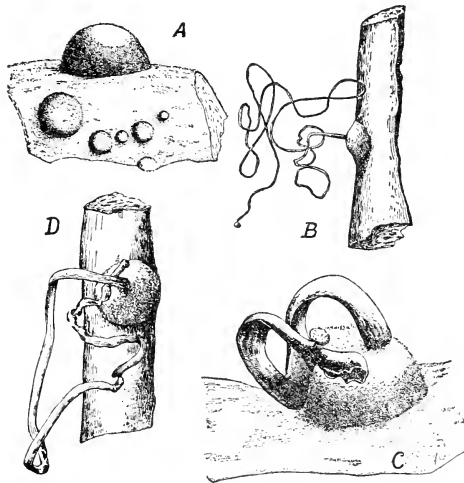
FIG. 219.—Chestnut-blight fungus ( Endothia parasitica ). Fruiting pustules and spore-masses from cultures. \times about 8. A , stages in the development of the pustules; B , C , D , various forms of spore discharge in a moist atmosphere. (After Murrill.)
