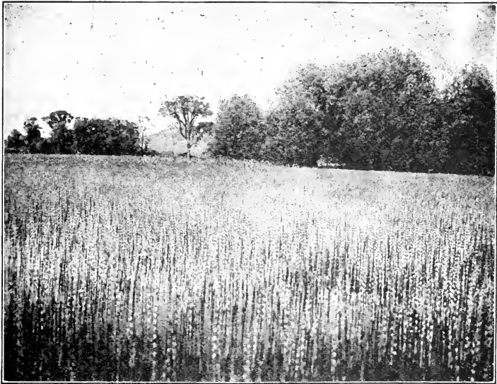
FIG. 266.— Equisetum fluviatile . Pure stand in shallow water, at Tully Lake, N. Y. (Photo by W. L. Bray.)
