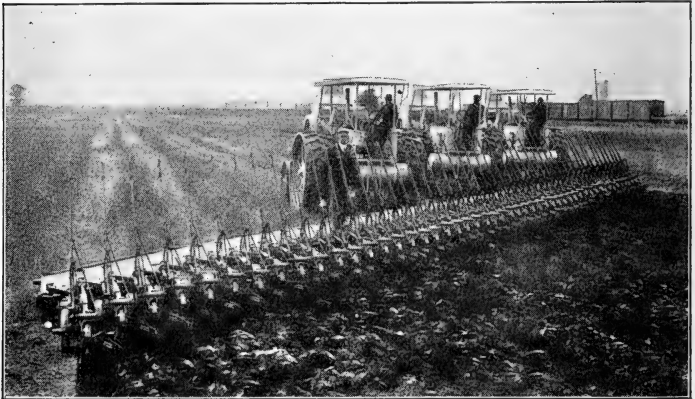
FIG. 5. The "Oil Pull" Gang Plow which, in a demonstration in 1911, with three engines, did the work of 100 men, 200 horses, and 50 plows, plowing 14 acres an hour at a fuel cost of 6\frac{1}{2} cents per acre.
