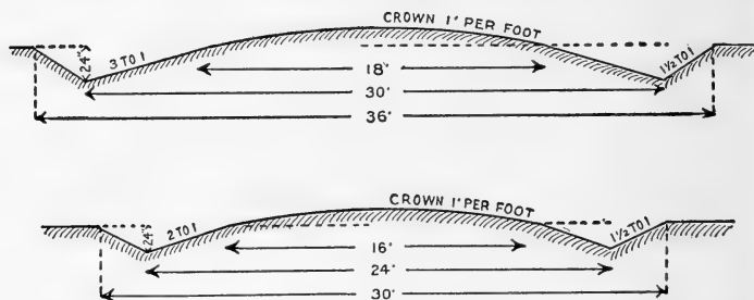
FIG. 239. Standard cross-sections for first and second class earth roads. Iowa Roadway Commission.
