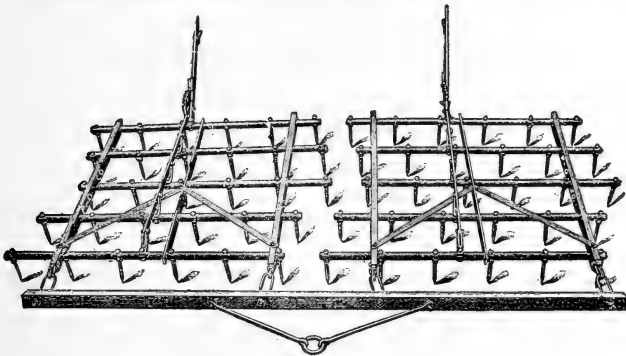
FIG. 80. Spike-tooth harrow.
