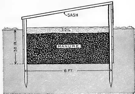
FIG. 124. A hot-bed.
