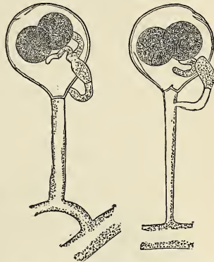
FIG. 97. — Conjugation in Achlya racemosa . (Cornu.)
