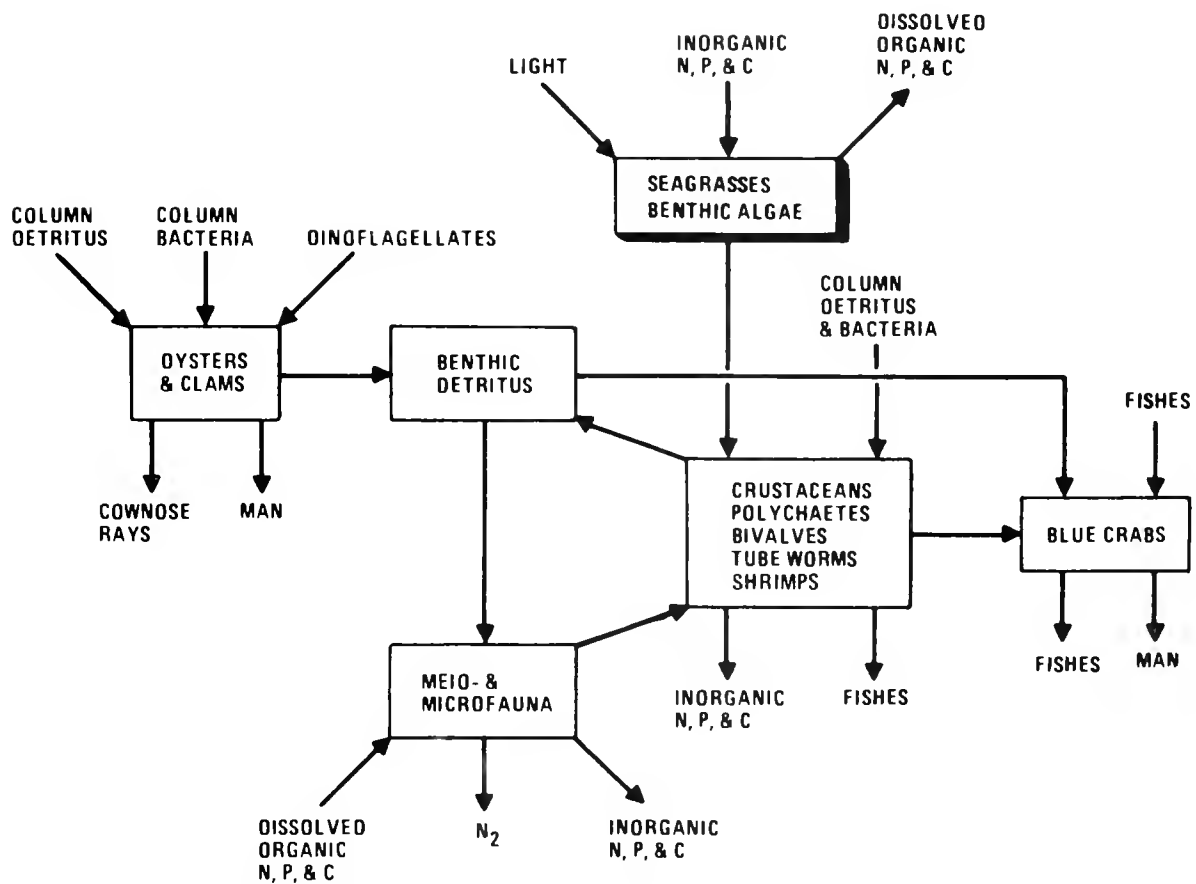
Figure 6. Conceptual model of other benthic communities.
