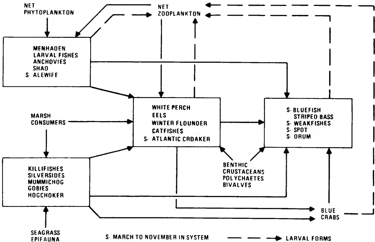
Figure 7. Trophic dynamics of fish.
