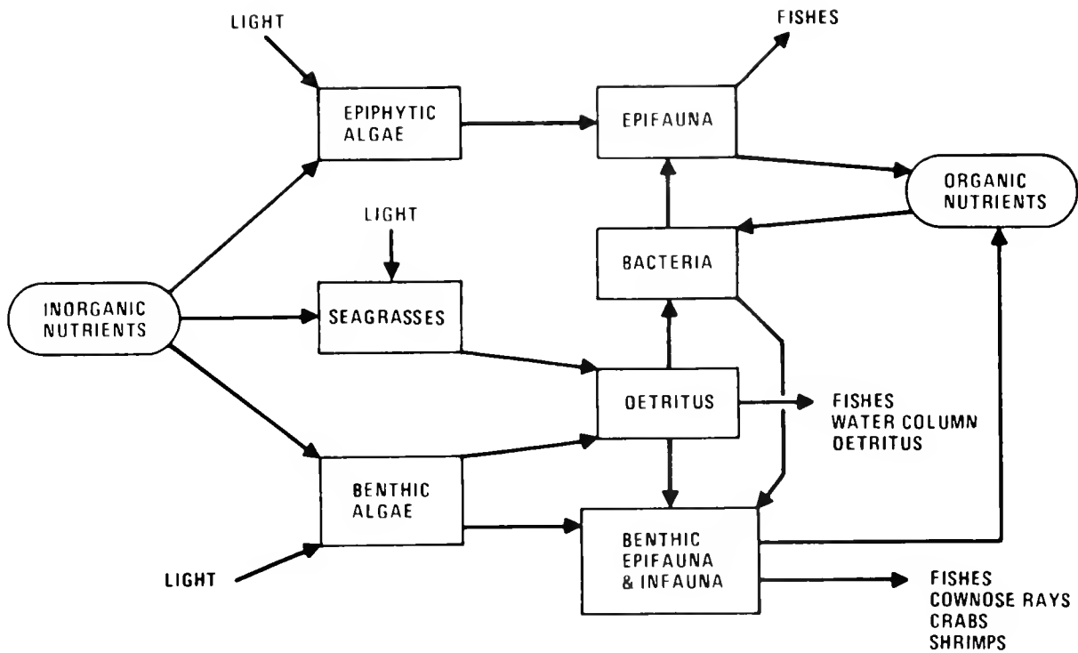
Figure 5. Conceptual model of seagrass communities.
