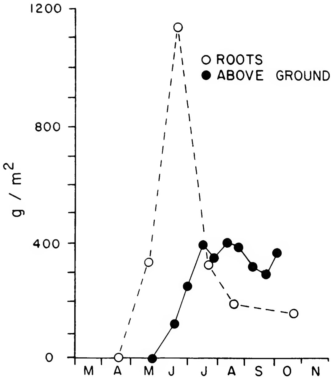
Figure 19. Amounts of aboveground vegetation and roots from April through November on the high marsh at Great Sippewissett Marsh on Cape Cod (Valiela et al. 1976).
