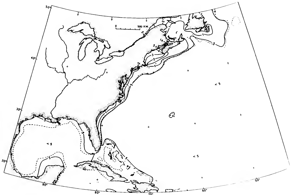
Figure 9. Height of mean spring tides offshore along the Atlantic and Gulf of Mexico coasts of the United States (Emery and Uchupi 1972). Contours are in meters with extra contours for 0.5 and 1.5 m.
