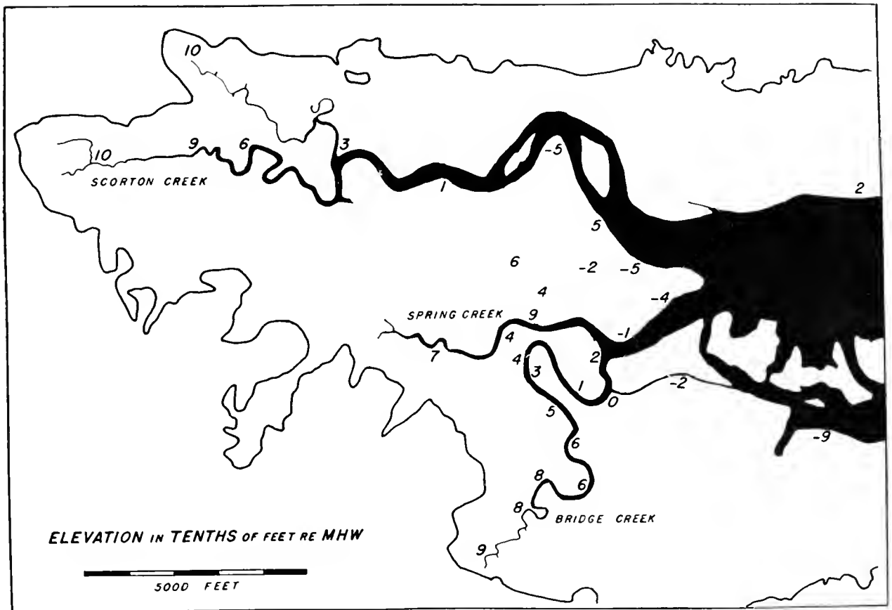
Figure 12. Elevations in tenths of feet of the high marsh surface relative to mean high water (MHW) at Barnstable, Cape Cod (Redfield 1972). Older portions of the marsh are higher.
