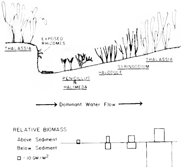
Figure 10. Idealized sequence through a seagrass blowout. Note erosion and recovery zones moving into the dominant water flow.
