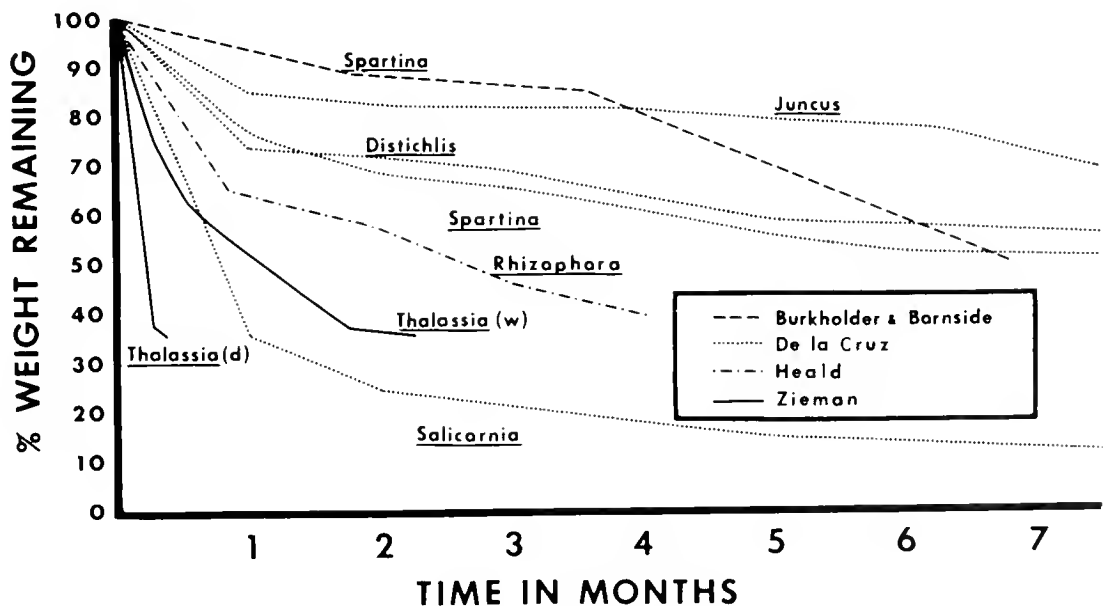
Figure 23. Comparative decay rates showing the rapid decomposition of seagrasses compared with other marine and estuarine plants (references: Burkholder and Barnside 1957; de la Cruz 1965; Heald 1969; Zieman 1975b).
