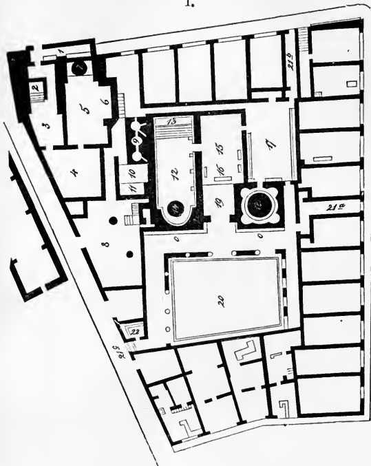
PLAN OF THE BATHS AT POMPEII.
