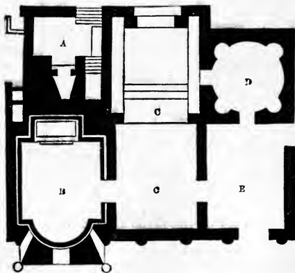
PLAN OF THE BATHS OF STABÆ, AFTER GELL.
