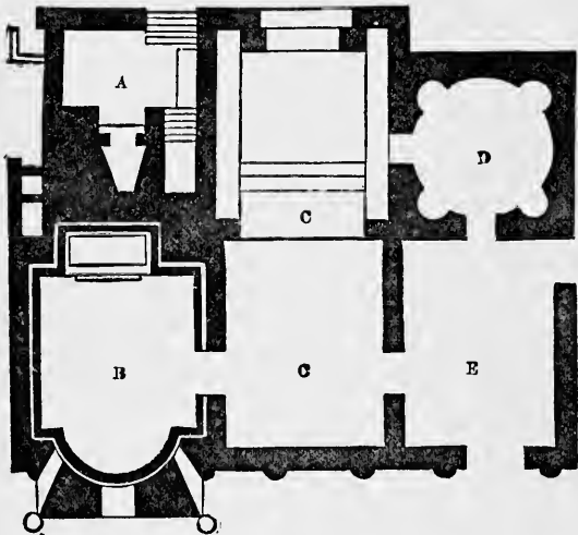
PLAN OF THE BATHS OF STABLE, AFTER GELL.
