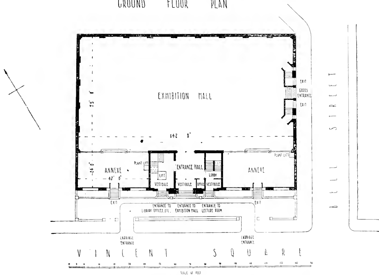
FIG. 128.—GROUND FLOOR PLAN OF NEW HORTICULTURAL HALL. (SEE P. 378.)
