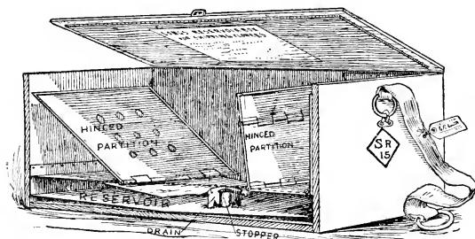
Reservoir Shipping Box showing one side removed and zinc bottom partly broken to show interior arrangement.
