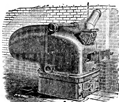
Corrugated Fire-box Boiler.
