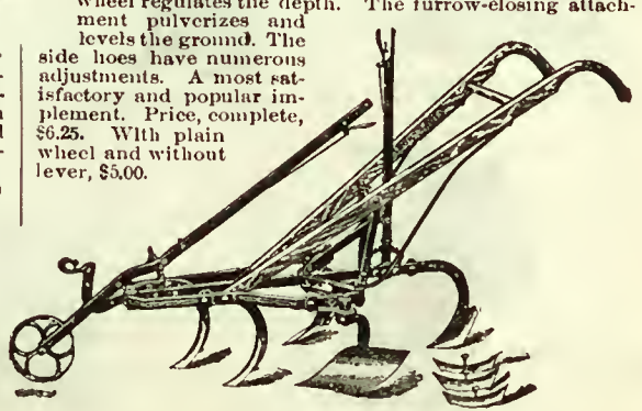
No. 6 “IRON AGE” HORSE HOE AND CULTIVATOR Remarkable for great adjustability. With lever is expanded from 11 in. to 30 in. The wheel regulates the depth. The furrow-closing attachment pulverizes and levels the ground. The side hoes have numerous adjustments. A most satisfactory and popular implement. Price, complete, $6.25. With plain wheel and without lever, $5.00.
