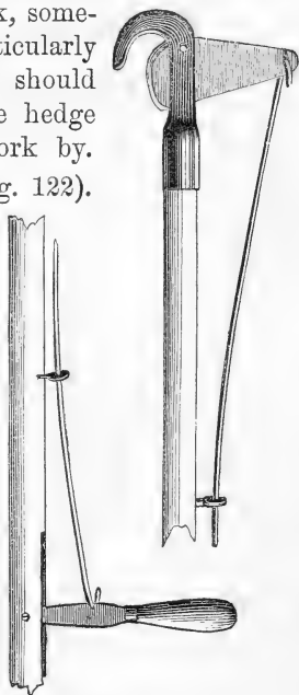
Fig. 123.—TREE PRUNER.
