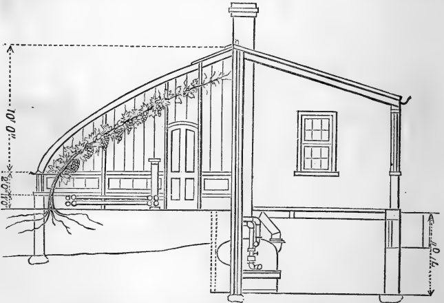
Fig. 63.—SECTION OF FORCING GRAPERY.
