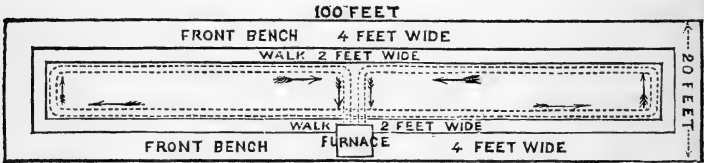
Fig. 42.—PLAN OF GREENHOUSE HEATED BY DOUBLE FLUES.
