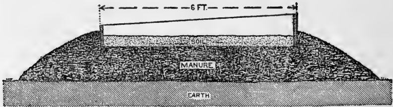
Cross-section diagram of a Hotbed.
