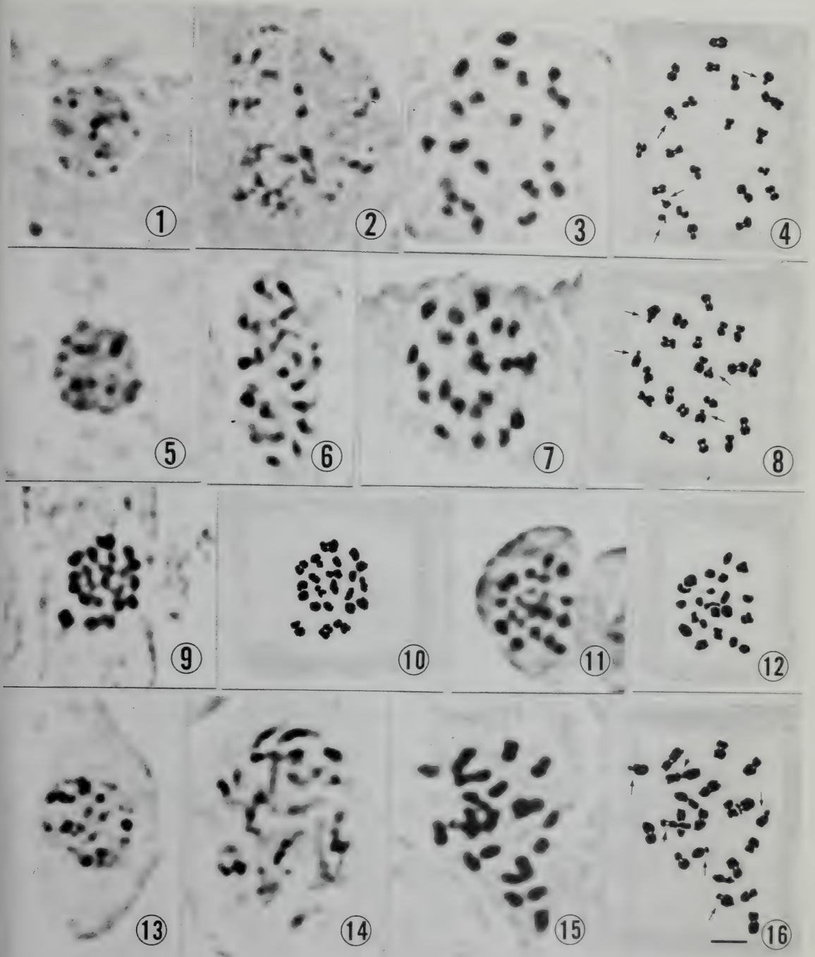
Figs. 1-16. Somatic chromosomes at interphase nucleus (1, 5, 13), prophase (2, 6, 14), and metaphase (3, 4, 7-11, 15, 16) in Myrtaceae. 1-4. Callistemon citrinus ( 2n=22 ). 5-8. Melaleuca cajuputi ( 2n=22 ). 9, 10. M. genistifolia ( 2n=22 ). 11, 12. M. dealbata ( 2n=22 ). 13-16. Syzygium aromaticum ( 2n=22 ). Arrows point out chromosomes with centromeres at subterminal or terminal position. Arrowheads point out chromosomes with secondary constriction. Figures 4, 8, 10, 12 and 16 are drawings of respective preceding photographs. Scale = 2\mu\text{m} .
