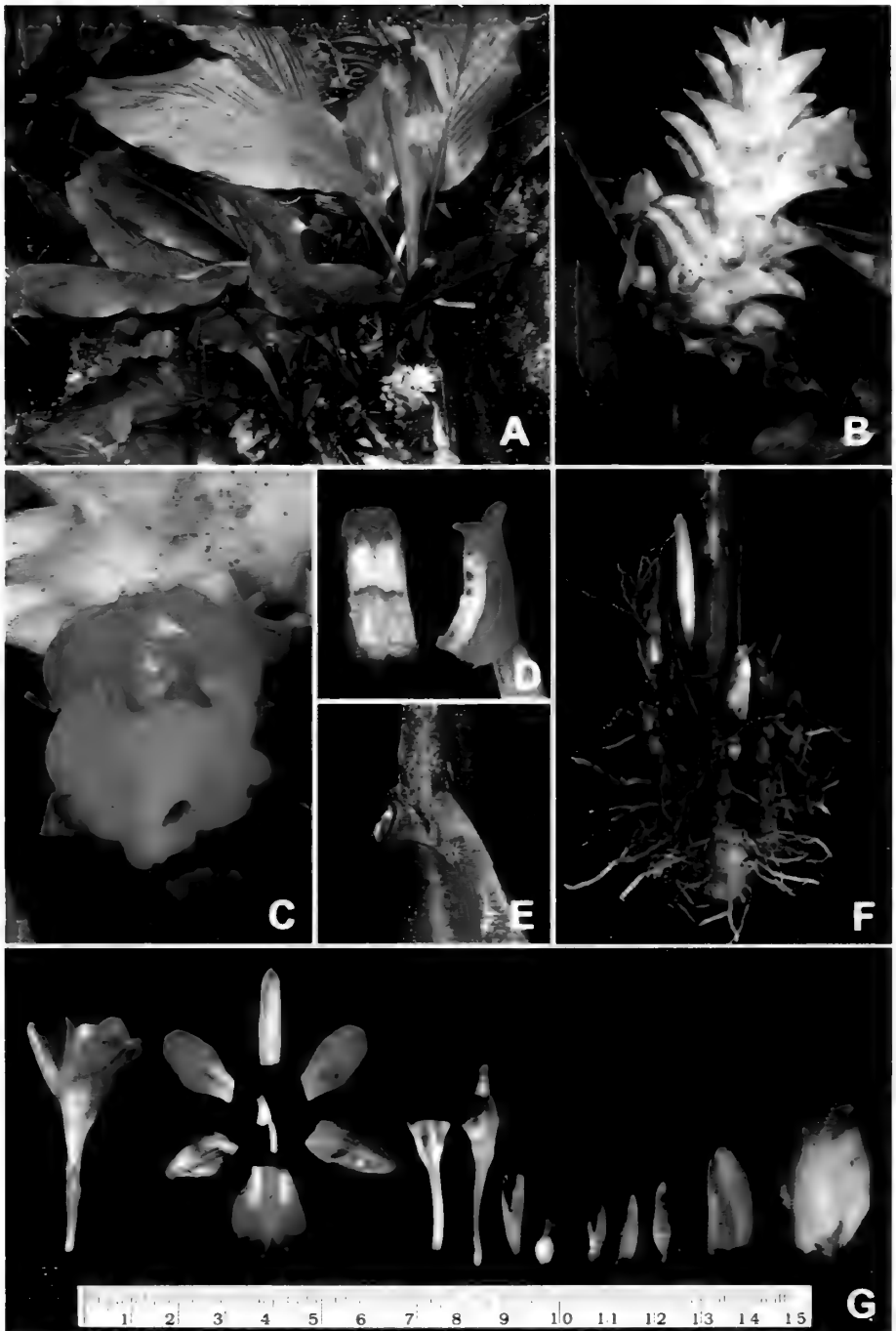
Figure 1. Curcuma vuellina , sp. nov. A. Habit; B. Inflorescence; C. Flower (front view); D. Detail of anther (front and side view); E. Ligule; F. Rhizome and base of leafy shoot; G. Dissected flower. Photographs by J. Leong-Škorničková taken from Tràn et al. 70.
