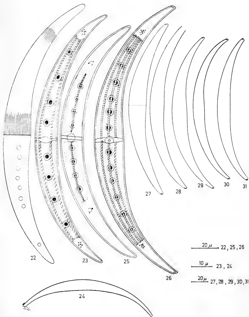
Fig. 22.— Closterium archerianum . Fig. 23.— Closterium parvulum . Fig. 24.— Closterium parvulum var. angustum . Fig. 25.— Closterium calosporum . Figs. 26, 27, 28, 29, 30 y 31.— Closterium dianaе .
