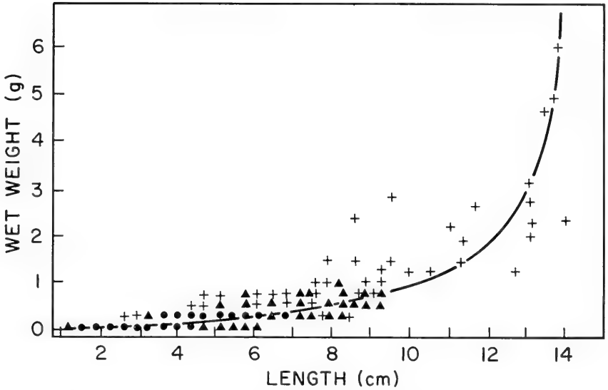
Fig. 11. Relationship between biomass (g wet wt) and length (cm) of fronds (triangles); + = 1 datum point, ▲ = 2-9 points, ● = > 9 points; line drawn by eye.
