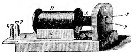
FIG. 10. INDUCTION COIL.
