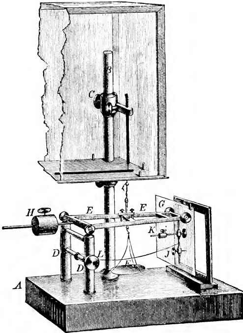
FIG. 8. SIMPLE MYOGRAPH.
