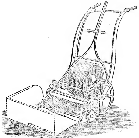
PATENT GRASS-CUTTER.
