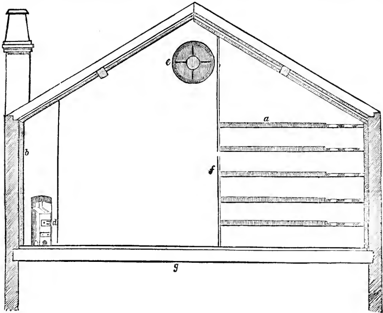
Fig. 3. LONGITUDINAL SECTION.
