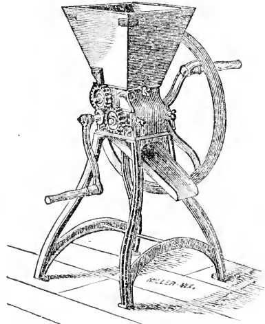
GRAIN CRUSHER. Fig. 5.
