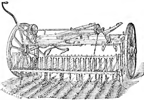
GARRETT'S HORSE-HOE.—END VIEW. Fig. 2.
